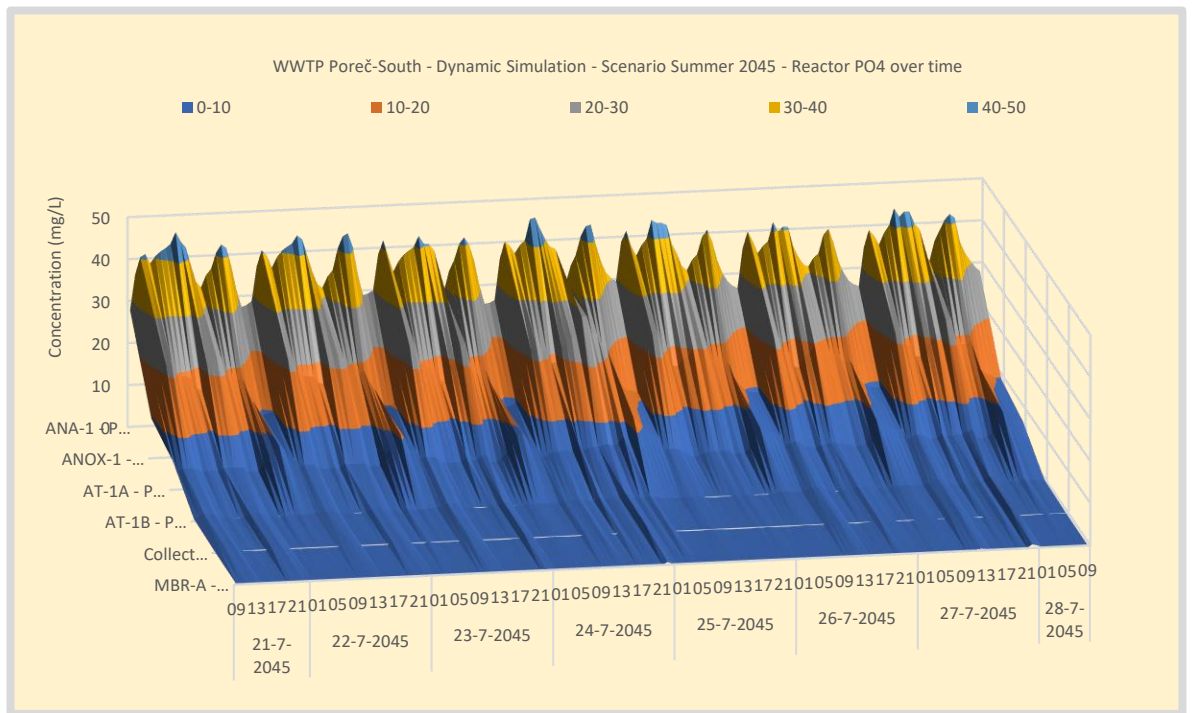
Figure 69. Simulation WWTP Poreč-South - Scenario Summer 2045 - PO4 concentration profile over the waterline.
