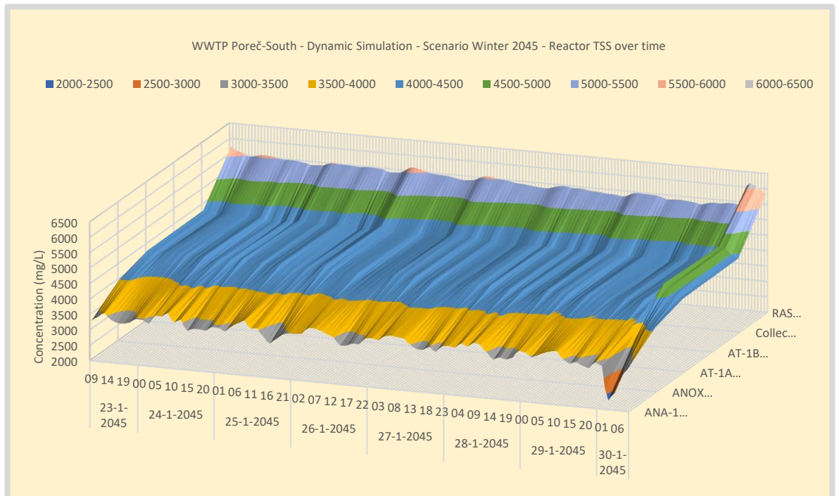
Figure 32. WWTP Poreč-South - Scenario Winter 2045 - TSS concentration profile over the waterline.
