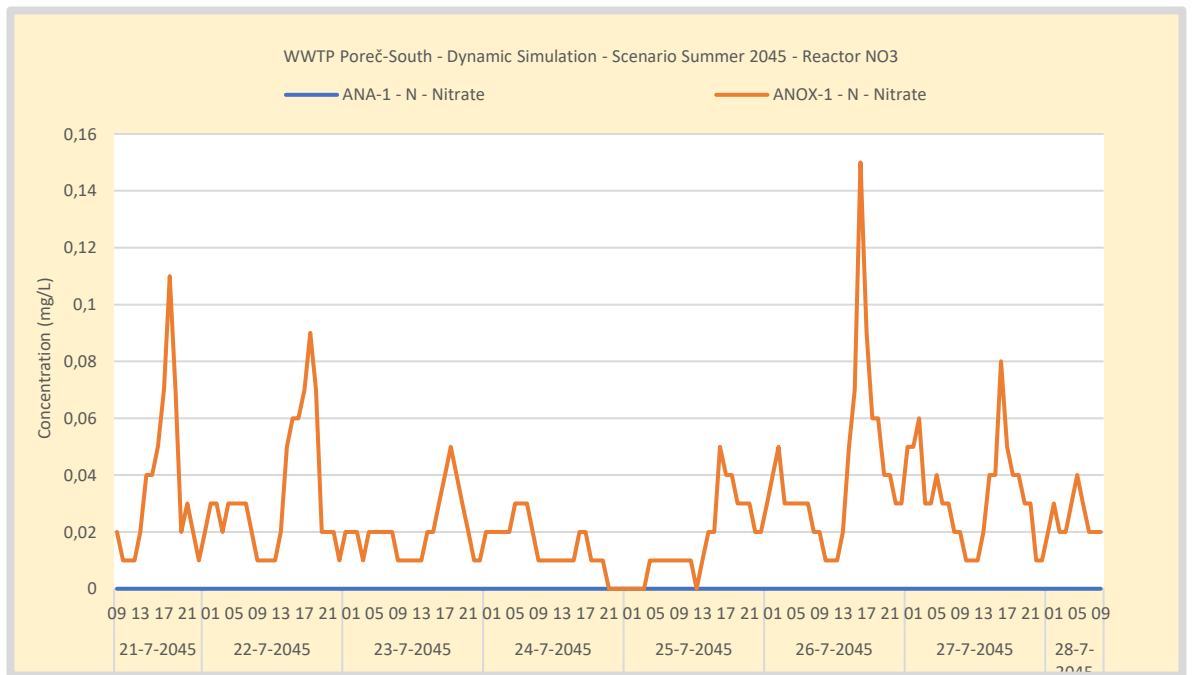
Figure 65. Simulation WWTP Poreč-South - Scenario Summer 2045 - nitrate in the anoxic tank. The anoxic recycle rate is controlled on a nitrate setpoint of 2 mgNO 3 /L in the anoxic tank. Internal recycle capacity is not sufficient to reach this setpoint.
