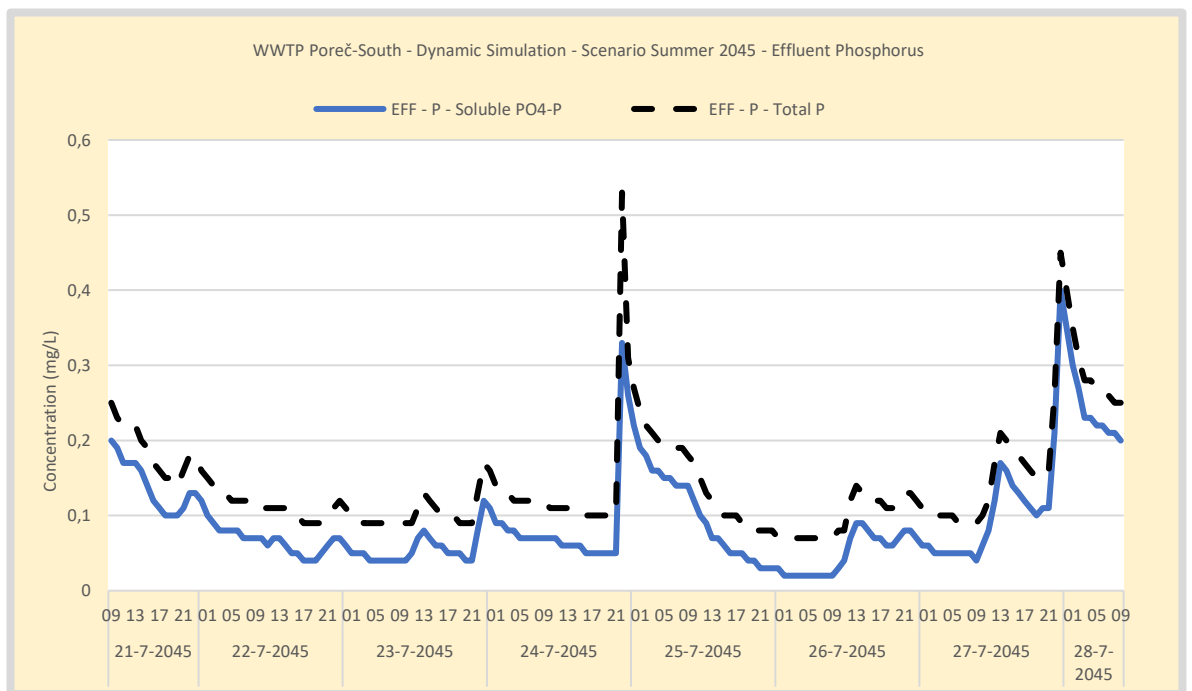
Figure 82. Simulation WWTP Poreč-South - Scenario Summer 2045 - Effluent phosphorus concentration. No Iron is dosed. Effluent is measured in the outflow of the large effluent buffer. The average effluent concentration is below the maximum requirement. At 22 hours on day 4, a bypass event is simulated due to a hydraulic peak loading.
