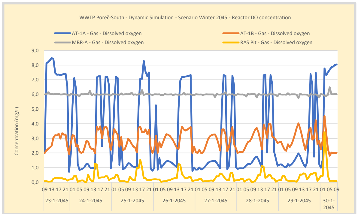
Figure 37. Simulation WWTP Poreč-South - Scenario Winter 2045 - DO concentration gradients. The MBR is DO controlled on 6 mgO 2 /L. DO is controlled in the AT-B at 2 mgO 2 /L. The DO is higher due to oxygen recycle from the MBR during periods of low influent loading.
