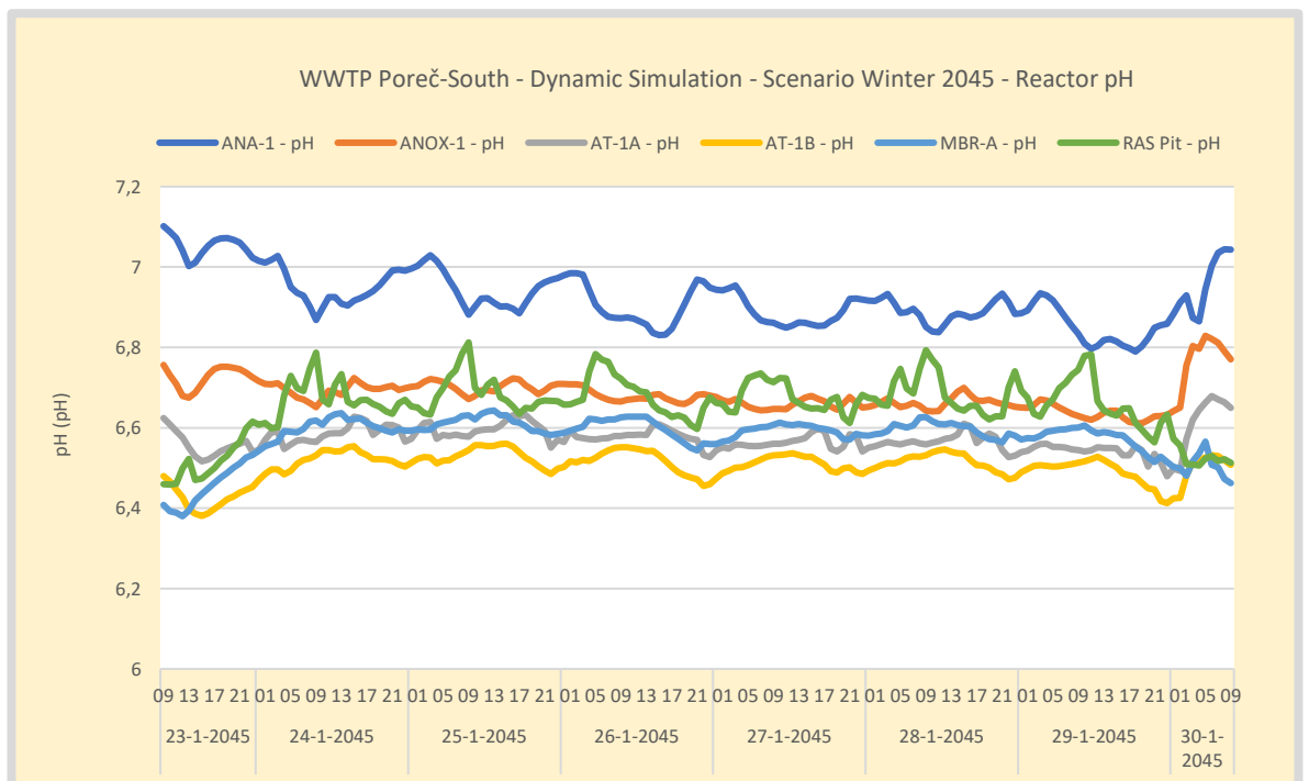
Figure 38. Simulation WWTP Poreč-South - Scenario Winter 2045 - pH profile over the activated sludge reactors. Influent pH is measured continuously and not limiting.
