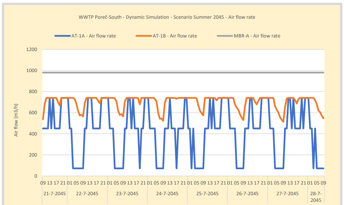
Figure 70. Simulation WWTP Poreč-South - Scenario Summer 2045 - air input in the different aerated reactors. AT-A is step controlled on NH4, AT-B is setpoint controlled on the DO, the MBR is fully aerated according to the design value.
