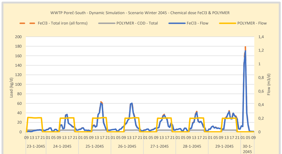
Figure 40. Simulation WWTP Poreč-South - Scenario Winter 2045 - load and flow of Iron and PE. Iron is dosed proportionally to a PO 4 measurement in the outflow of the MBR. PE is dosed to the dewatering and is assumed to be particulate biodegradable COD with a COD/VSS ratio of 1,42 gCOD/gTSS. Dosage is proportional to the WAS load based on 8 kg PE (dry weight) dosed per 1000 kg WAS (dry weight).
