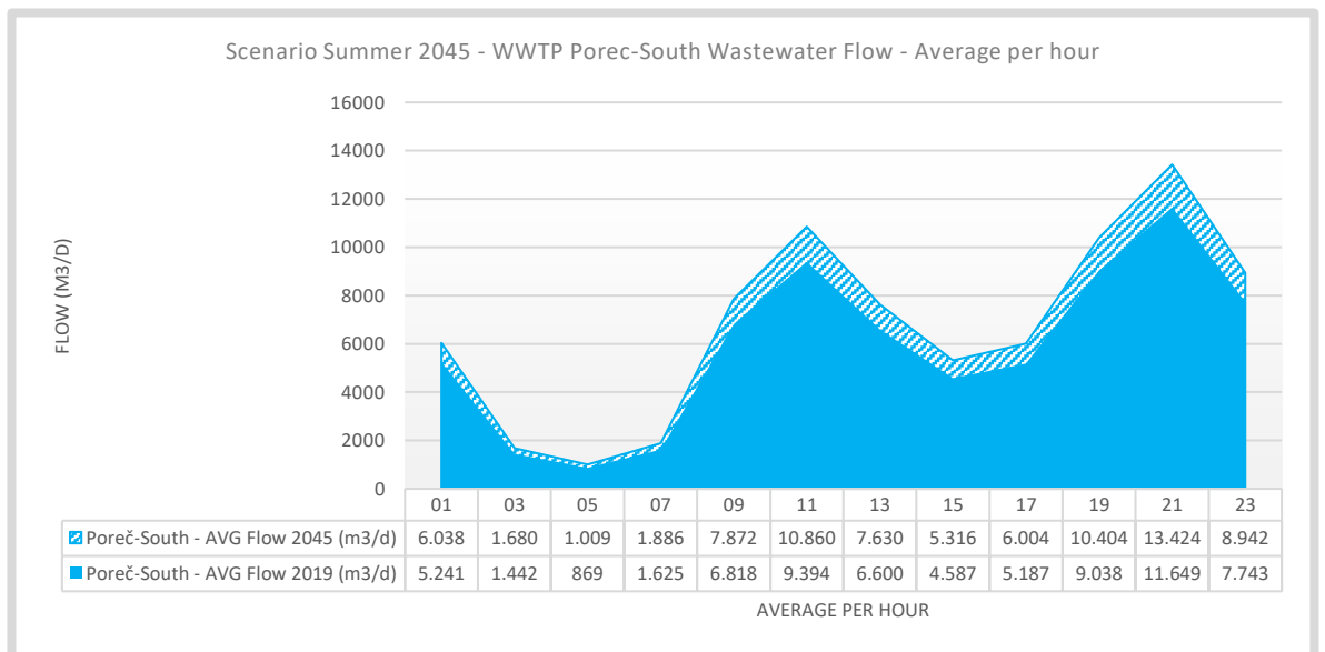
Figure 15. Scenario Summer 2045 – WWTP Poreč-South Wastewater Flow 24-hour average hourly 2019 measurements and 2045 prognosis. Data are used to reconstruct missing data in the flow measurements and for development of scenarios.
