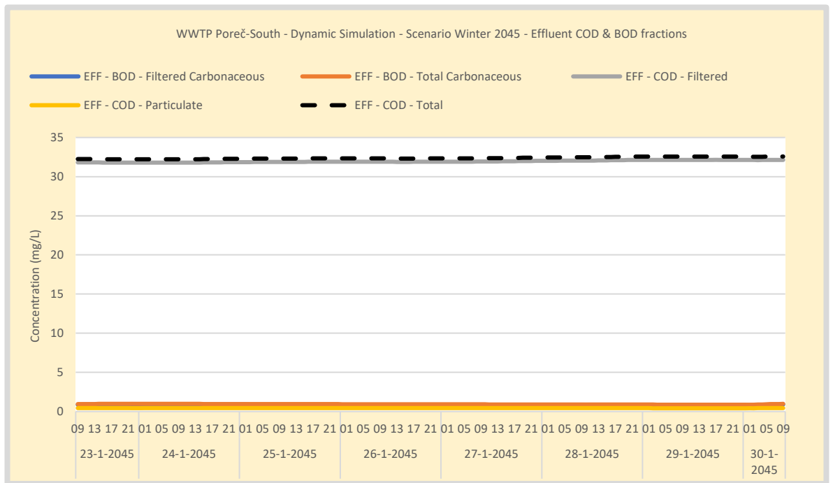
Figure 49. Simulation WWTP Poreč-South - Scenario Winter 2045 - Effluent COD and BOD concentration. Effluent is measured in the outflow of the large effluent buffer. COD is below the maximum required concentration. The Particulate fraction is the result of a MBR efficiency of 99,9% for particulate and 99,99% for colloidal material.
