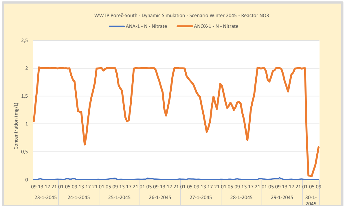
Figure 31. Simulation WWTP Poreč-South - Scenario Winter 2045 - nitrate in the anoxic tank. The anaerobic recycle rate is set to a maximum flow to reduce the effective anaerobic volume. The anoxic recycle is controlling nitrate in the anoxic tank on 2 mgNO 3 /L. This is done to avoid too long anaerobic HRT and decay of biomass. For part of the operation the anoxic recycle flow is insufficient to maintain the setpoint.
