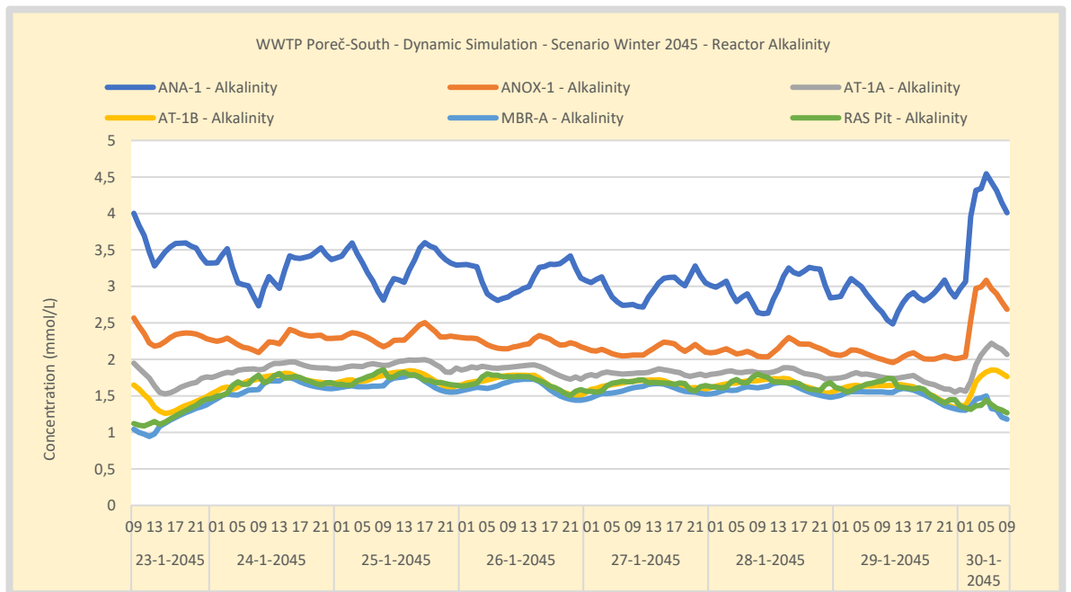
Figure 39. Simulation WWTP Poreč-South - Scenario Winter 2045 - alkalinity profile over the activated sludge reactors. Influent alkalinity is estimated from local drinking water quality measurements at 7,46 mmol/L. Alkalinity is sufficient. However, limitation of alkalinity in the winter may occur depending on operational conditions due to CO 2 stripping caused by over aeration.
