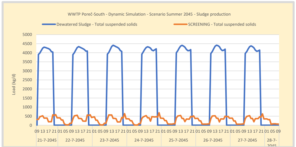
Figure 79. Simulation WWTP Poreč-South - Scenario Summer 2045 - dewatered sludge load and compacted screening load. Dewatered sludge is operated 10 hours a day at 23%. Screening is produced continuously as a factor of the influent and stored separately from the dewatered sludge.
