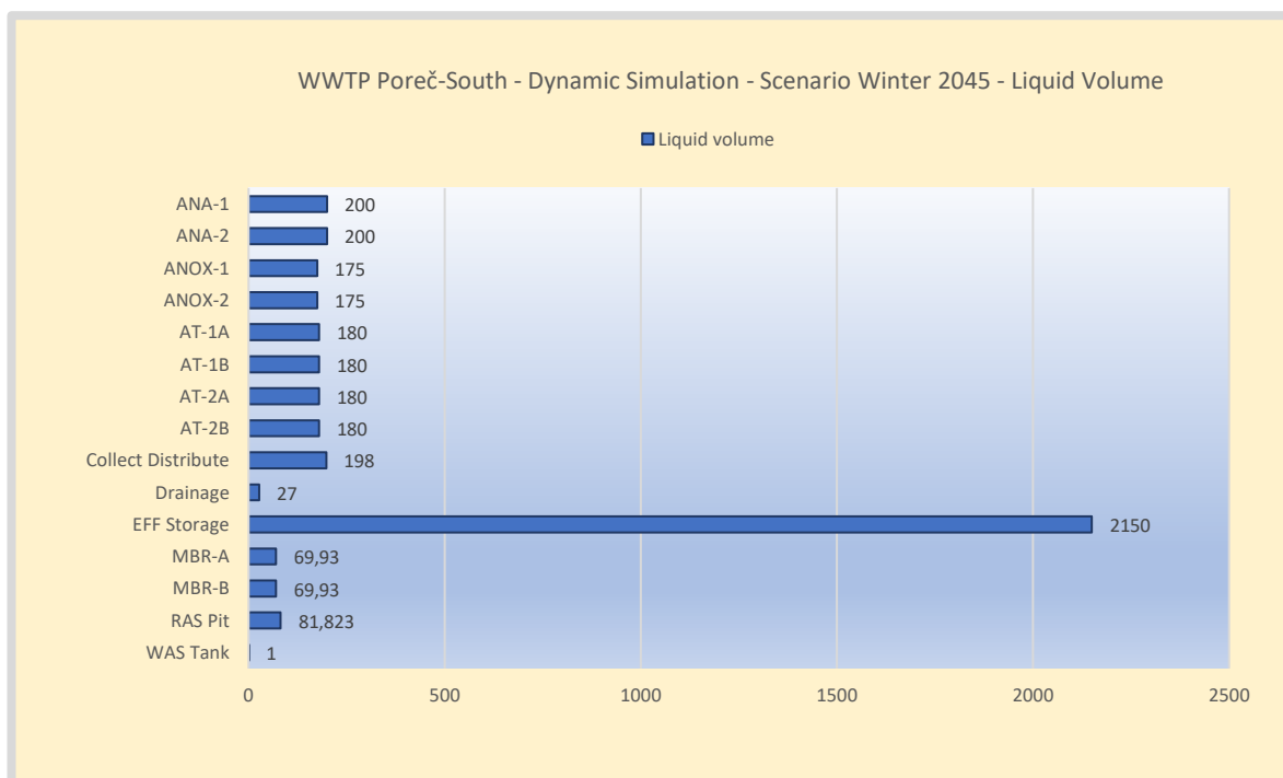
Figure 18. Simulation WWTP Poreč-South - Scenario Winter 2045 - Volume distribution of modelled reactor elements. The actual WAS tank is 150 m3 however, the sludge volume is modelled based on an HRT < 2,5 hours to avoid P-release. From the model it is concluded the WAS tank should not be used for longer storage of Bio-P sludge.
