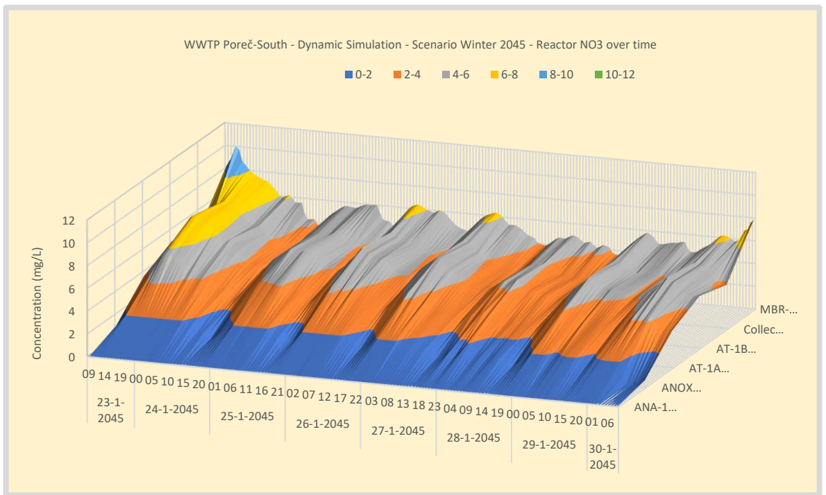
Figure 34. Simulation WWTP Poreč-South - Scenario Winter 2045 - NO3 concentration profile over the waterline.
