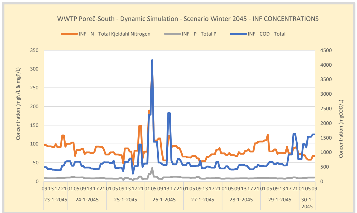
Figure 25. Simulation WWTP Poreč-South - Scenario Winter 2045 - Influent loads COD, TKN and TP. The profile is based on data measured in 2019 extrapolated towards 2045. In the data a large concentration peak is simulated. The larger peak occurs at low flow conditions and has a limited effect on the plant loading.
