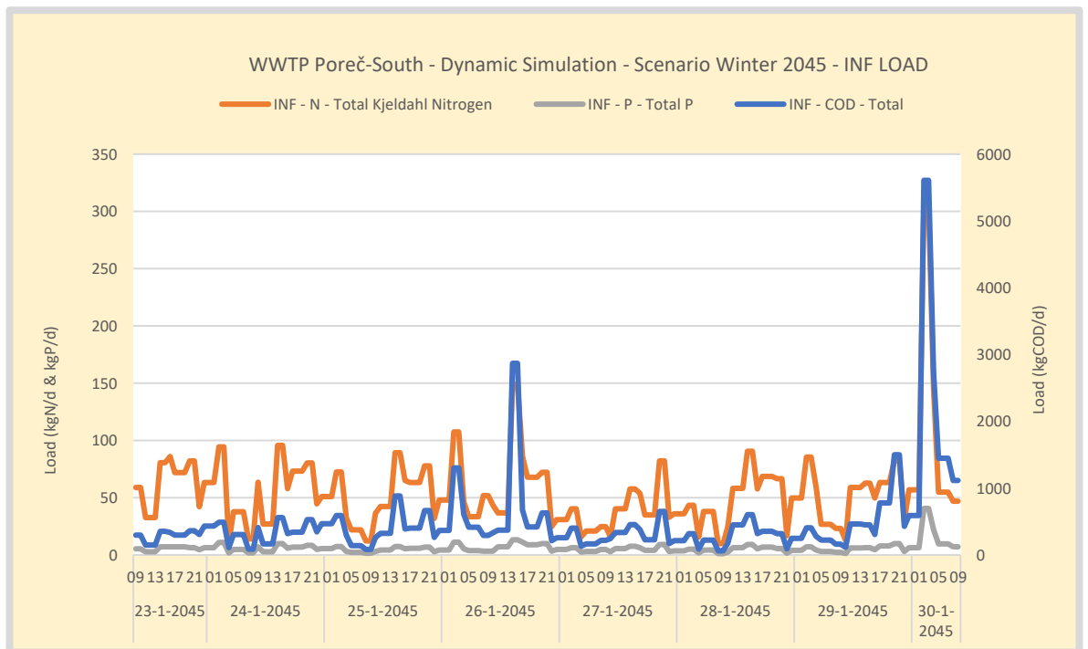
Figure 26. Simulation WWTP Poreč-South - Scenario Winter 2045 - Influent loads COD, TKN and TP. The profile is based on data measured in 2019 extrapolated towards 2045. The influent has peak loads at day 4 and 7. The larger concentration peak at day 4 occurs at low flow conditions and has a limited effect on the plant loading
