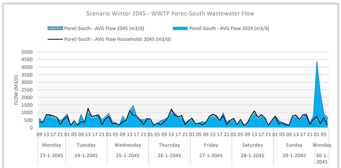
Figure 7. Scenario Winter 2045 – WWTP Poreč-South Wastewater Flow 24-hour 7-day dynamic 2019 measurements and 2045 prognosis. Both the 2019 and 2045 flow data are modelled and included in the scenario study. The 2045 data includes the growth of households and touristic activity.
