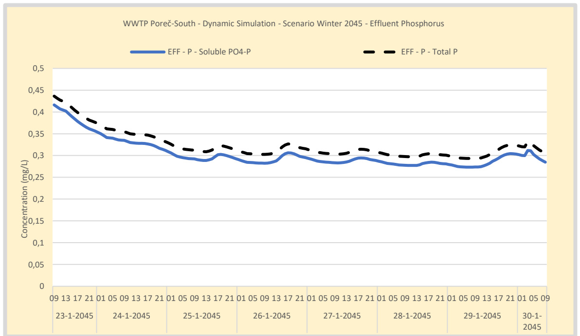
Figure 47. Simulation WWTP Poreč-South - Scenario Winter 2045 - Effluent phosphorus concentration. Effluent is measured in the outflow of the effluent buffer. In average TP is below the maximum required concentration.
