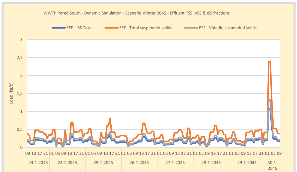
Figure 52. Simulation WWTP Poreč-South - Scenario Winter 2045 - Effluent suspended solids load. Effluent is measured in the outflow of the effluent buffer. The effluent load dynamics are the result of the flow dynamics. It is assumed that the MBR has a 99,9% removal efficiency for solids and 99,99% for colloidal material. Effluent VSS is related to the fecal load for sea water quality modelling.
