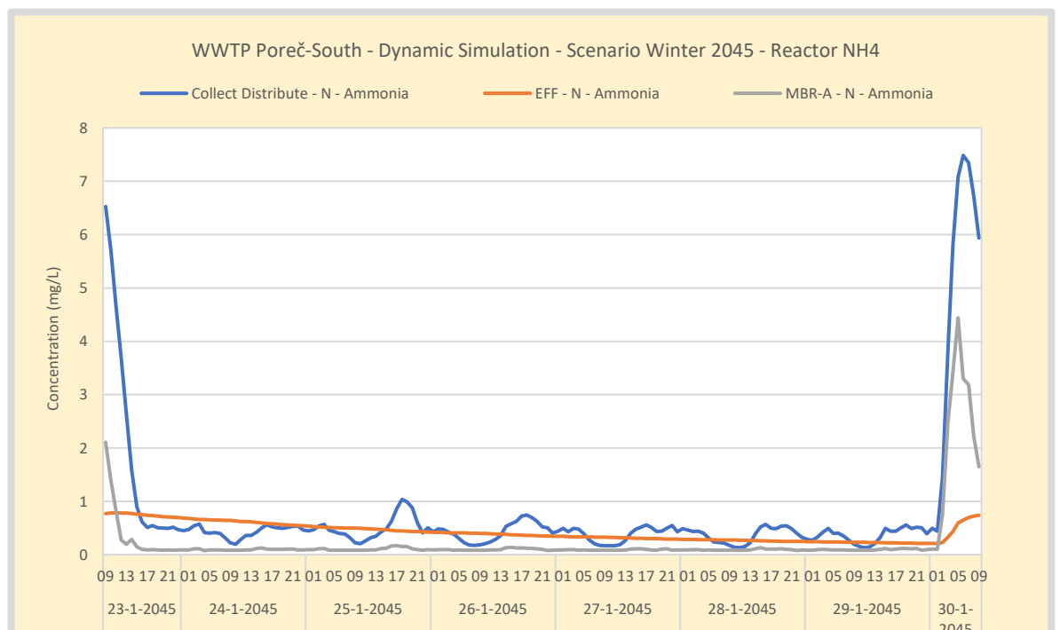
Figure 30. Simulation WWTP Poreč-South - Scenario Winter 2045 - ammonium profile in the waterline. The air input of AT-A is controlled based on NH4 in the Collect Distribute tank.
