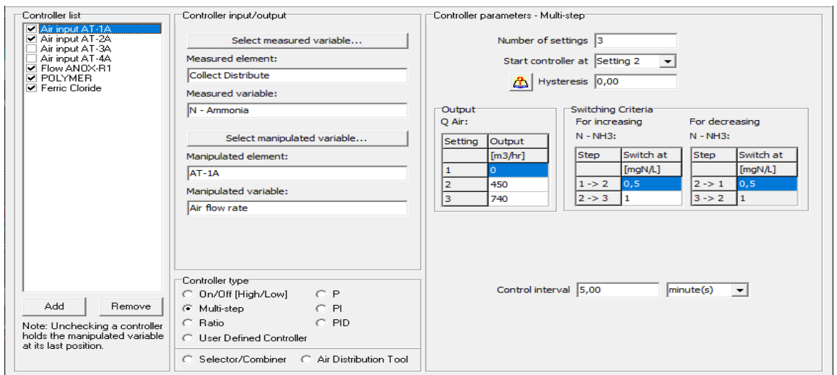
Figure 20. Simulation WWTP Poreč-South - Scenario Winter 2045 - Controlling the air input of AT-A. The measured variable is NH4 in the collect distribute tank. The manipulated variable the air flow in AT-A. There are 3 settings for the air flow depending on the NH4 concentration. Parallel lines are operated similar.
