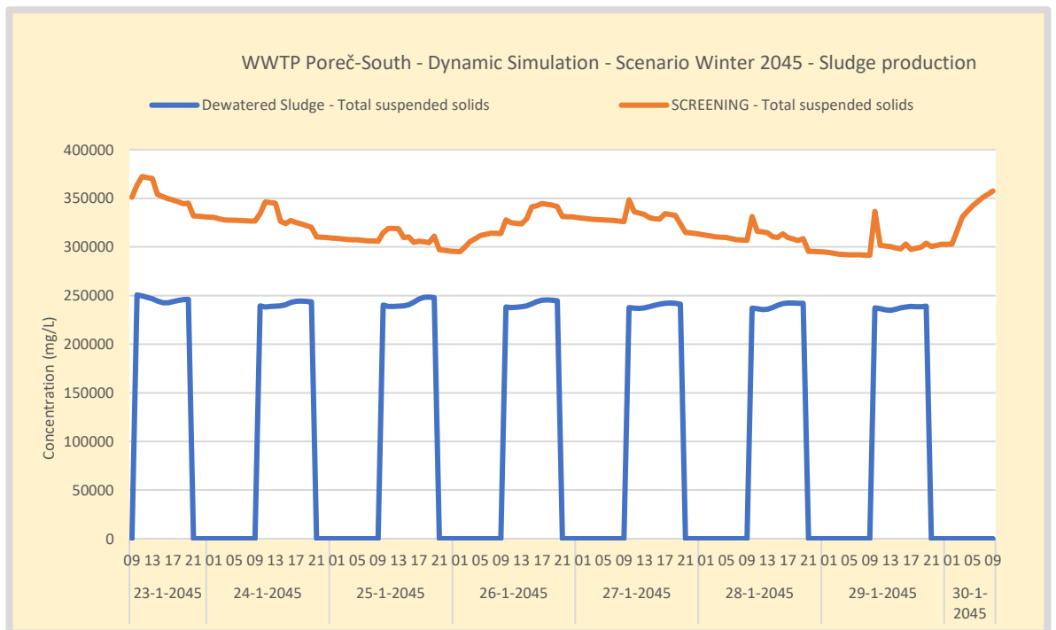
Figure 42. Simulation WWTP Poreč-South - Scenario Winter 2045 - dewatered sludge and screening sludge concentration. The design assumes dewatered sludge at approximately 23% dry matter. Screening is an estimated concentration as the result of the press operation.
