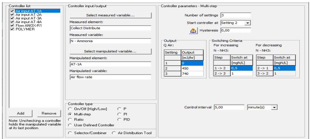
Figure 56. Simulation WWTP Poreč-South - Scenario Summer 2045 - Controlling the air input of AT-A. The measured variable is NH 4 in the collect distribute tank. The manipulated variable the air flow in AT-A. There are 3 settings for the air flow depending on the NH 4 concentration.
