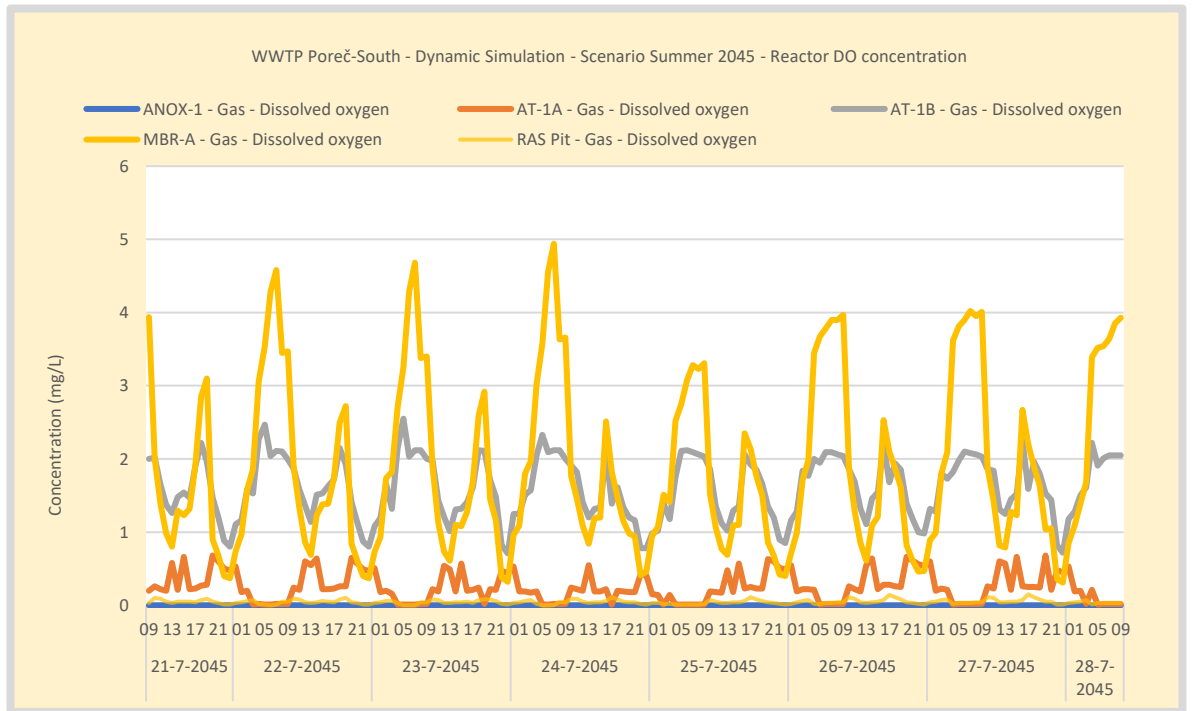
Figure 71. Simulation WWTP Poreč-South - Scenario Summer 2045 - DO concentration gradients. DO is controlled in the AT-B on 2 mgO 2 /L and the air flow of AT-B on NH 4 concentration in the outflow of the aeration. During influent TKN peak loading the air flow of AT-B is not sufficient to maintain the DO setpoint. The DO in the MBR is the result of the designed maximum air input. No oxygen is measured in the anoxic zone.
