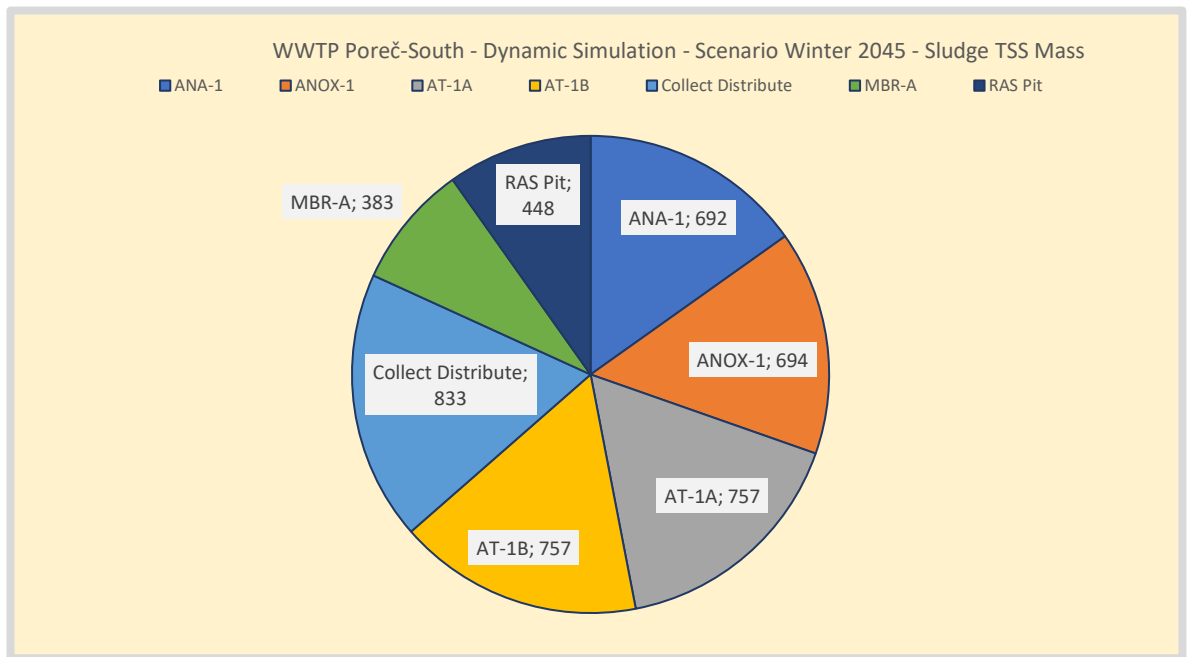
Figure 19. Simulation WWTP Poreč-South - Scenario Winter 2045 - Sludge mass distribution (kgTSS) in the activated sludge reactors. This data is used to calculate the SRT of the WWTP. Idle reactors are not included in SRT calculations.
