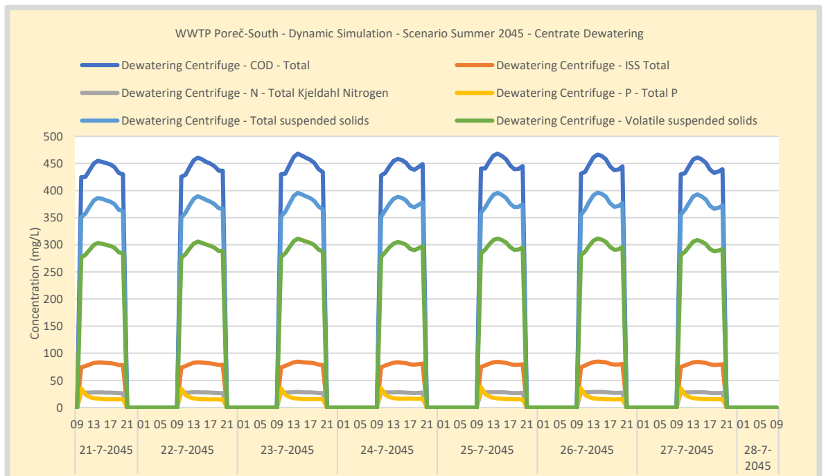
Figure 78. Simulation WWTP Poreč-South - Scenario Summer 2025 - Centrate concentrations dewatering.
