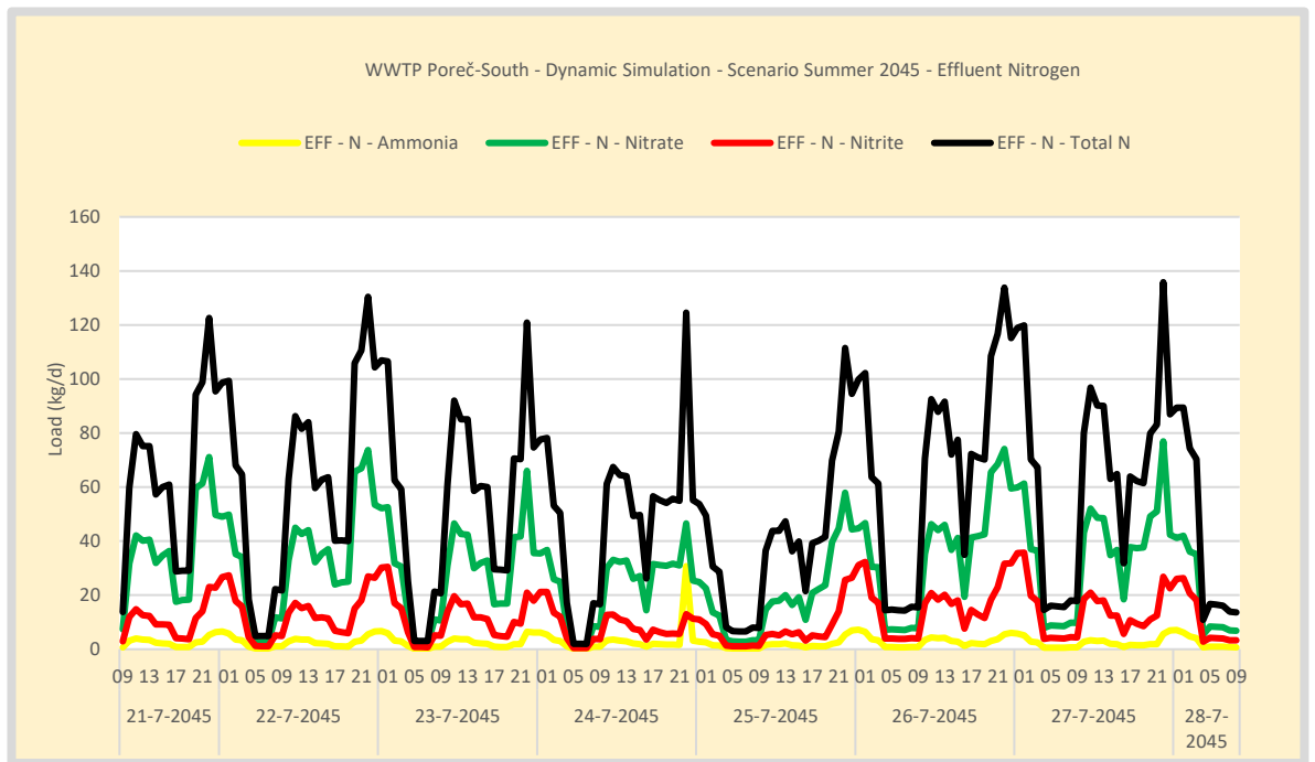
Figure 81. Simulation WWTP Poreč-South - Scenario Summer 2045 - Effluent nitrogen load. Effluent is measured in the outflow of the large effluent buffer. Fluctuations are mainly the result of flow variation.
