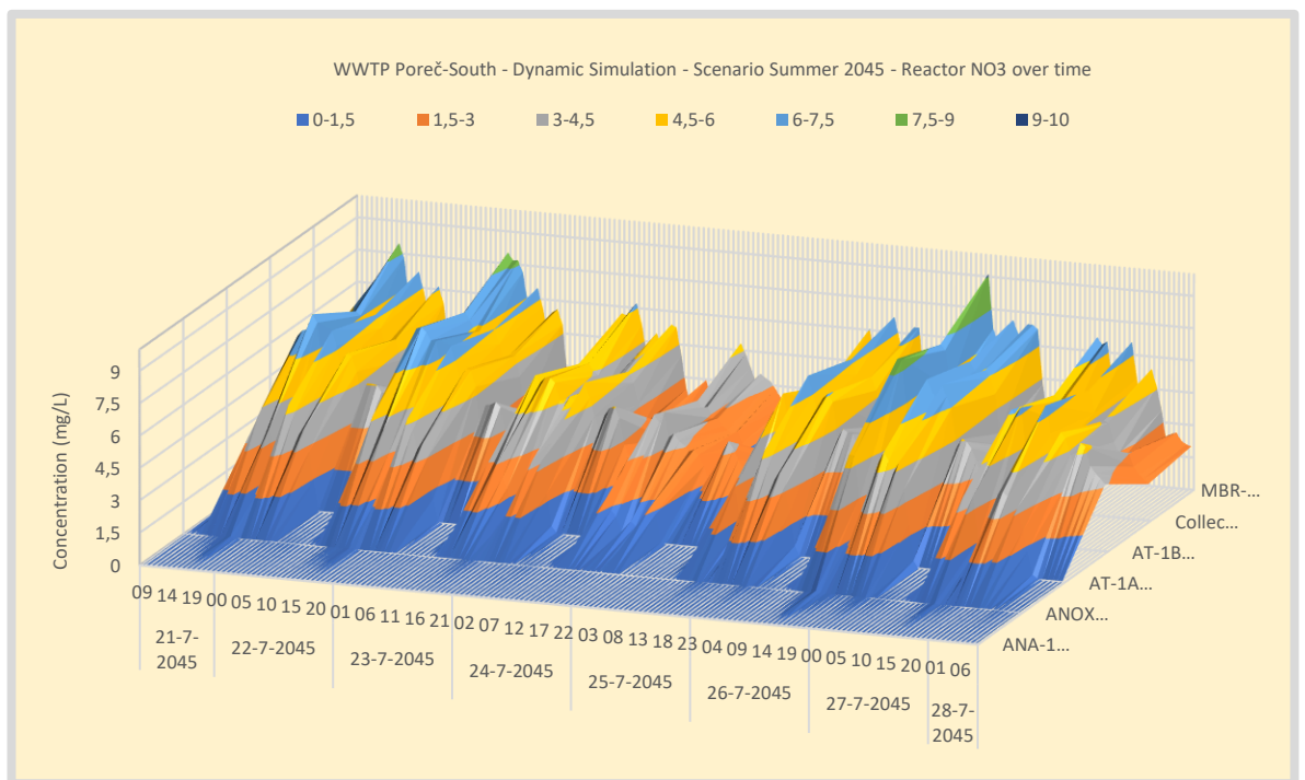
Figure 68. Simulation WWTP Poreč-South - Scenario Summer 2045 - NO3 concentration profile over the waterline.
