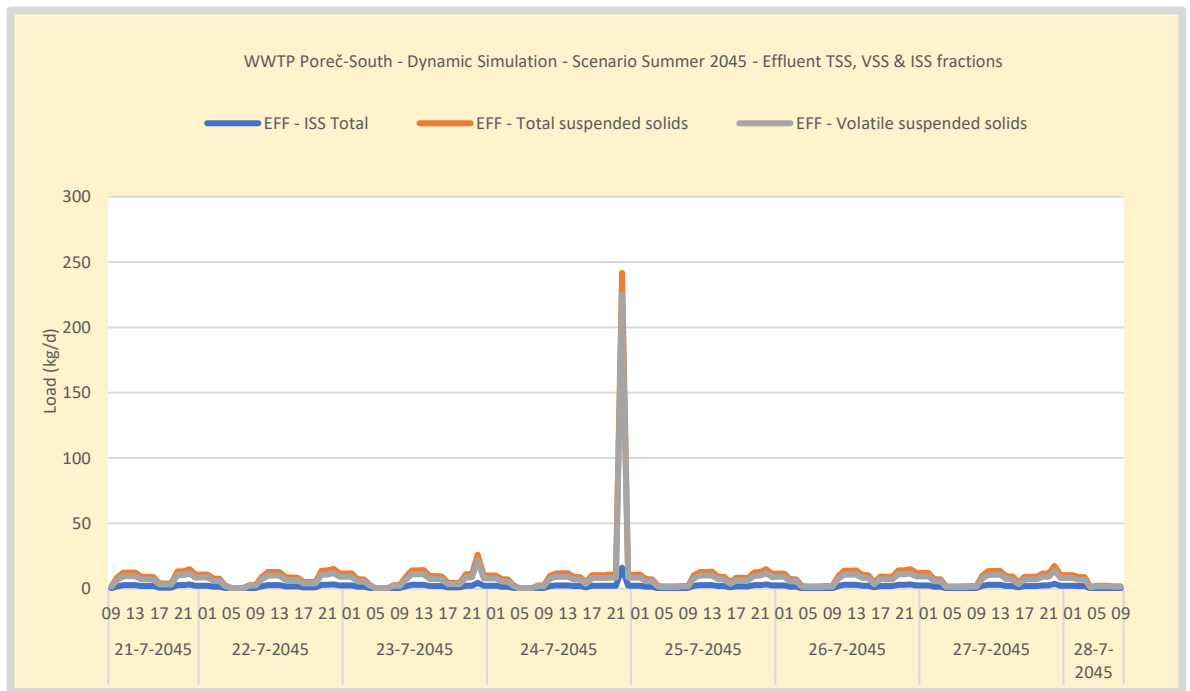
Figure 87. Simulation WWTP Poreč-South - Scenario Summer 2045 - Effluent TSS, VSS and ISS load. The Particulate fraction is the result of a MBR efficiency of 99,9% for particulate and 99,99% for colloidal material. Load variations are mainly due to flow variations. Effluent VSS is related to the fecal load for sea water quality modelling. At 22 hours on day 4, a bypass event is simulated due to a hydraulic peak loading.
