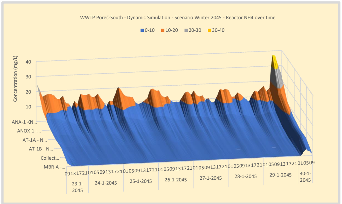
Figure 33. Simulation WWTP Poreč-South - Scenario Winter 2045 - NH4 concentration profile over the waterline.
