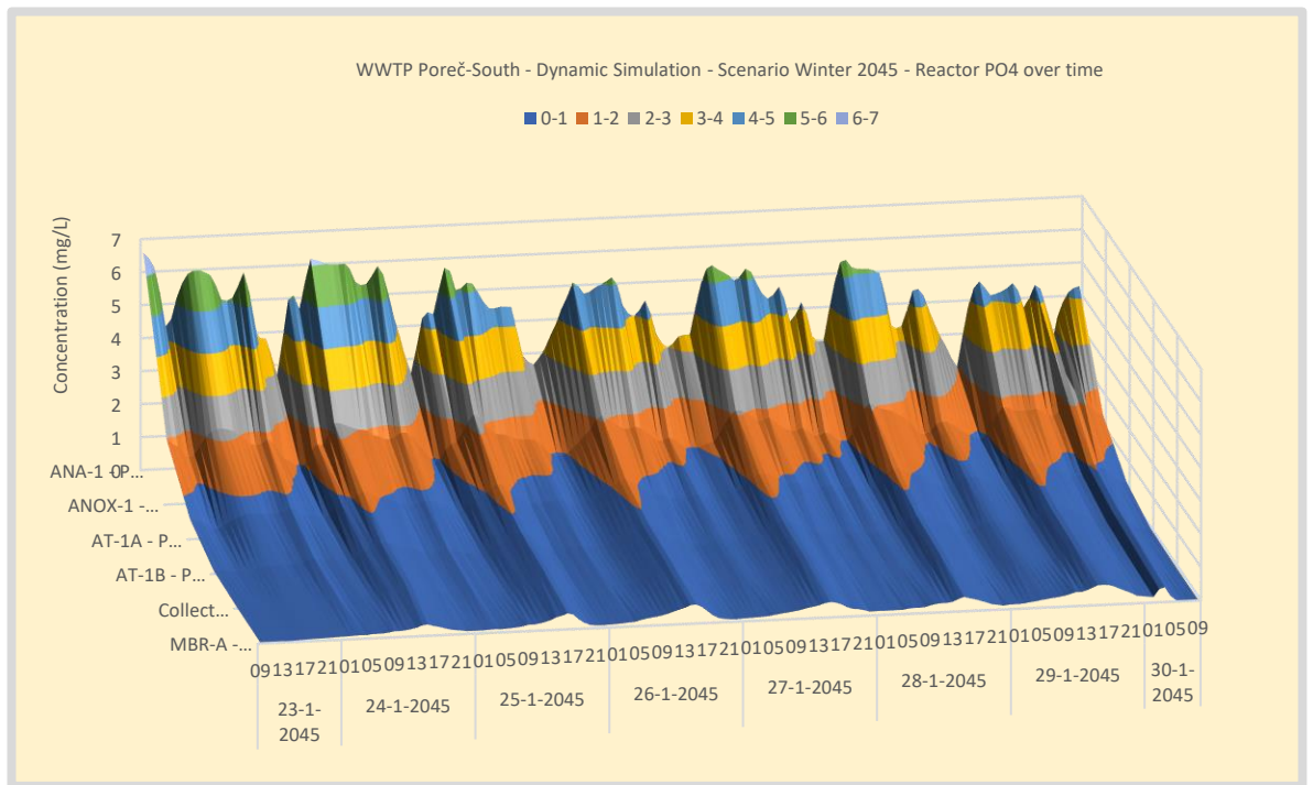
Figure 35. Simulation WWTP Poreč-South - Scenario Winter 2025 - PO4 concentration profile over the waterline.
