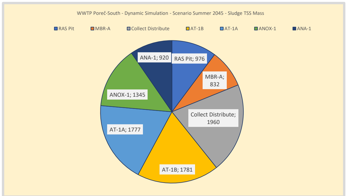
Figure 55. Simulation WWTP Poreč-South - Scenario Summer 2045 - Sludge mass distribution (kgTSS) in the activated sludge reactors. This data is used to calculate the SRT of the WWTP. Idle reactors containing sludge are not included in SRT calculations.
