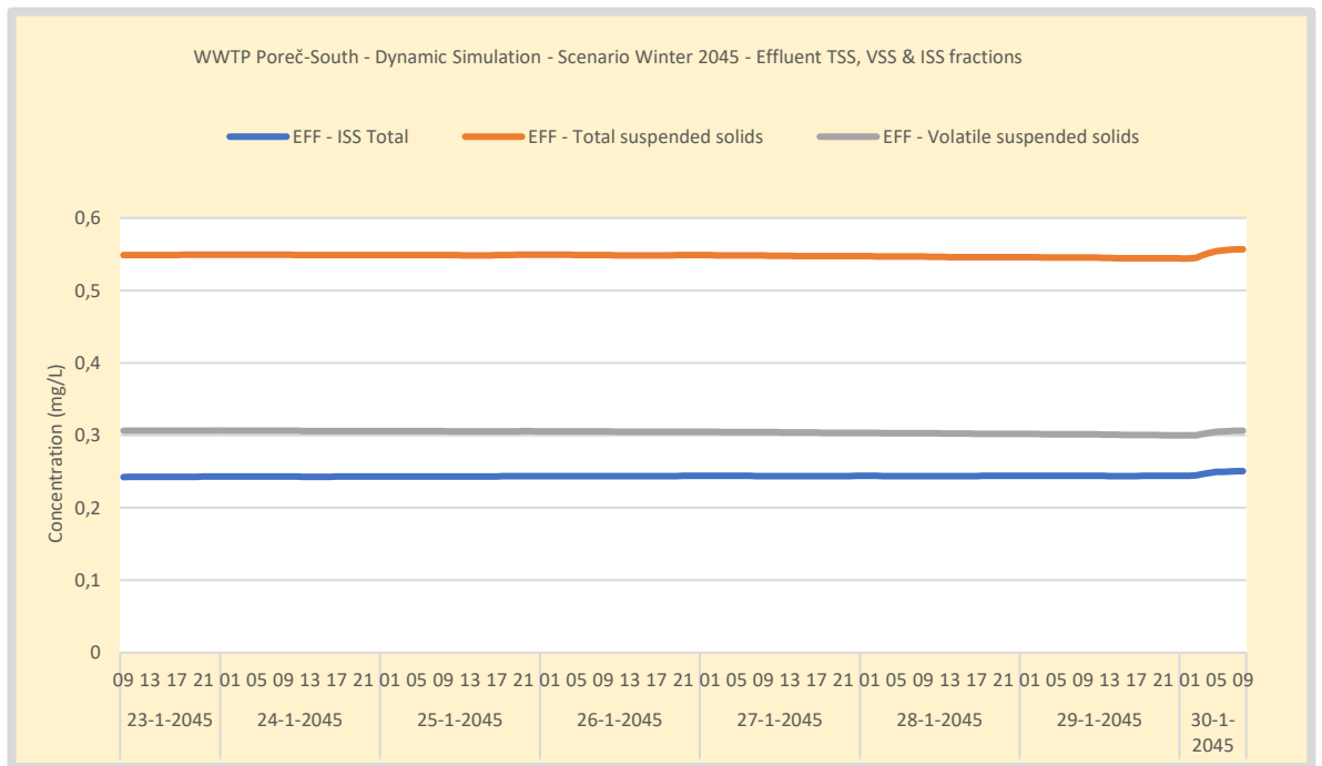
Figure 51. Simulation WWTP Poreč-South - Scenario Winter 2045 - Effluent suspended solids concentration. Effluent is measured in the outflow of the effluent buffer. It is assumed that the MBR has a 99,9% removal efficiency for solids and 99,99% for colloidal material and that this performance is not affected in time.
