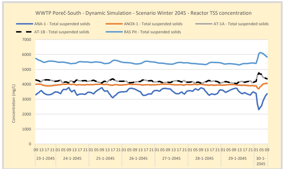
Figure 29. Simulation WWTP Poreč-South - Scenario Winter 2045 - TSS profile in the waterline. TSS in the MBR is controlled on approximately 5,5 gTSS/L by adjusting the WAS flow and SRT. In the winter the volume of the activated sludge system is high relative to the influent loading resulting in long SRT and low sludge production.
