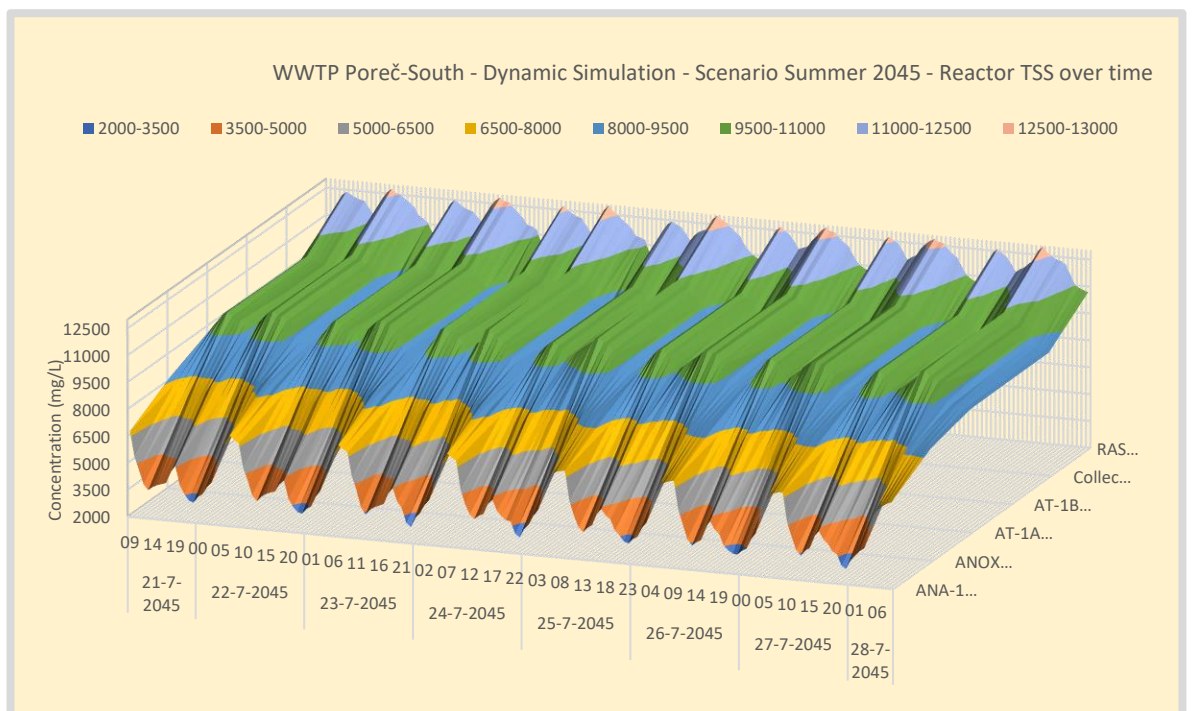
Figure 66. Simulation WWTP Poreč-South - Scenario Summer 2045 - TSS concentration profile over the waterline.
