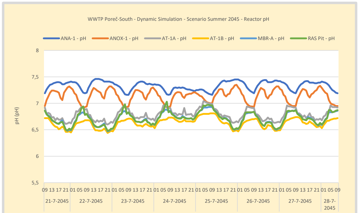
Figure 72. Simulation WWTP Poreč-South - Scenario Summer 2045 - pH profile over the activated sludge reactors. Influent pH is measured continuously and not limiting.
