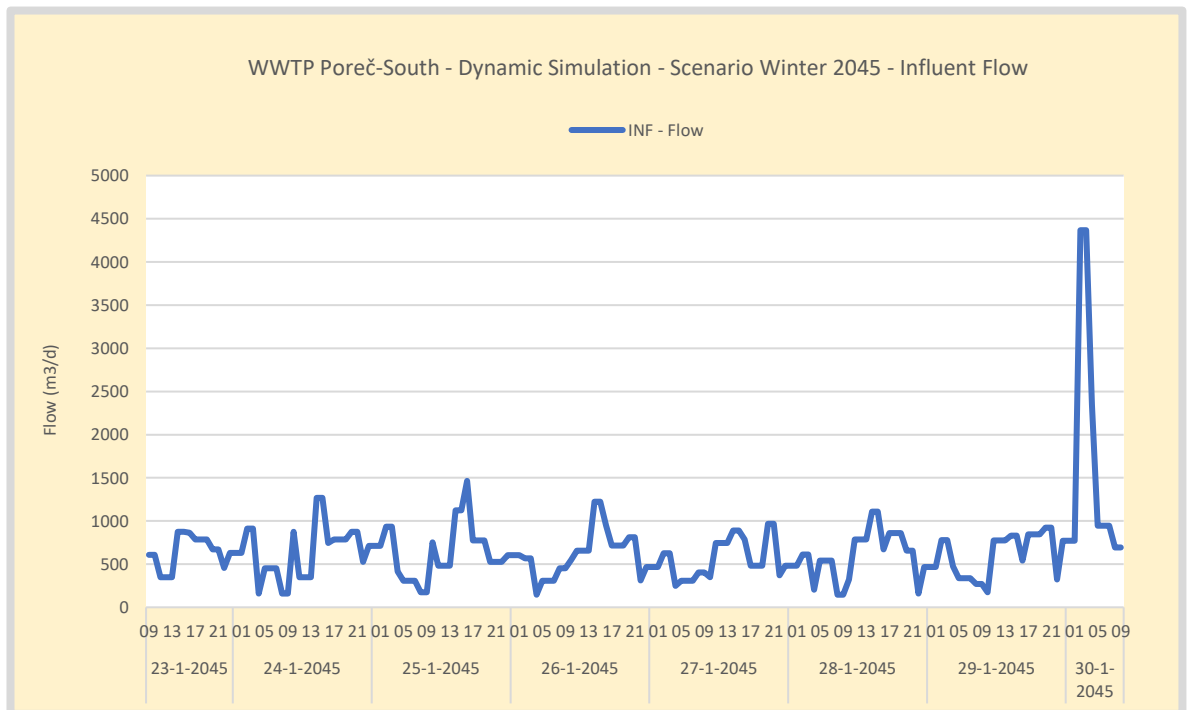
Figure 24. Simulation WWTP Poreč-South - Scenario Winter 2045 - Influent flow. The profile is based on data measured in 2019 extrapolated towards 2045. Day 7 has a large rain event.
