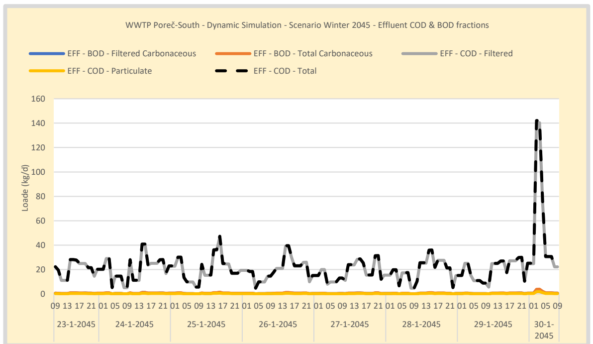
Figure 50. Simulation WWTP Poreč-South - Scenario Winter 2045 - Effluent COD and BOD load. Effluent is measured in the outflow of the large effluent buffer. Variations in the load are largely the result of flow variations. The Particulate fraction is the result of a MBR efficiency of 99,9% for particulate and 99,99% for colloidal material.
