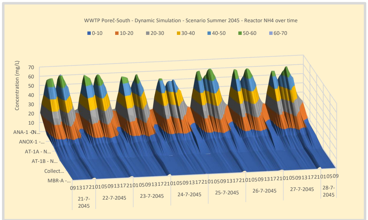
Figure 67. Simulation WWTP Poreč-South - Scenario Summer 2045 - NH4 concentration profile over the waterline.
