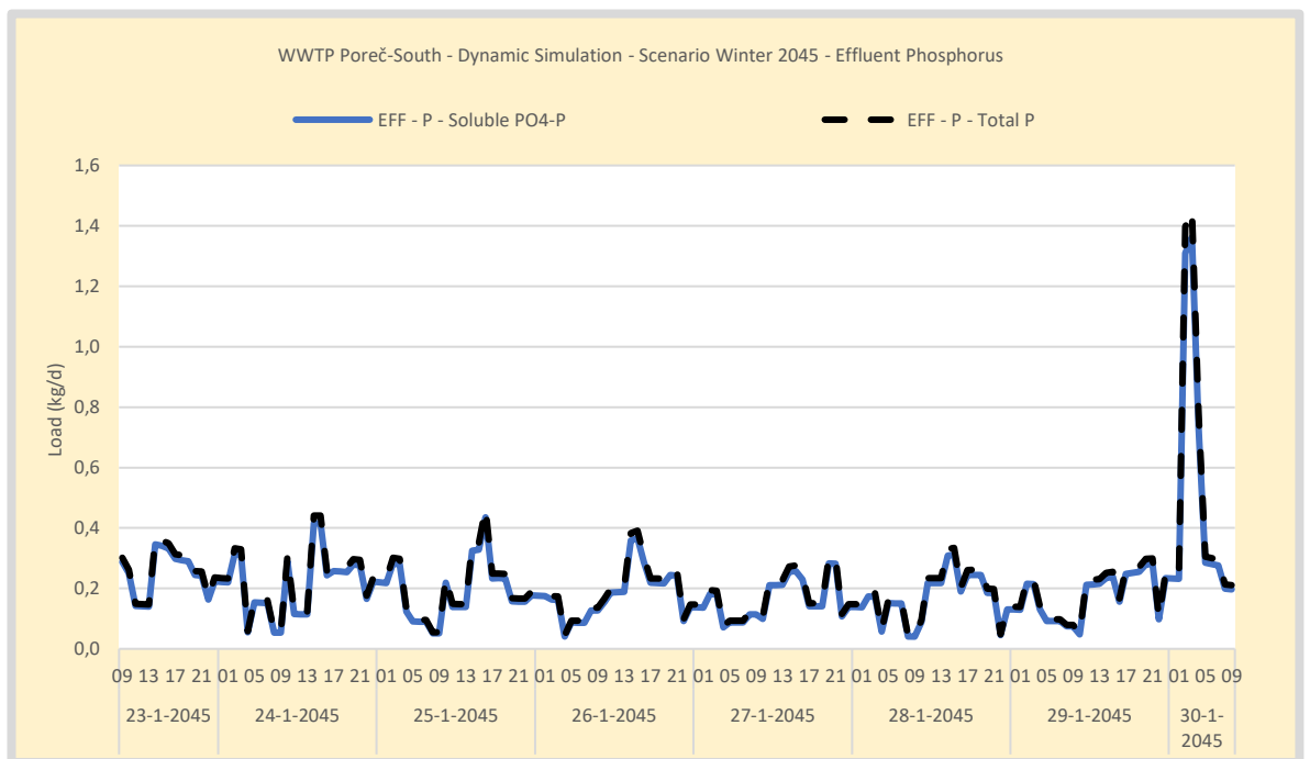
Figure 48. Simulation WWTP Poreč-South - Scenario Winter 2045 - Effluent phosphorus load. The last day is a major rain event negatively affecting P-removal. Effluent is measured in the outflow of the effluent buffer. Variations in the effluent load are mainly the result of variations the flow.
