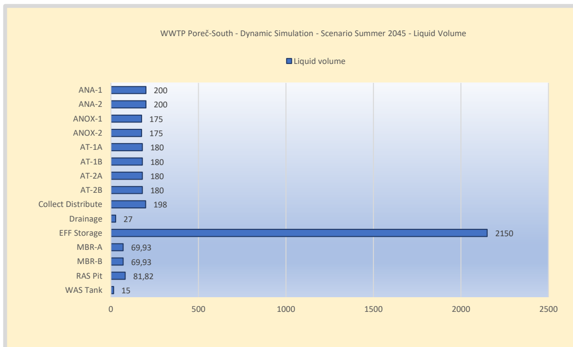
Figure 54. Simulation WWTP Poreč-South - Scenario Summer 2045 - Volume distribution of modelled reactor elements. The actual WAS tank is 150 m3 however the sludge volume is modelled based on an HRT less than 2,5 hours to avoid P-release. From the model it is concluded the WAS tank should not be used for storage of Bio-P sludge.
