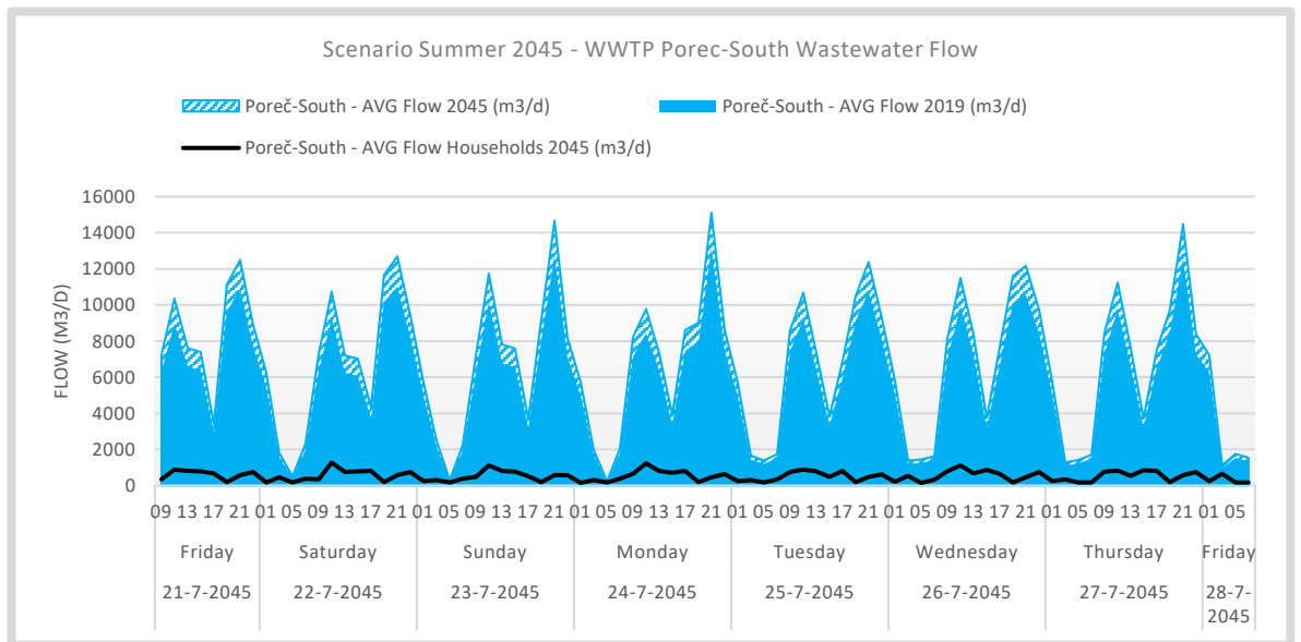
Figure 14. Scenario Summer 2045 – WWTP Poreč-South Wastewater Flow 24-hour 7-day dynamic 2019 measurements and 2045 prognosis. Both the 2019 and 2045 flow data are used for dynamic modelling. The 2045 data includes the growth of households and touristic activity.
