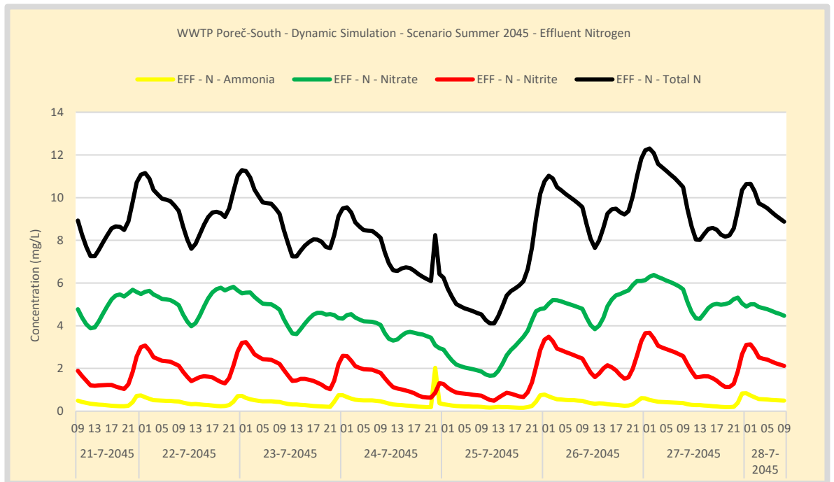
Figure 80. Simulation WWTP Poreč-South - Scenario Summer 2045 - Effluent nitrogen concentration. Effluent is measured in the outflow of the large effluent buffer. Some Nitrite is produced indicating limiting aeration capacity during peak loading. The average effluent concentration is below the maximum requirement. At 22 hours on day 4, a bypass event is simulated due to a hydraulic peak loading.
