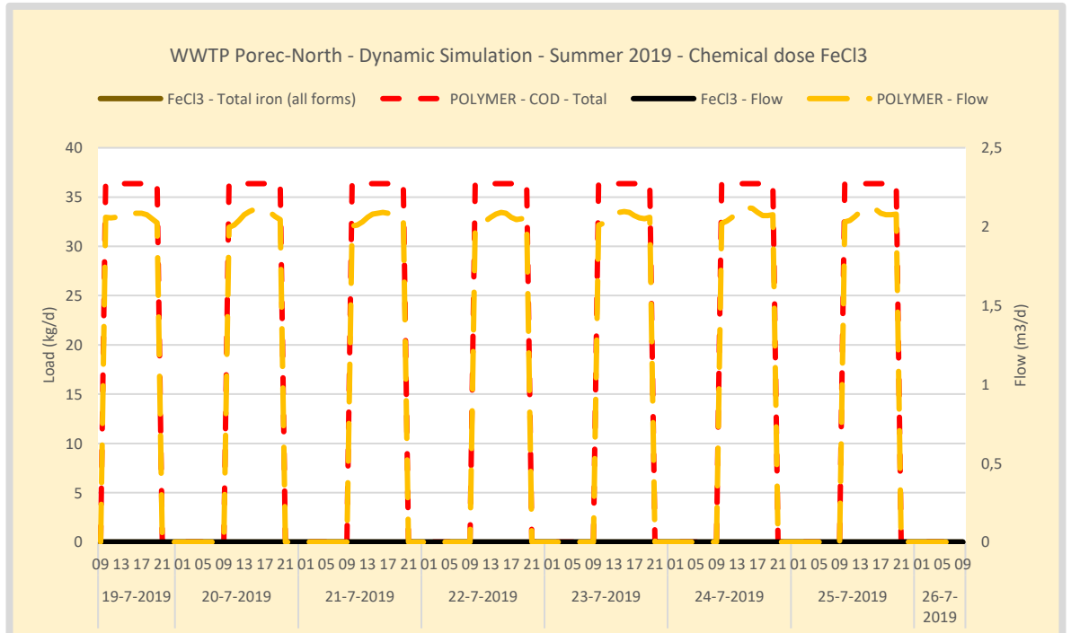
Figure 130. Summer – WWTP Poreč-North load and flow of Iron and PE. No iron is dosed. PE is assumed particulate biodegradable COD with a COD/VSS ratio of 1,42 gCOD/gTSS and dosed
