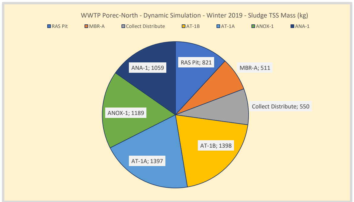
Figure 82. Winter – WWTP Poreč-North sludge mass distribution (kgTSS) in the reactor tanks. Based on these data and the average sludge production, the SRT of the WWTP is calculated. Mass of idle tanks is not included.
