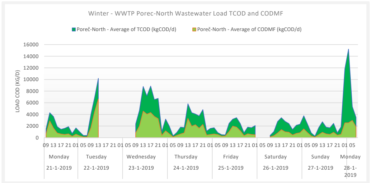
Figure 50. Winter – WWTP Poreč-North Influent Total and filtered COD Loads based on 7 measurement days. A rain event occurred Monday 28-01-2019. Some data is missing. For modelling missing data points (22 and 26-1) are reconstructed based on the hourly average dry weather load.
