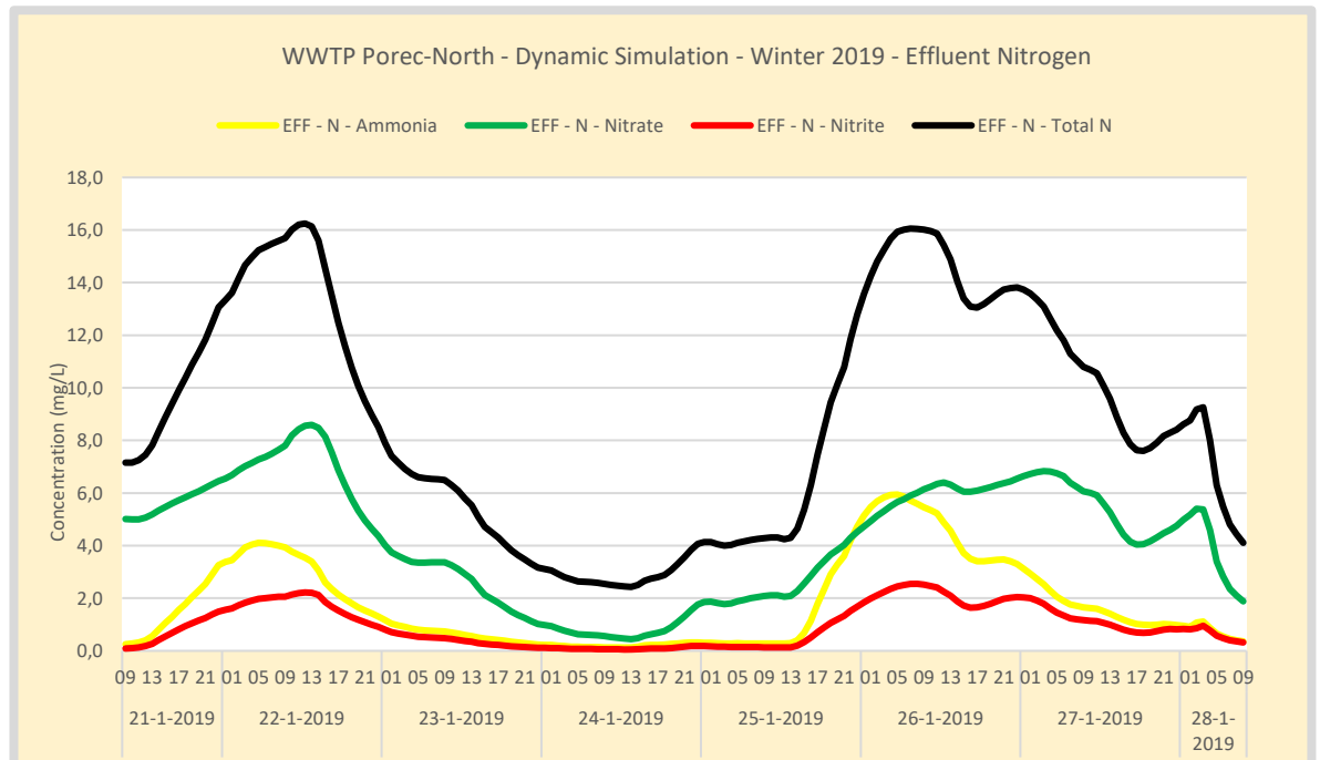
Figure 106. Winter – WWTP Poreč-North Effluent nitrogen concentration. Effluent is measured in the outflow of the large effluent buffer.
