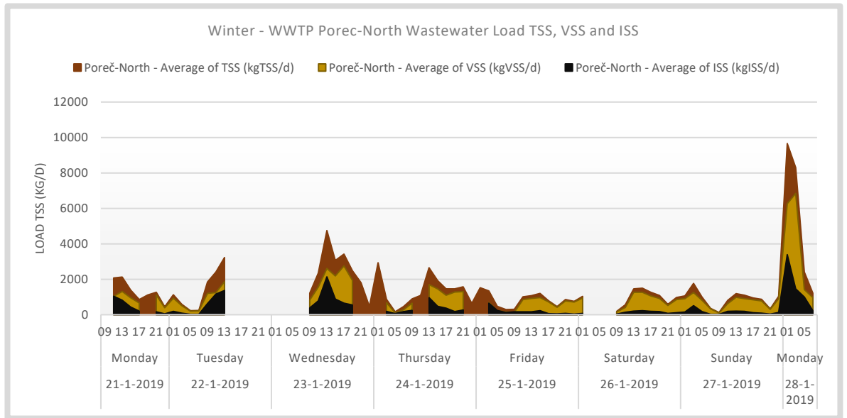
Figure 74. Winter – WWTP Poreč-North Influent TSS, VSS and ISS Loads based on 7 measurement days. A rain event occurred Monday 28-01-2019. For the model input missing data points are reconstructed based on the hourly average dry weather load. In practice TSS is difficult to get a homogeneous sample of TSS. TSS is easily biased, especially when automated samplers are used. This often results in high measurement variations.
