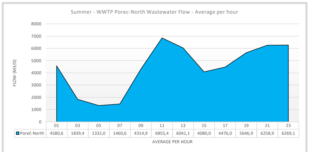
Figure 14. Summer - WWTP Poreč-North Wastewater Flow 24-hour average hourly measurements. Data are used to reconstruct missing data in the flow measurements and for development of scenarios.
