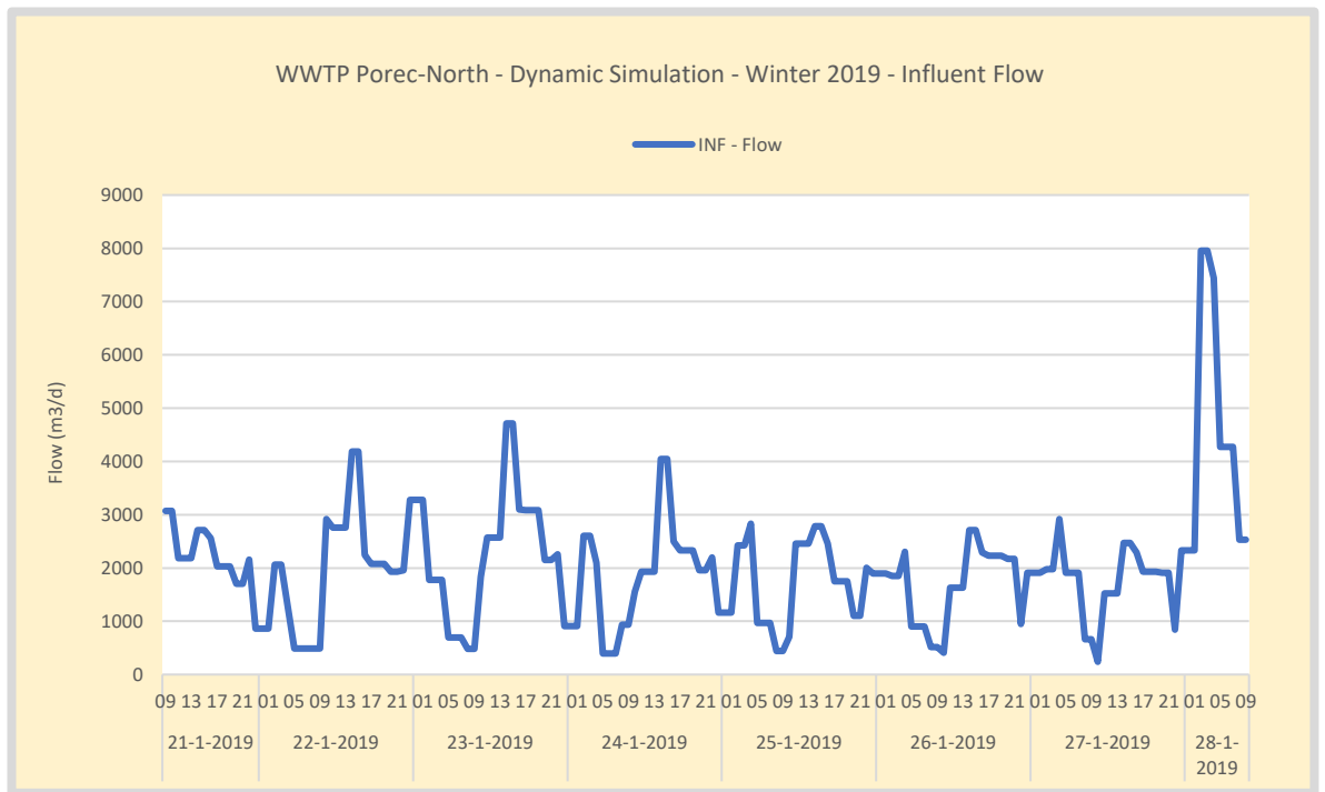
Figure 8. Winter – BioWin modelling WWTP Poreč-North: Wastewater Flow 24-hour 7-day dynamic model input data. Some datapoint are reconstructed from 24-hour average hourly measurements. The data is interpolated in the model on an hourly basis.
