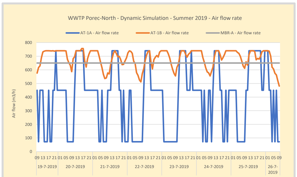
Figure 126. Summer – WWTP Poreč-North air input in the different aerated reactors. AT-A is step controlled on NH4, AT-B is setpoint controlled on the DO, the MBR is fully aerated according to the design value.
