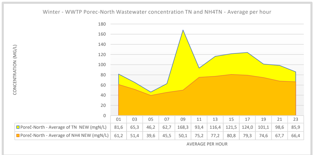
Figure 25. Winter – WWTP Poreč-North 24-hour average TN and NH4 influent Concentration.
