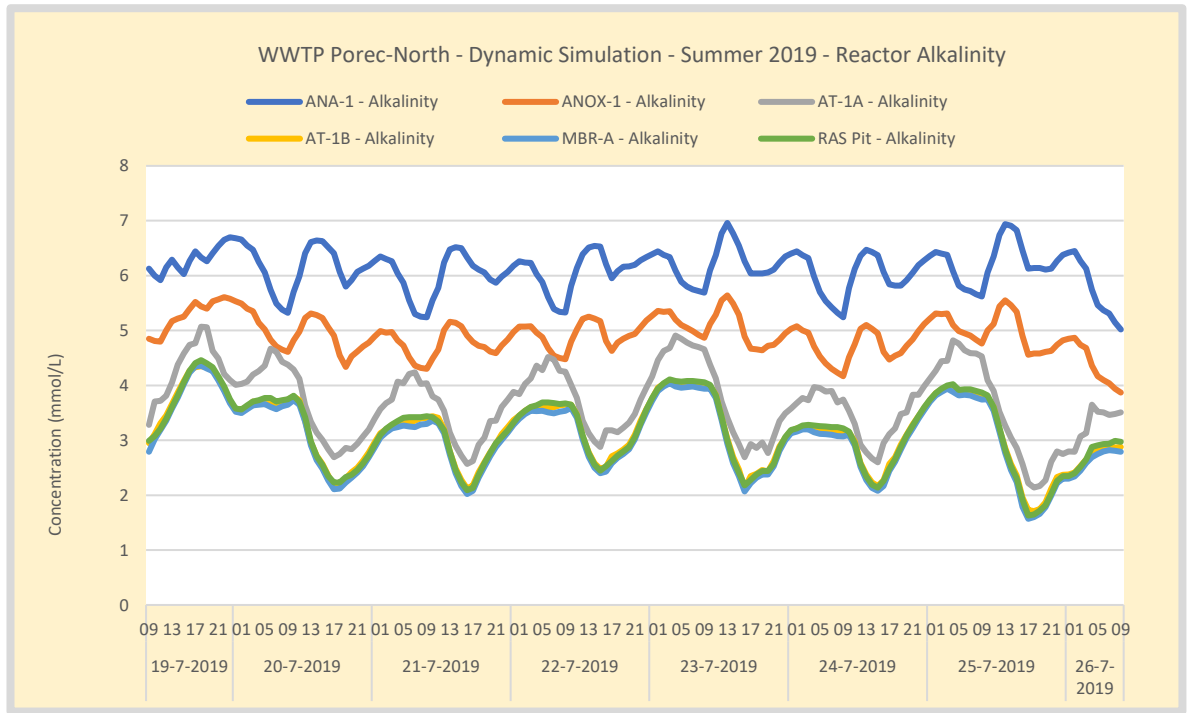
Figure 129. Summer – WWTP Poreč-North alkalinity profile over the activated sludge reactors. Influent alkalinity is estimated from local drinking water quality measurements at 7,46 mmol/L. Alkalinity is not becoming zero however potentially limiting under the operated conditions.
