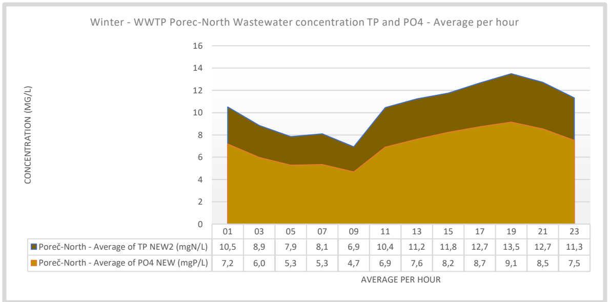
Figure 31. Winter – WWTP Poreč-North 24-hour average TP and PO4 influent Concentration.
