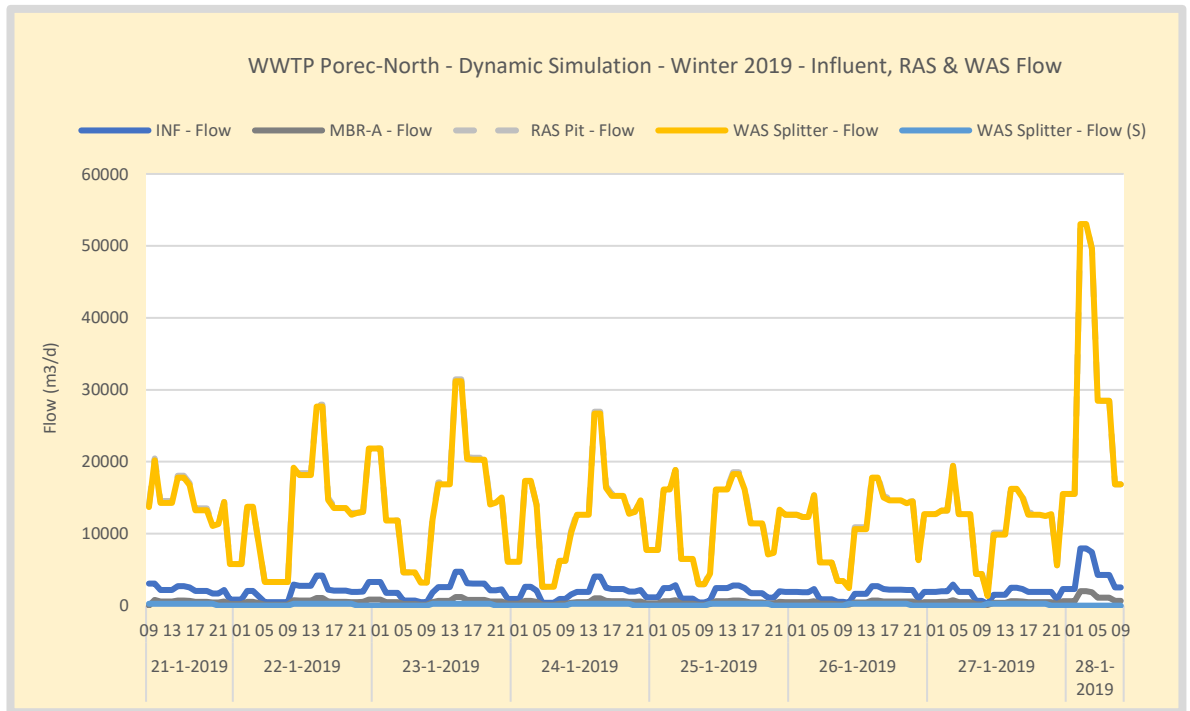
Figure 88. Winter – WWTP Poreč-North flow rate settings and control. The MLSS sludge return flow is controlled proportional to the influent. This results in a more stable TSS concentration in the reactors. The WAS flow is operated 10 hours a day on a constant flow to the dewatering.
