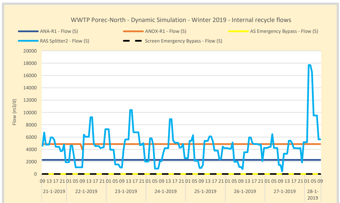
Figure 89. Winter – WWTP Poreč-North flow rate settings and control. The bypasses are not used. The anoxic recycle is controlled based on nitrate in the anoxic tank. The flow is reduced when Nitrate becomes higher than 2 mgNO 3 /L. This does not occur indicating that the anoxic tank is too large for the low loading conditions.
