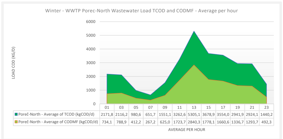
Figure 51. Winter – WWTP Poreč-North hourly average dry weather influent loads of total and filtered COD, based on 7 measurement days, excluding the rain event Monday 28-01-2019. This data is used to reconstruct missing data points in 7-day measurement series.
