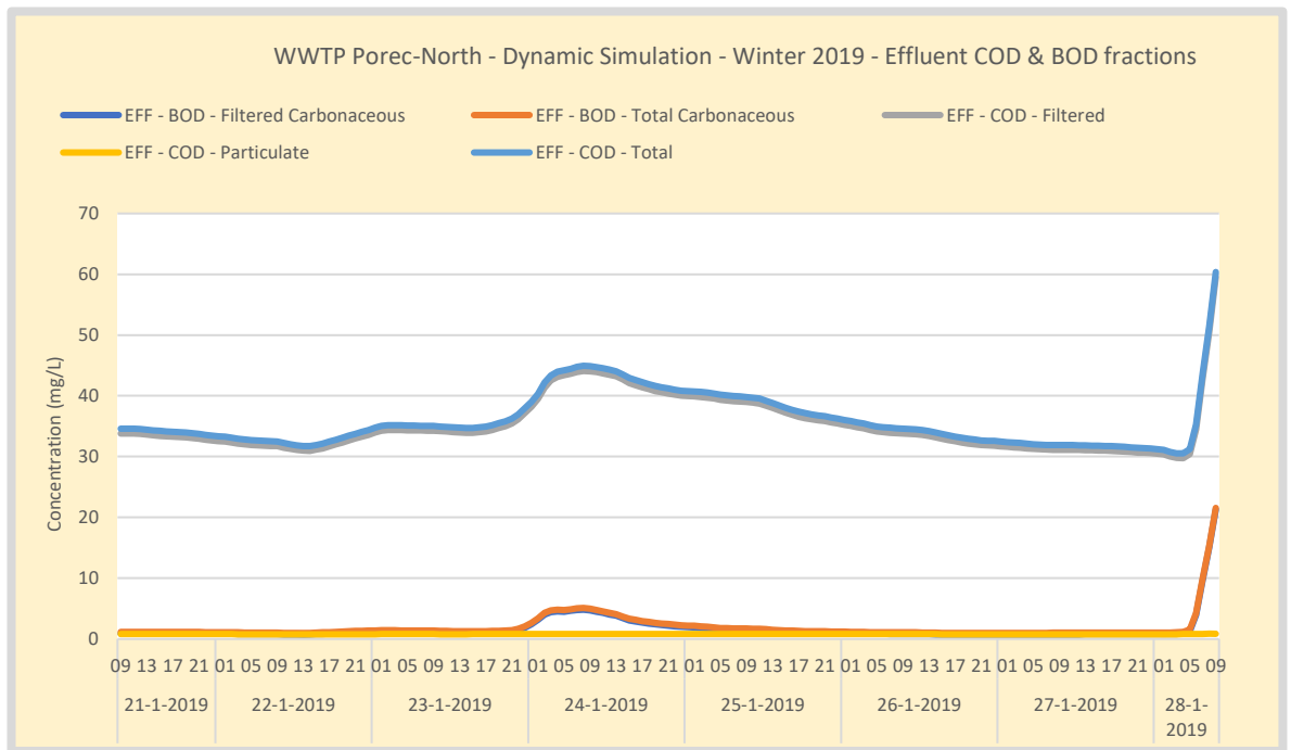
Figure 108. Winter – WWTP Poreč-North Effluent COD and BOD concentration. Effluent is measured in the outflow of the large effluent buffer.
