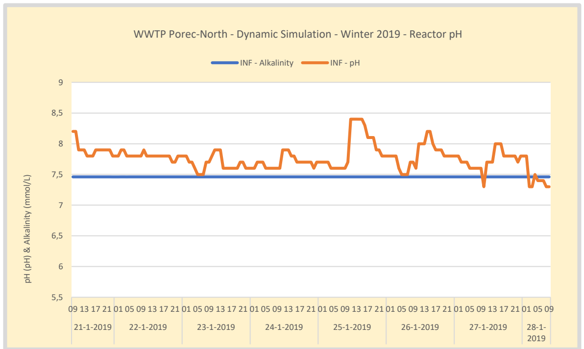
Figure 43. Dynamic Simulation – WWTP Poreč-North – Winter 24-hour average influent pH measurement. pH is a dynamic model input. The alkalinity of wastewater is estimated from Poreč drinking water quality. 28-01-2019 a major rain event occurred. The peaks 25 and 26-1 coincide with other measured parameters indicating a nondomestic discharge.
