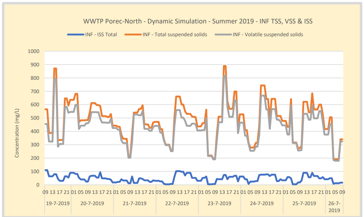
Figure 41. Dynamic Simulation – WWTP Poreč-North – Summer 24-hour average TSS, VSS (organic particulate) and ISS (inorganic particulate) influent Concentration. The model input is the measured and reconstructed ISS concentration. VSS is calculated based on (constant) fractions determined in the influent specification. TSS is modelled as the sum of ISS and VSS. No rain occurred. Peak are measured 19 and 23-7 indicating measurement errors.
