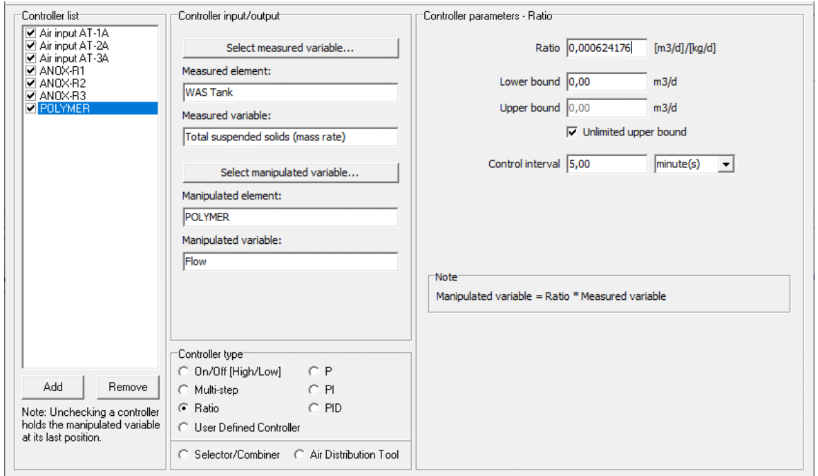
Figure 114. Summer – WWTP Poreč-North BioWin controller toolbox used for controlling the polymer dosage of the dewatering. Indicated are the measured variable being the TSS load entering the dewatering and manipulated variable the PE flow. The applied control ratio is 8 kg PE
