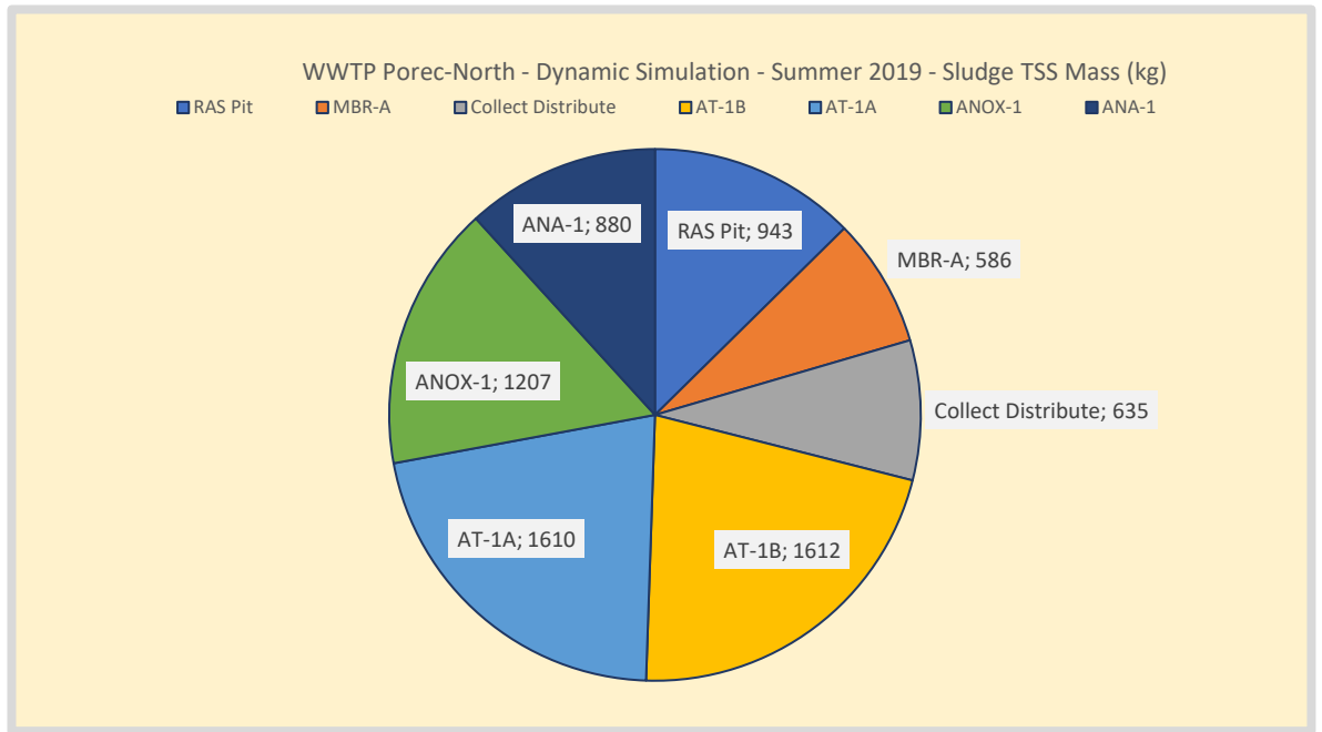
Figure 111. Summer – WWTP Poreč-North sludge mass distribution (kgTSS) in the reactor tanks. Based on these data and the average sludge production, the SRT of the WWTP is calculated. All operated reactors containing activated sludge are included in the SRT calculations.
