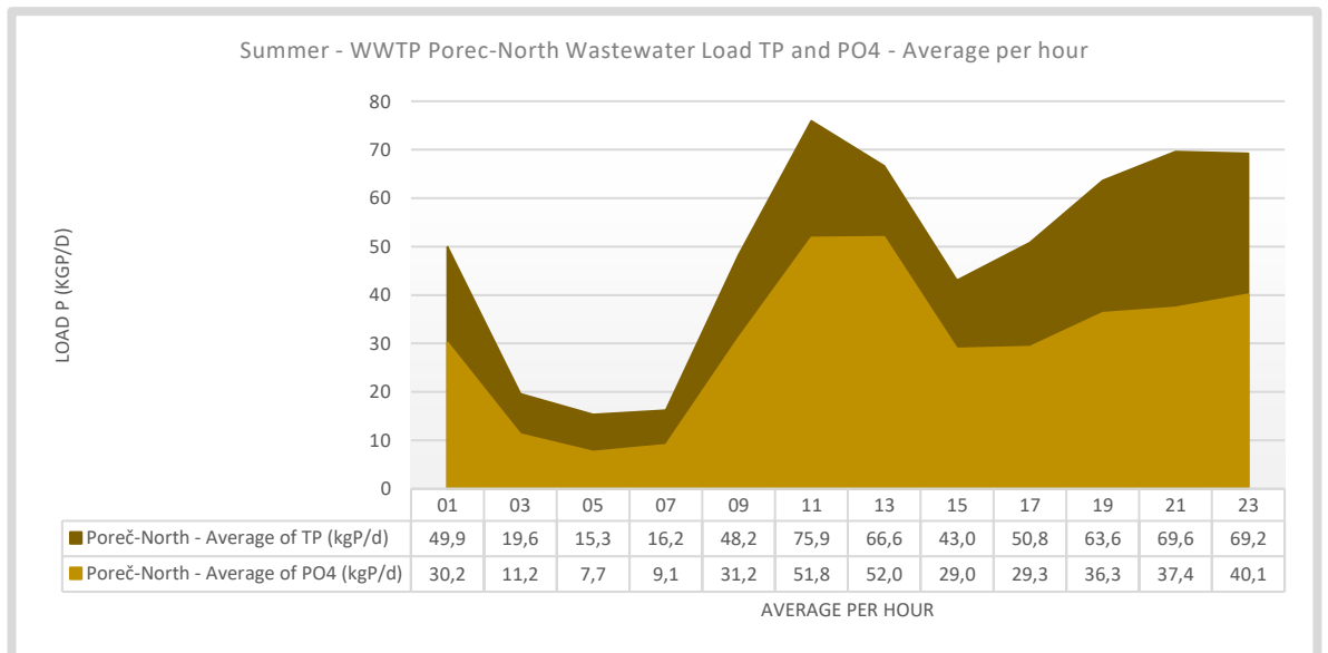
Figure 71. Summer – WWTP Poreč-North hourly average influent loads TP and PO4, based on 7 measurement days. No rain events occurred during the measurement period. This data is used to reconstruct missing data points in 7-day measurement series.
