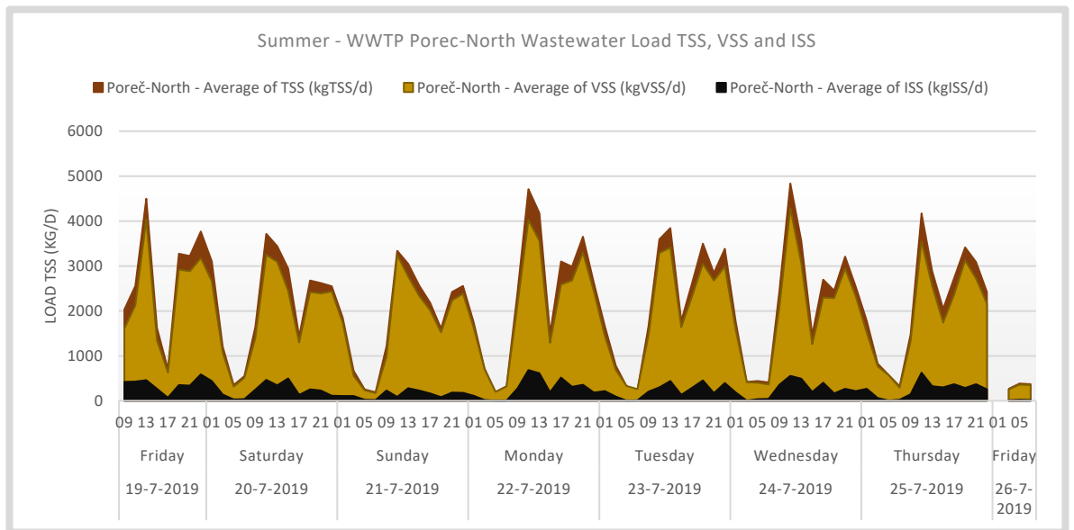
Figure 78. Summer - WWTP Poreč-North Wastewater Loads TSS, VSS and ISS. No rain events occurred during the measurement period. For the model input missing data points are reconstructed based on the hourly average load.
