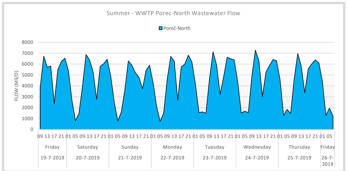
Figure 13. Summer - WWTP Poreč-North Dry Weather Wastewater Flow 24-hour 7-day dynamic measurements. No rain events occurred during the measurements.
