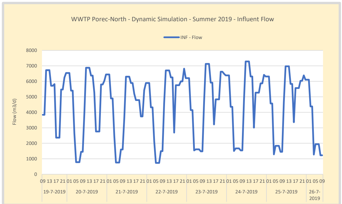
Figure 15. Summer – BioWin modelling WWTP Poreč-North: Wastewater Flow 24-hour 7-day dynamic model input data. In the model data are interpolated on an hourly basis.
