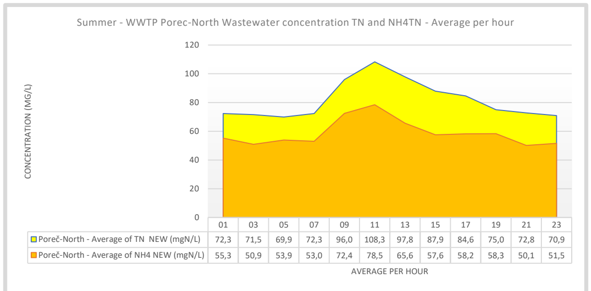
Figure 28. Summer – WWTP Poreč-North 24-hour average TN and NH4 influent Concentration. A typical distribution with peak in the morning. A typical distribution with peak in the morning. Based on the time of the morning peak the estimated sewer HRT is 4 hours.
