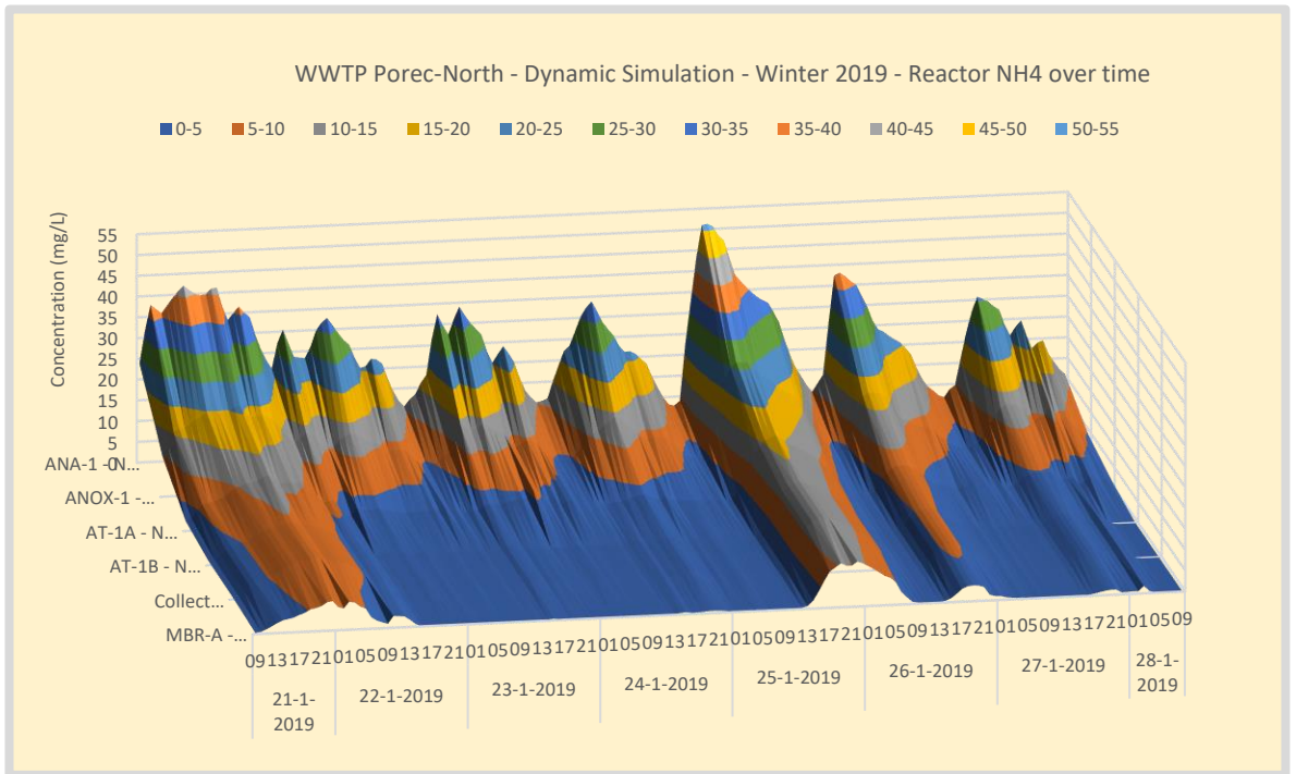
Figure 94. Winter – WWTP Poreč-North NH4 concentration profile over the waterline.
