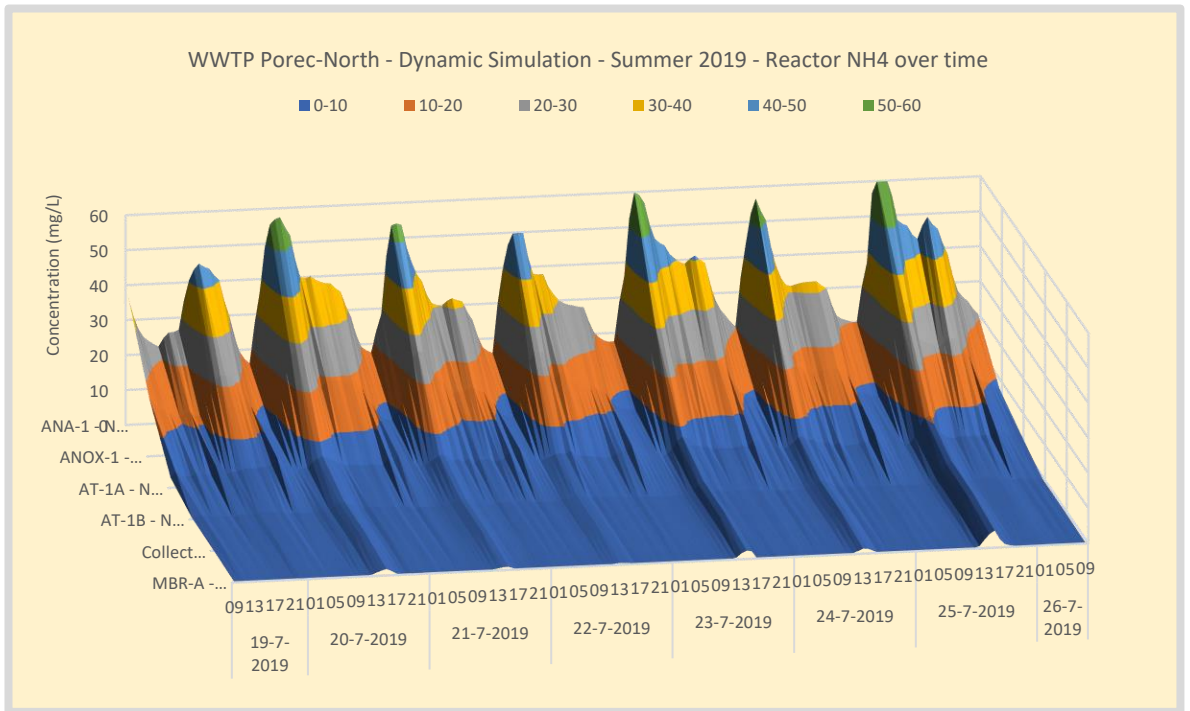
Figure 123. Summer – WWTP Poreč-North NH4 concentration profile over the waterline.
