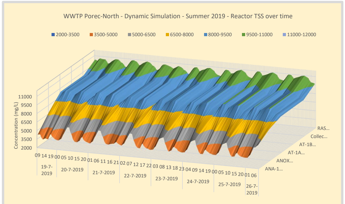
Figure 122. Summer – WWTP Poreč-North TSS concentration profile over the waterline.
