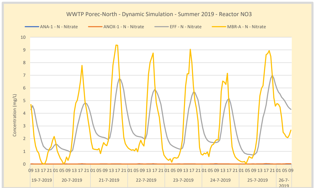
Figure 121. Summer – WWTP Poreč-North nitrate in the anoxic tank. The anoxic recycle rate is controlled on a nitrate setpoint of 2 mgNO 3 /L in the anoxic tank. Internal recycle capacity is not sufficient to reach this setpoint. The concentration of NO 3 in the anoxic tank is almost zero.
