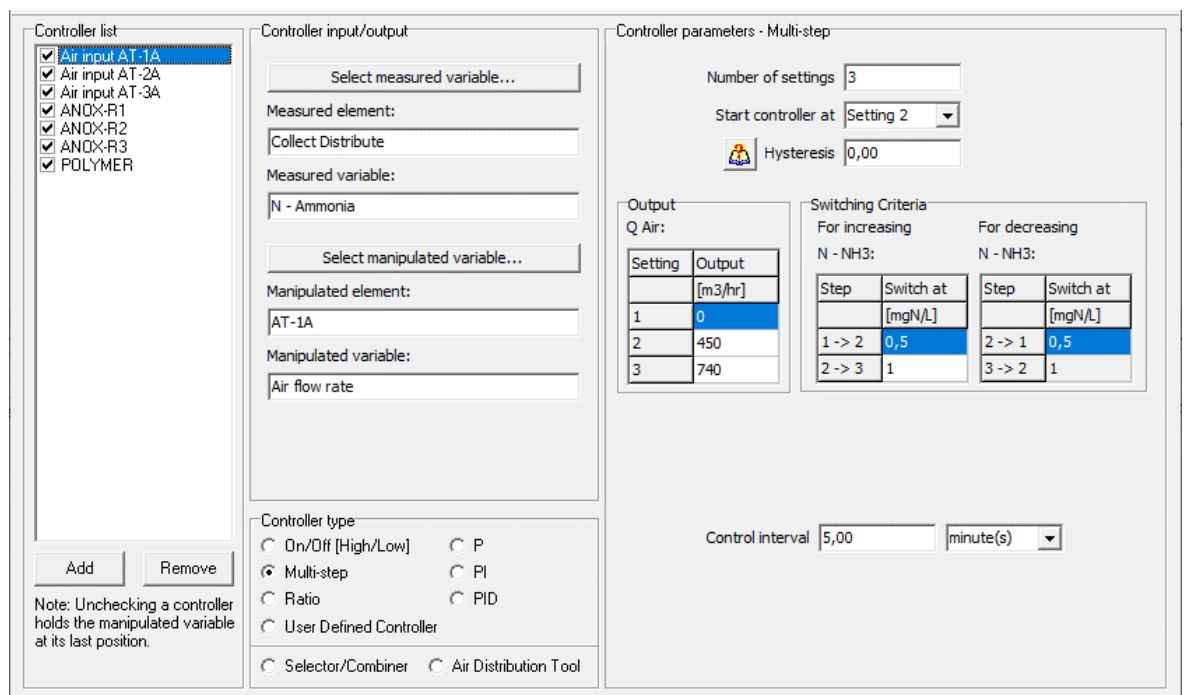
Figure 83. Winter – WWTP Poreč-North BioWin controller toolbox used for controlling the air input of AT-A. The measured variable is NH 4 in the collect distribute tank. The manipulated variable the air flow in AT-A. There are 3 settings for the air flow depending on the NH 4 concentration.
