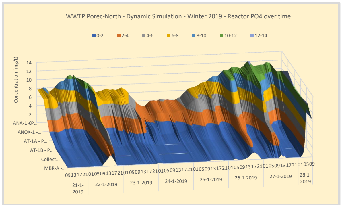
Figure 96. Winter – WWTP Poreč-North PO4 concentration profile over the waterline.
