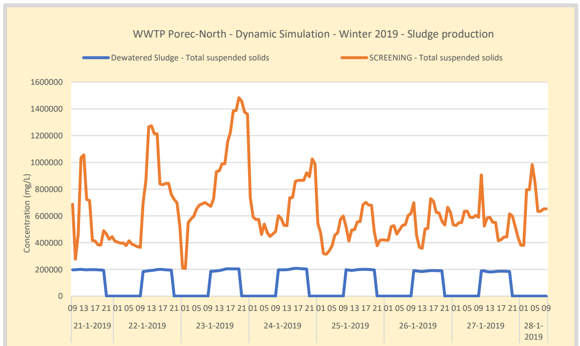
Figure 103. Winter – WWTP Poreč-North dewatered sludge and screening sludge concentration. The design assumes dewatered sludge at 23% dry matter. Screening is an estimated concentration as the result of the press operation.
