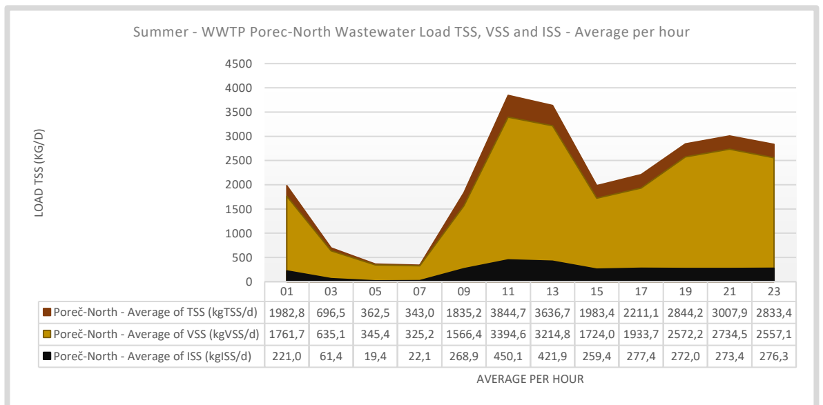
Figure 79. Summer – WWTP Poreč-North hourly average influent loads TSS, VSS and ISS, based on 7 measurement days. No rain events occurred during the measurement period. This data is used to reconstruct missing data points in 7-day measurement series. TSS and ISS are both exceptionally high. ISS could be sand ending up in the sewer.
