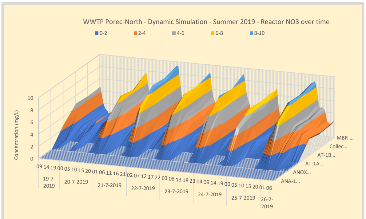
Figure 124. Summer – WWTP Poreč-North NO3 concentration profile over the waterline.
