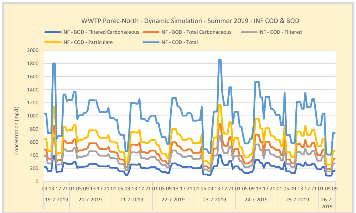
Figure 23. Dynamic Simulation – WWTP Poreč-North – Summer 24-hour average COD, COD micro-filtered, COD particulate, BOD and BOD filtered influent Concentration. The model input is the measured and reconstructed COD concentration. The other lines are calculated based on (constant) fractions determined in the influent specification. No rain occurred. Peaks are measured 19-7, 23-7 and 24-7 indicating nondomestic discharge.
