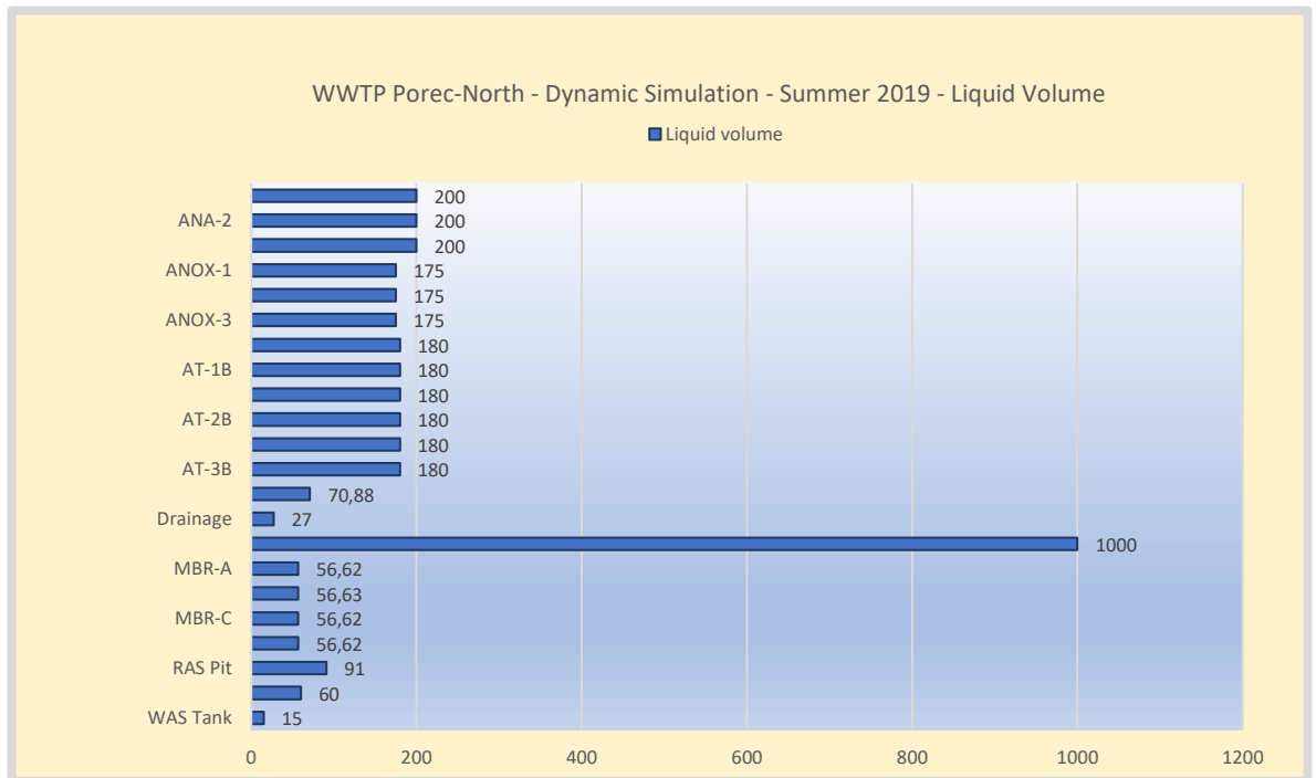
Figure 110. WWTP Poreč-North – Volume distribution of modelled reactor elements. The actual WAS tank is 150 m3 however the sludge volume is modelled based on an HRT less than 2,5 hours to avoid P-release. The WAS tank is not suitable for sludge storage.
