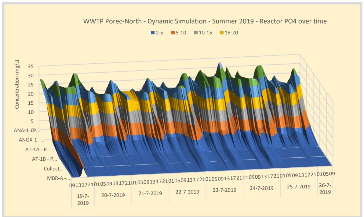
Figure 125. Summer – WWTP Poreč-North PO4 concentration profile over the waterline.
