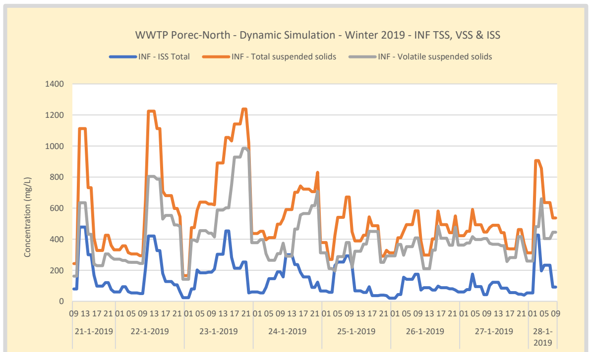
Figure 38. Dynamic Simulation – WWTP Poreč-North – Winter 24-hour average TSS, VSS (organic particulate) and ISS (inorganic particulate) influent Concentration. The model input is the measured and reconstructed ISS concentration. VSS is calculated based on (constant) fractions determined in the influent specification. TSS is modelled as the sum of ISS and VSS. 28-01-2019 a major rain event occurred causing an increase in the TSS concentration. TSS peaks 22-1 and 23-1 coinciding with other parameters indicating a nondomestic discharge.
