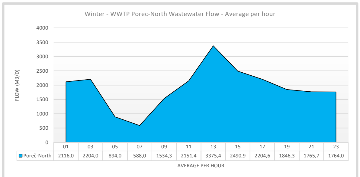
Figure 7. Winter - WWTP Poreč-North Dry Weather Wastewater Flow 24-hour average hourly measurements. These data are used to reconstruct missing datapoints in the 7-day 24-hours measurements and can be used for scenario calculations.
