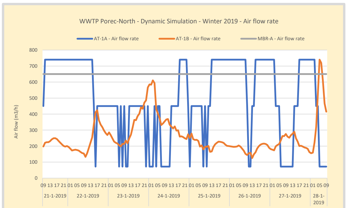
Figure 97. Winter – WWTP Poreč-North air input in the different aerated reactors. AT-A is step controlled on NH4, AT-B is setpoint controlled on the DO, the MBR is fully aerated according to the design value.
