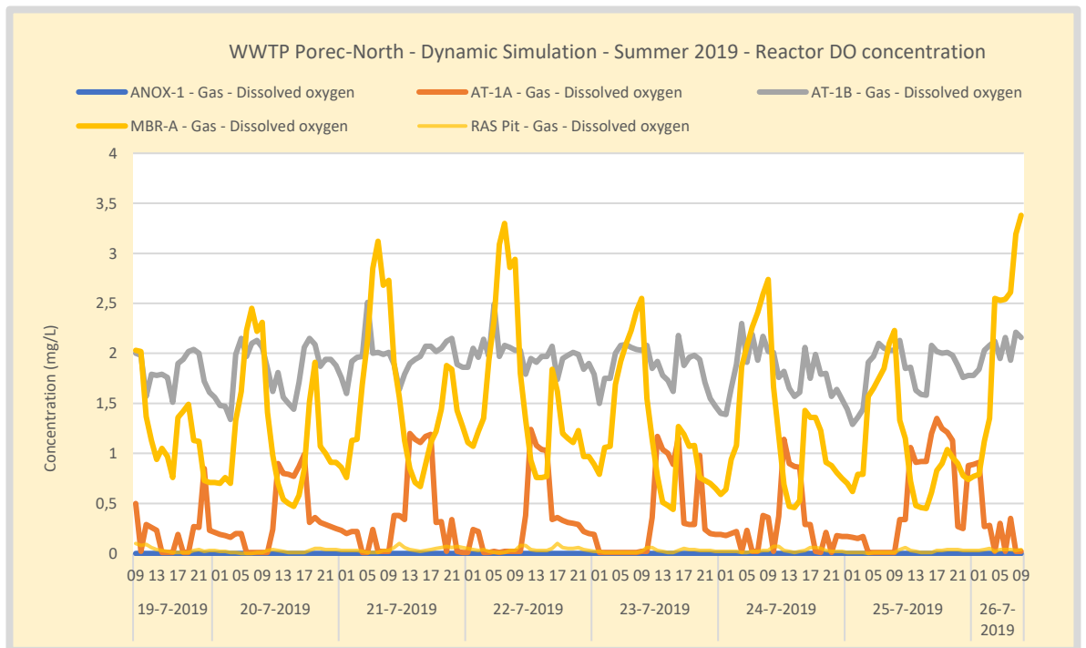
Figure 127. Summer – WWTP Poreč-North DO concentration gradients. DO is controlled in the AT-B on 2 mgO 2 /L and the air flow of AT-B on NH 4 concentration in the outflow of the aeration. In the MBR the DO is the result of the designed maximum air input. Little oxygen is recycled over the reactors and little oxygen is measured in the anoxic zone. The DO setpoint can be maintained based on the designed air flow.
