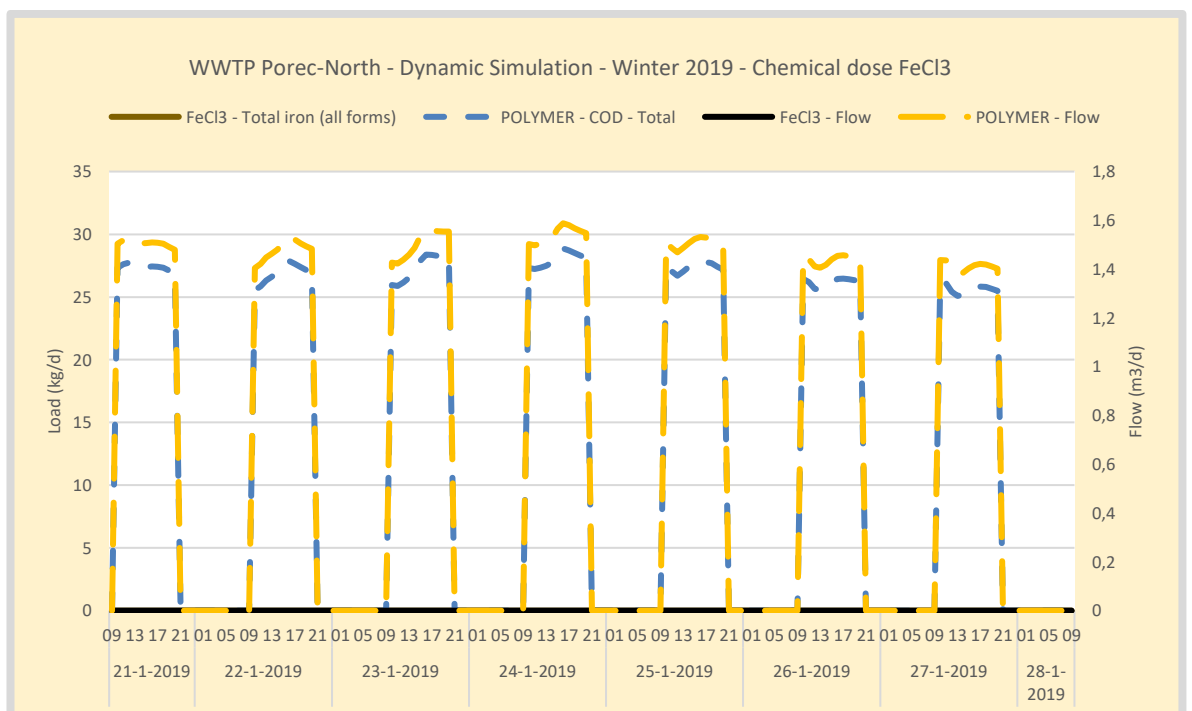
Figure 101. Winter – WWTP Poreč-North load and flow of Iron and PE. No Iron dosage is required for P-removal. PE is assumed particulate biodegradable COD with a COD/VSS ratio of 1,42 gCOD/gTSS and dosed proportional to the WAS load based on 8 kg PE (dry weight) dosed per 1000 kg WAS (dry weight) flowing in the dewatering.
