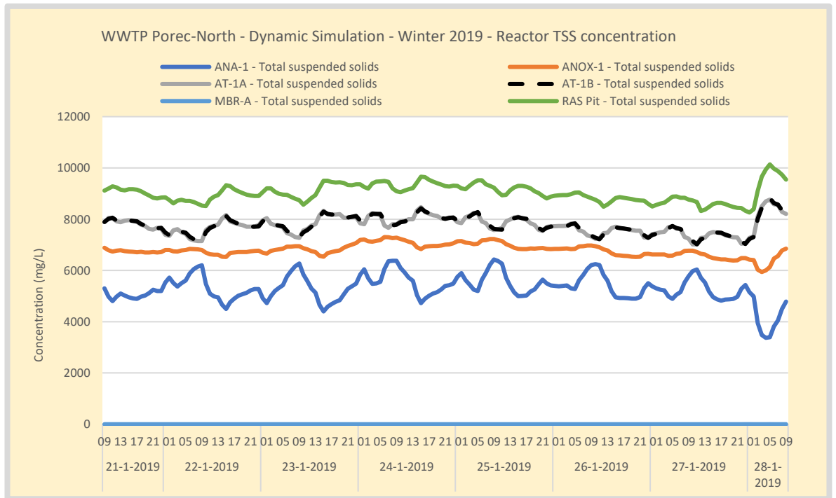
Figure 90. Winter – WWTP Poreč-North TSS profile in the waterline. TSS in the MBR is controlled on 9 gTSS/L.
