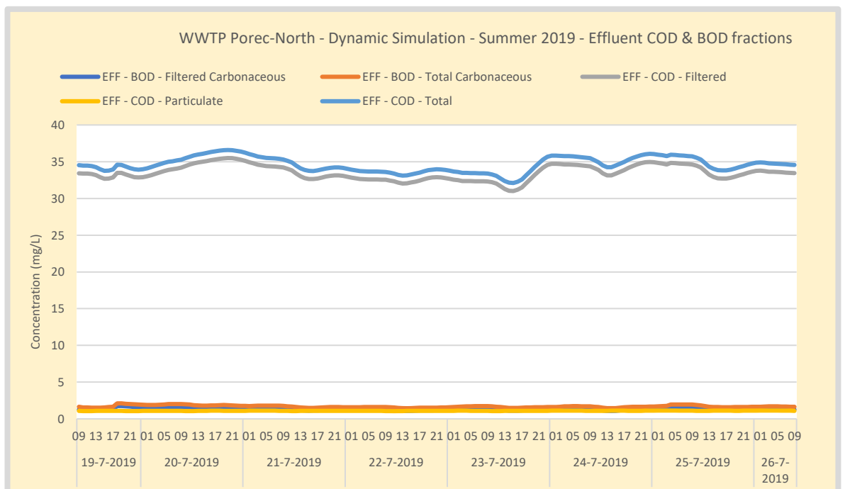
Figure 138. Summer – WWTP Poreč-North Effluent COD and BOD concentration. The Particulate fraction is the result of a MBR efficiency of 99,9% for particulate and 99,99% for colloidal material. Effluent is measured in the outflow of the large effluent buffer.
