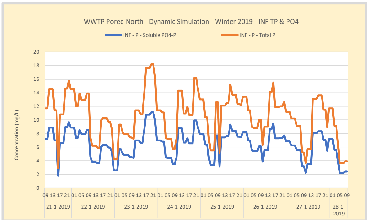
Figure 32. Dynamic Simulation – WWTP Poreč-North – Winter 24-hour average TP and PO4 influent Concentration. The model input is the measured and reconstructed TP concentration. PO4 is calculated based on a (constant) fraction determined in the influent specification. 28-01-2019 a major rain event occurred. No exceptional peaks occur.
