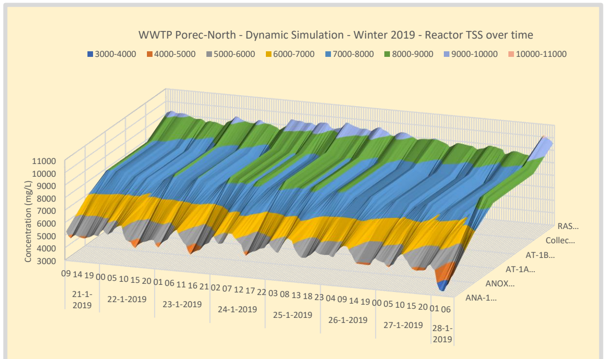
Figure 93. Winter – WWTP Poreč-North TSS concentration profile over the waterline.
