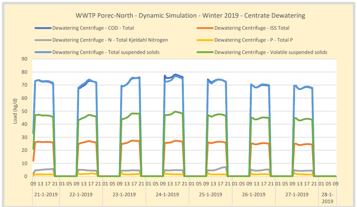
Figure 104. Winter – WWTP Poreč-North Centrate load dewatering.
