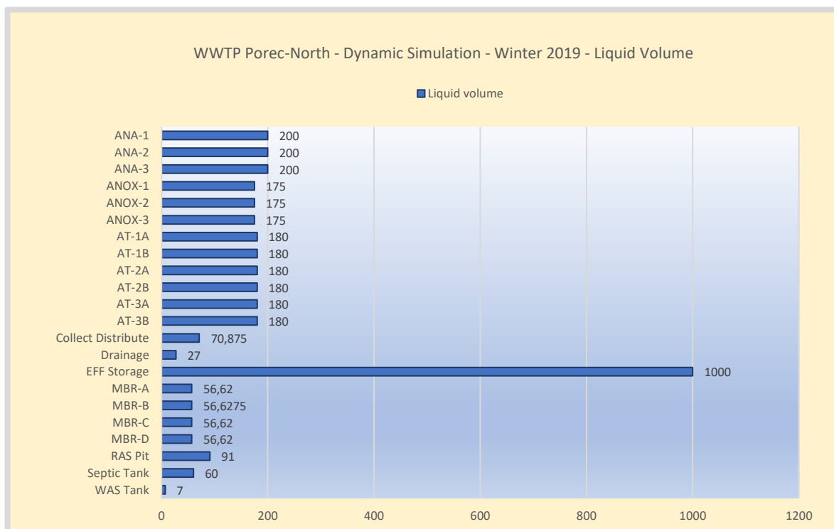
Figure 81. WWTP Poreč-North – Volume distribution of modelled reactor elements. The actual WAS tank is 150 m3 however the sludge volume is modelled based on an HRT less than 2,5 hours to avoid P-release. The WAS tank is not suitable for sludge storage.
