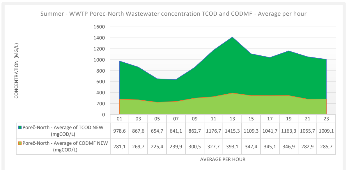
Figure 22. Summer – WWTP Poreč-North 24-hour average COD and COD micro-filtered influent Concentration. While soluble COD is relative constant the total which also contains the particulate is more distributed towards the first flow peak of the day.
