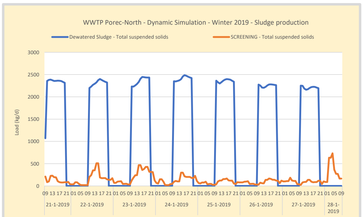
Figure 105. Winter – WWTP Poreč-North dewatered sludge load and compacted screening load. Dewatered sludge is operated 10 hours a day at 23%. Screening is produces continuously as a factor of the influent.
