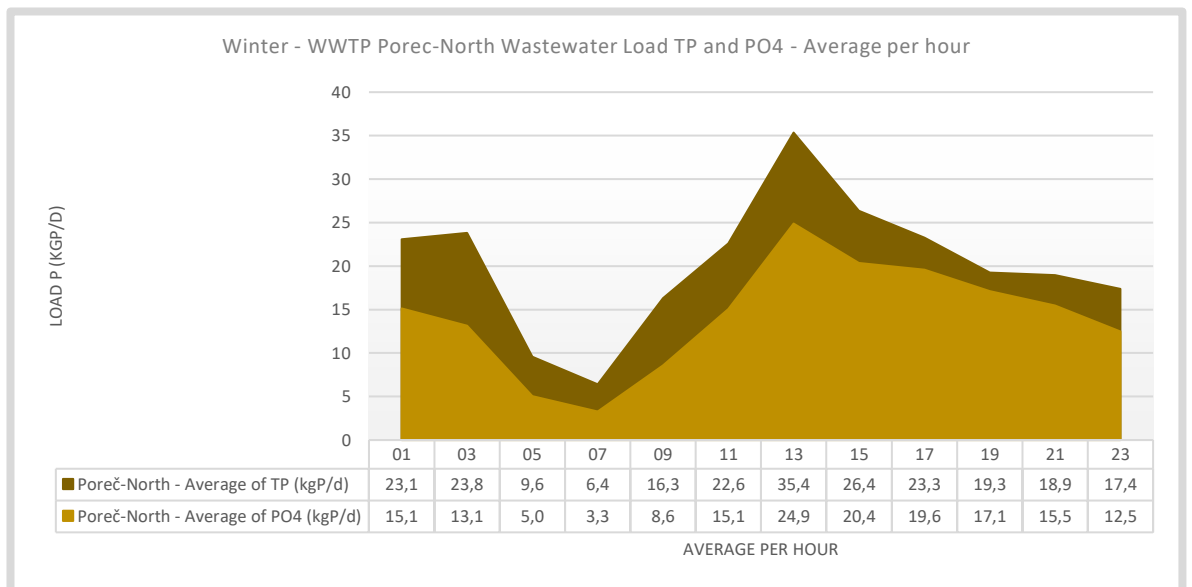
Figure 67. Winter – WWTP Poreč-North hourly average influent loads TP and PO4, based on 7 measurement days, excluding the rain event Monday 28-01-2019. This data is used to reconstruct missing data points in 7-day measurement series.
