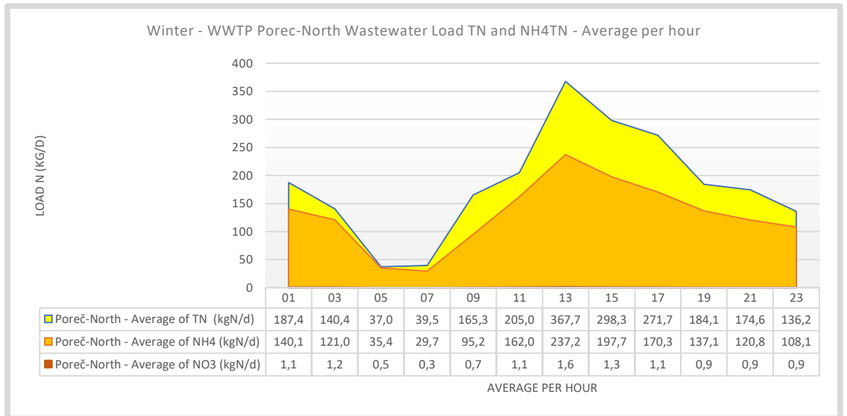
Figure 59. Winter – WWTP Poreč-North hourly average dry weather influent loads TN, NH4 and NO3, based on 7 measurement days, excluding the rain event Monday 28-01-2019. This data is used to reconstruct missing data points in 7-day measurement series.
