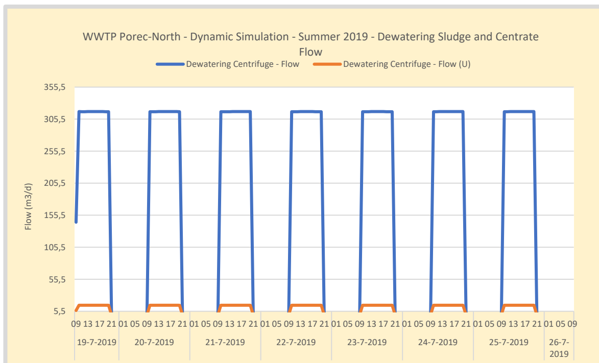
Figure 131. Summer – WWTP Poreč-North dewatered sludge and centrate flow.
