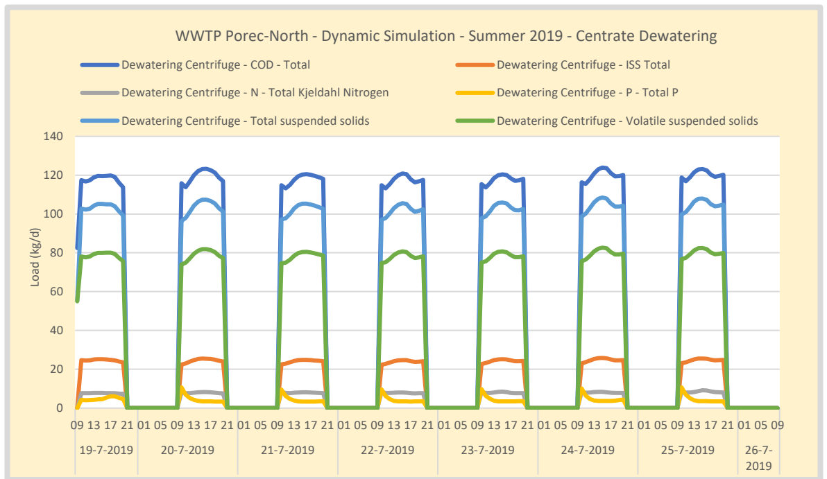
Figure 133. Summer – WWTP Poreč-North Centrate load dewatering.
