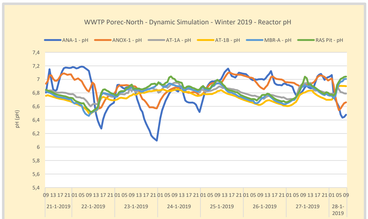
Figure 99. Winter – WWTP Poreč-North pH profile over the activated sludge reactors. Influent pH is measured continuously and is not limiting. pH is not limiting.
