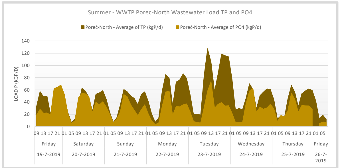
Figure 70. Summer - WWTP Poreč-North Wastewater Loads TP and PO4. No rain events occurred during the measurement period. For the model input missing data points are reconstructed based on the hourly average dry weather load. 23-7 there is a considerable peak loading.
