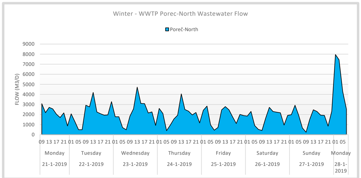
Figure 6. Winter - WWTP Poreč-North Wastewater Flow 24-hour 7-day dynamic measurements. This data is used for dynamic modelling.
