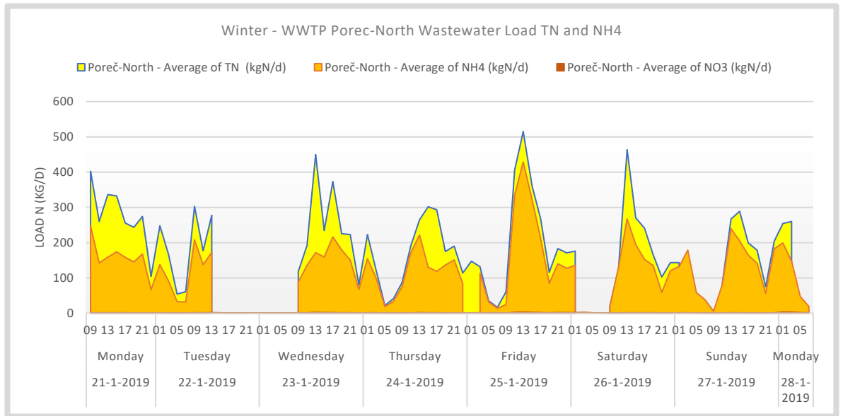
Figure 58. Winter – WWTP Poreč-North Influent TN, NH4 and NO3 Loads based on 7 measurement days. A rain event occurred Monday 28-01-2019. For the model input missing data (22, 23, 25, 26-1) points are reconstructed based on the hourly average dry weather load.
