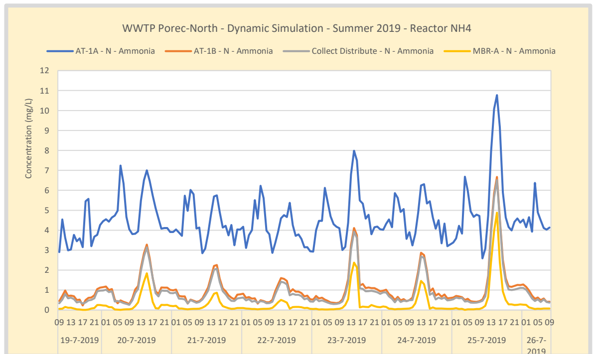
Figure 120. Summer – WWTP Poreč-North ammonium profile in the waterline. The air input of AT-A is controlled based on \text{NH}_4 measured in the collect distribute tank using a 3-step controller. Above 1,0 \text{mgNH}_4/\text{L} the air input goes to its maximum value. Below 0,5 air shuts off. AT-B is DO controlled on 2,0 \text{mgO}_2/\text{L} .
