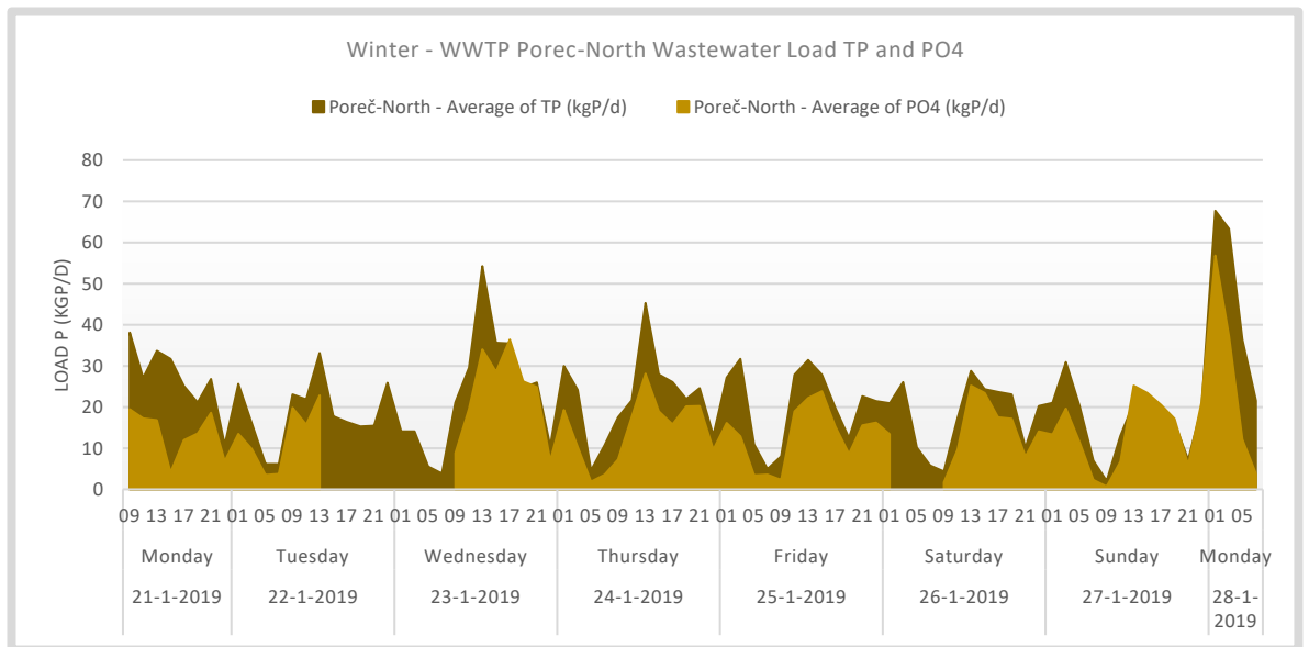
Figure 66. Winter – WWTP Poreč-North Influent TP and PO4 Loads based on 7 measurement days. A rain event occurred Monday 28-01-2019. For the model input missing data points are reconstructed based on the hourly average dry weather load.
