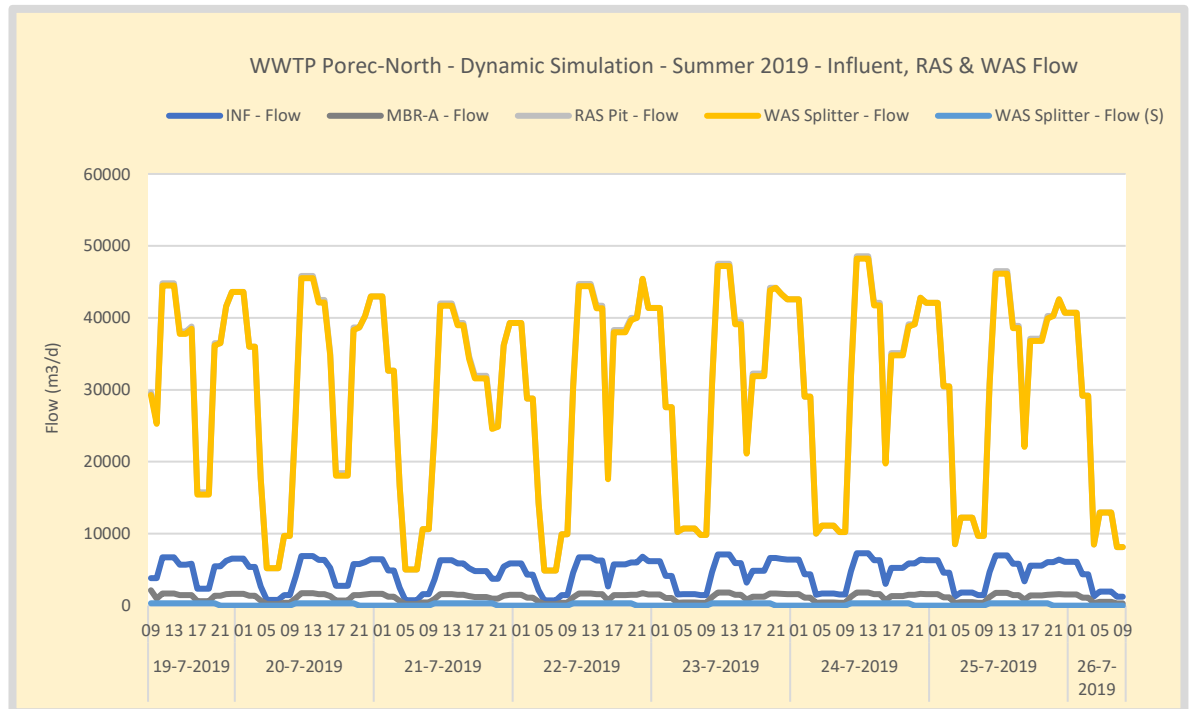
Figure 117. Summer – WWTP Poreč-North flow rate settings and control. The MLSS sludge return flow is controlled proportional to the influent. The WAS flow is time controlled and operated 10 hours a day on a constant flow.
