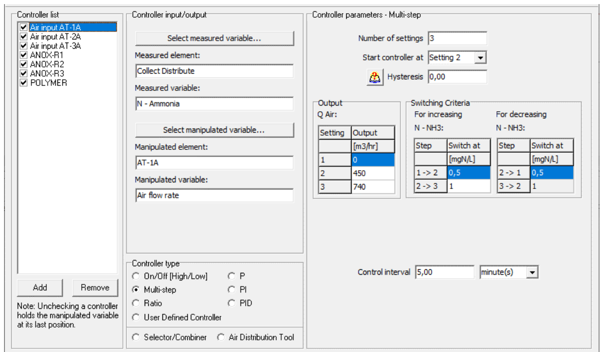
Figure 112. Summer – WWTP Poreč-North BioWin controller toolbox used for controlling the air input of AT-A. The measured variable is NH 4 in the collect distribute tank. The manipulated variable the air flow in AT-A. There are 3 settings for the air flow depending on the NH 4 concentration.
