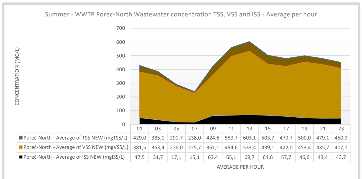
Figure 40. Summer – WWTP Poreč-North 24-hour average TSS, VSS and ISS influent Concentration.
