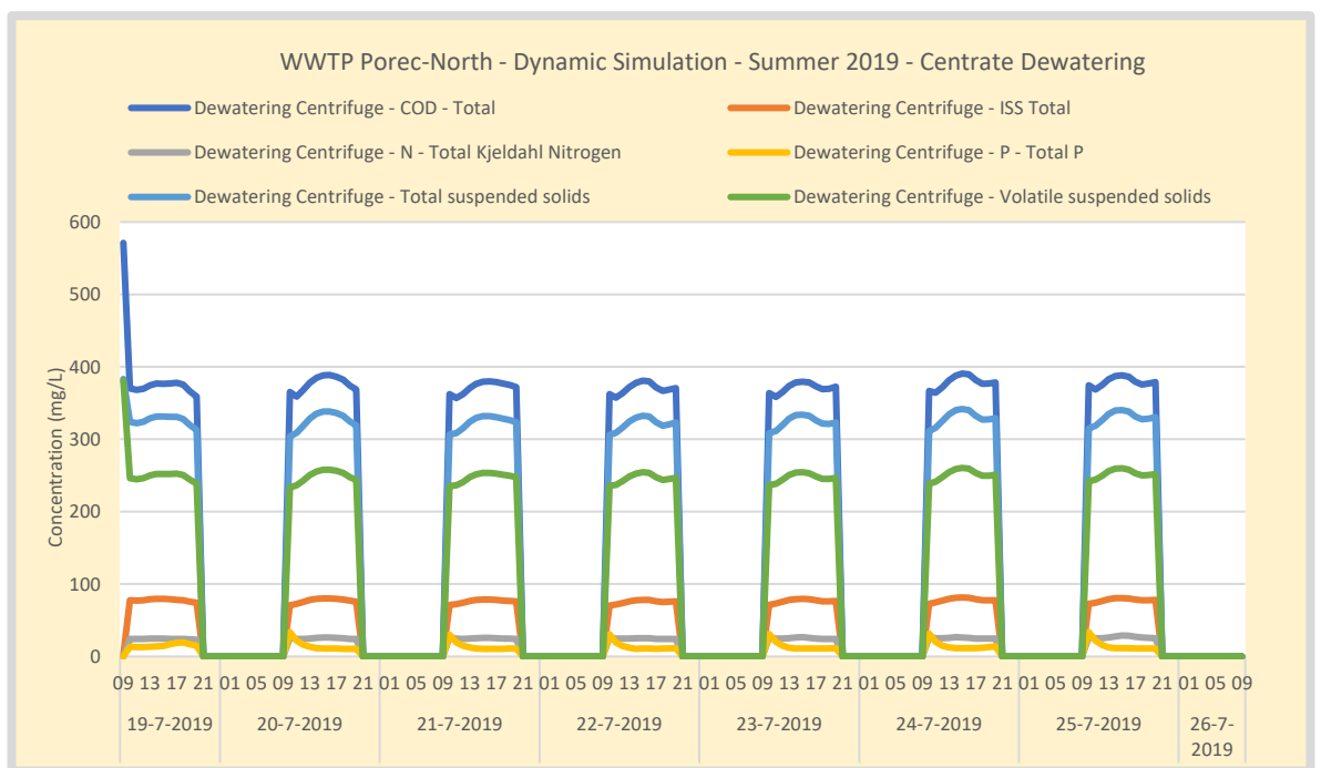
Figure 134. Summer – WWTP Poreč-North Centrate concentrations dewatering.
