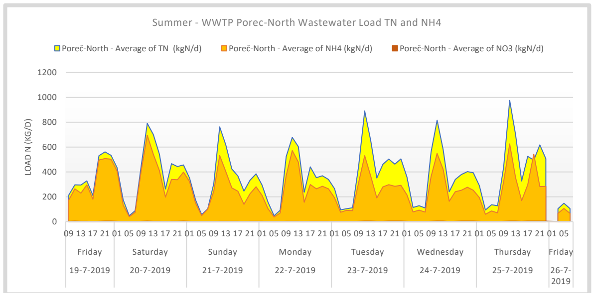
Figure 62. Summer - WWTP Poreč-North Wastewater Load TN, NH4 and NO3. No rain events occurred during the measurement period. For the model input missing data points (26-7) are reconstructed based on the hourly average dry weather load.
