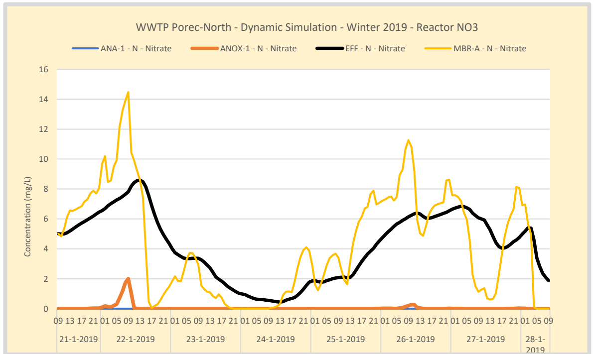
Figure 92. Winter – WWTP Poreč-North nitrate in the anoxic tank. The anoxic recycle rate is controlled on a nitrate setpoint of 2 mgNO 3 /L in the anoxic tank. The internal anoxic recycle is not sufficient to maintain that optimal condition. This indicates or the anoxic tank is too large or anoxic recycle too little. The effluent storage has a strong buffer effect and reduces nitrate peaks in the effluent.
