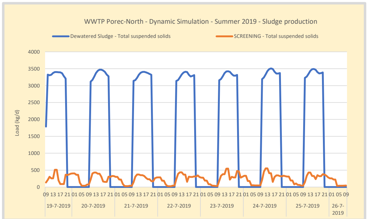
Figure 135. Summer – WWTP Poreč-North dewatered sludge load and compacted screening load. Dewatered sludge is operated 10 hours a day at 23%. Screening is produces continuously as a factor of the influent.
