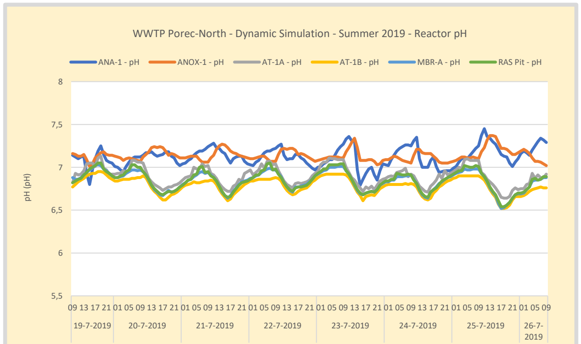
Figure 128. Summer – WWTP Poreč-North pH profile over the activated sludge reactors. Influent pH is measured continuously and is not limiting. pH is not limiting.
