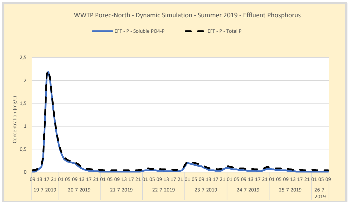
Figure 137. Summer – WWTP Poreč-North Effluent phosphorus concentration. No Iron dose is dosed. Effluent is measured in the outflow of the large effluent buffer.
