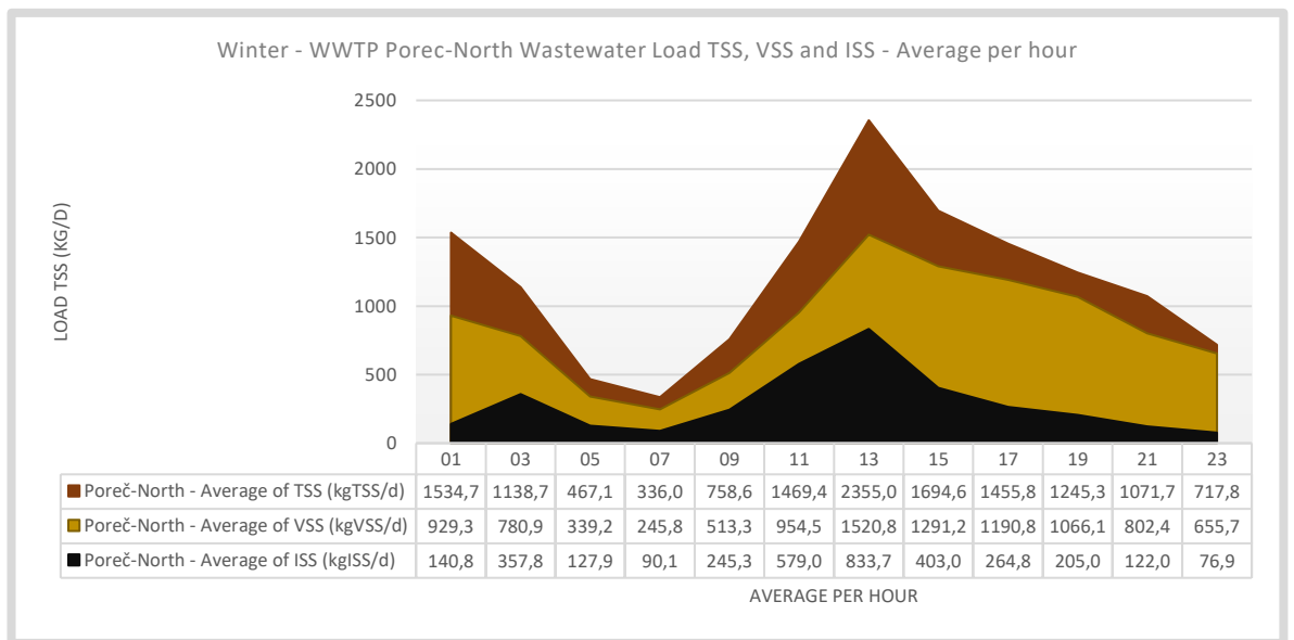
Figure 75. Winter – WWTP Poreč-North hourly average influent loads TSS, VSS and ISS, based on 7 measurement days, excluding the rain event Monday 28-01-2019. This data is used to reconstruct missing data points in 7-day measurement series. TSS and ISS are both exceptionally high. ISS could be sand ending up in the sewer.
