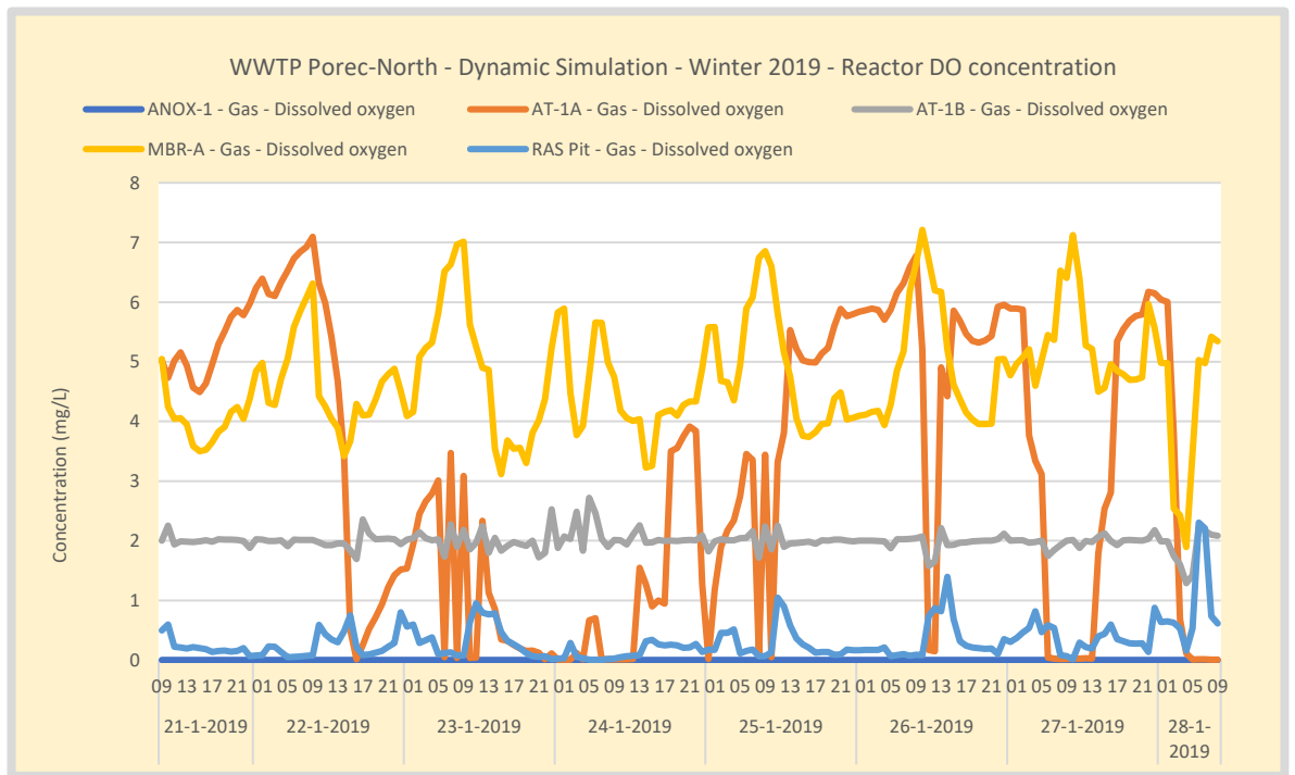
Figure 98. Winter – WWTP Poreč-North DO concentration gradients. DO is controlled in the AT. There is a maximum airflow in the MBR. Oxygen is recycled over the reactors causing accumulation of DO in the AT during periods of low influent loading.
