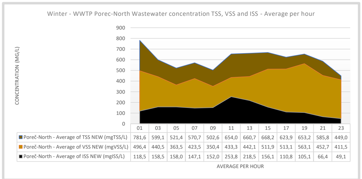
Figure 37. Winter – WWTP Poreč-North 24-hour average TSS, VSS and ISS influent Concentration.
