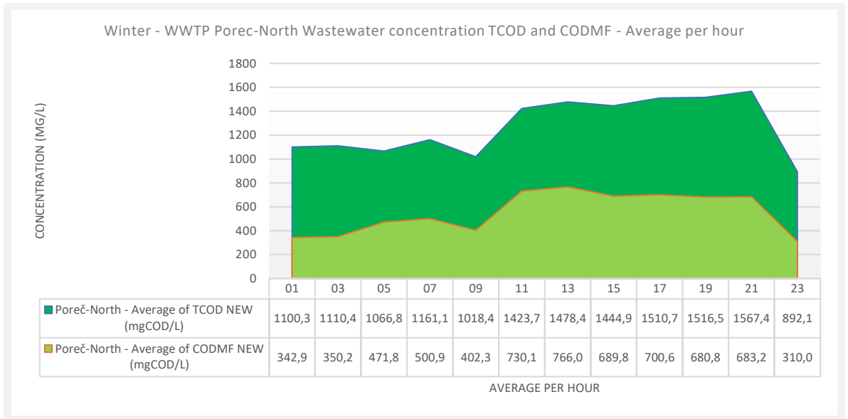
Figure 19. Winter – WWTP Poreč-North 24-hour average COD and COD micro-filtered influent Concentration. In average the wastewater of Poreč-North is more concentrated.
