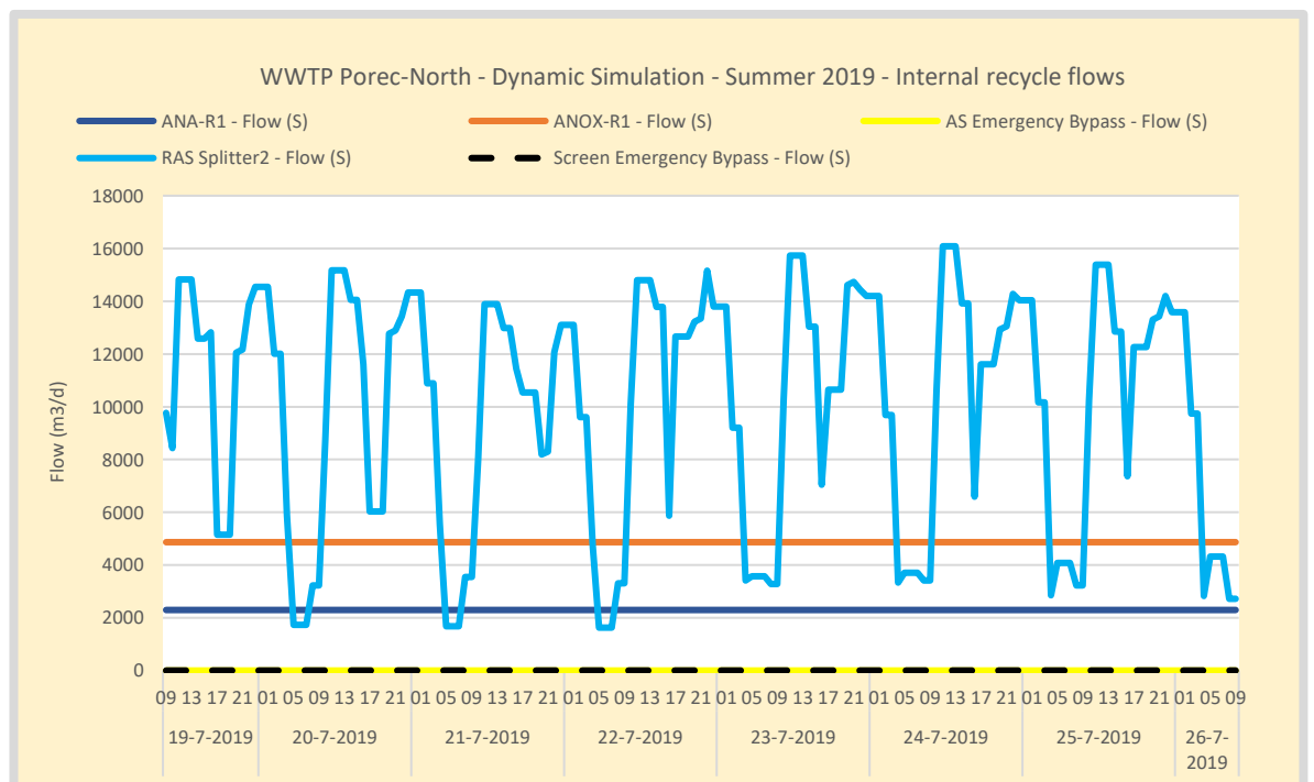
Figure 118. Summer – WWTP Poreč-North flow rate settings and control. The bypasses are not used. The anoxic recycle is constant at its maximum value. The anoxic recycle is reduced the moment Nitrate starts to accumulate in the anoxic tank (which does not occur).
