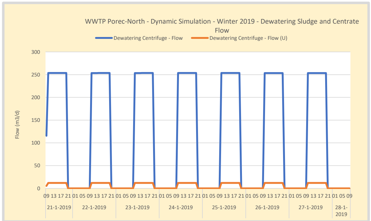
Figure 102. Winter – WWTP Poreč-North dewatered sludge and centrate flow.
