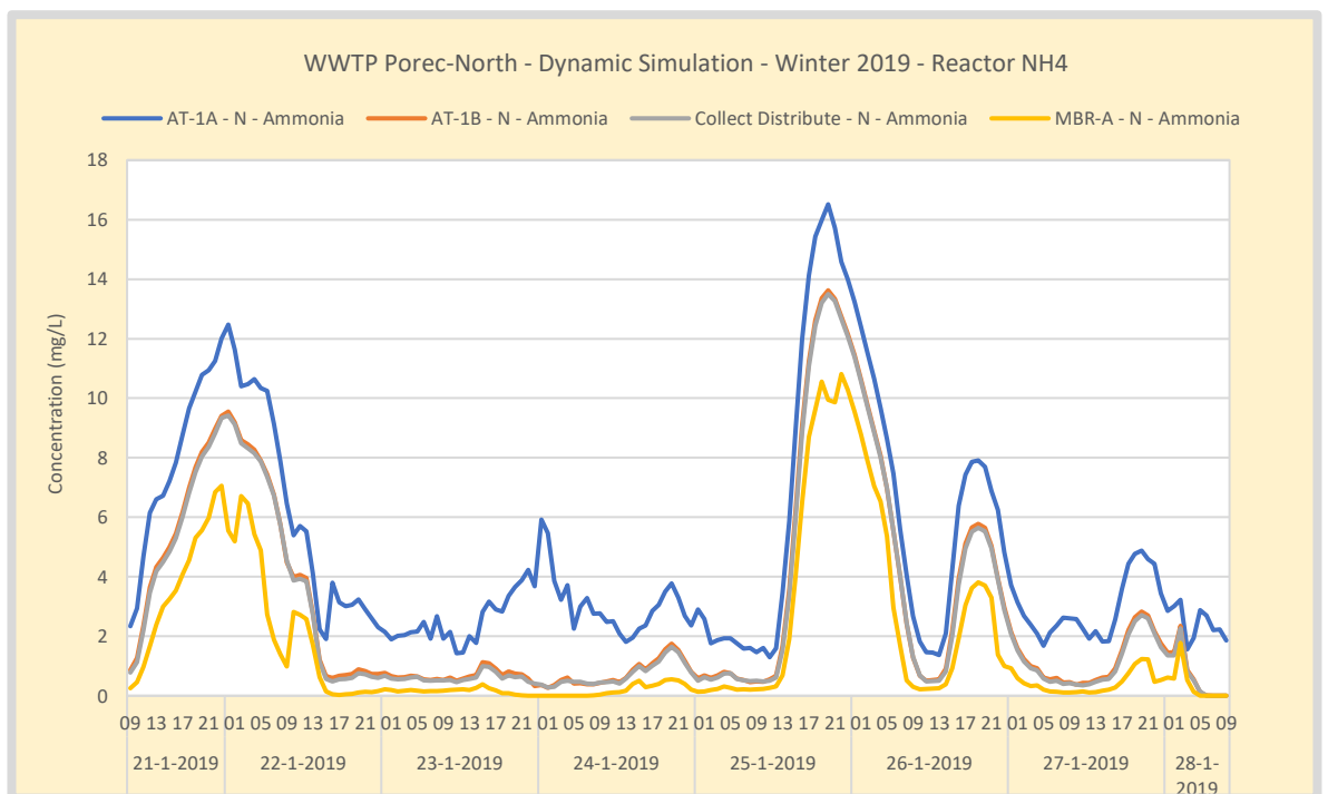
Figure 91. Winter – WWTP Poreč-North ammonium profile in the waterline. The air input of AT-A is controlled based on \text{NH}_4 measured in the collect distribute tank using a 3-step controller. Above 1,0 \text{ mgNH}_4/\text{L} the air input goes to its maximum value. Below 0,5 air shuts off. AT-B is DO controlled on 2,0 \text{ mgO}_2/\text{L} .
