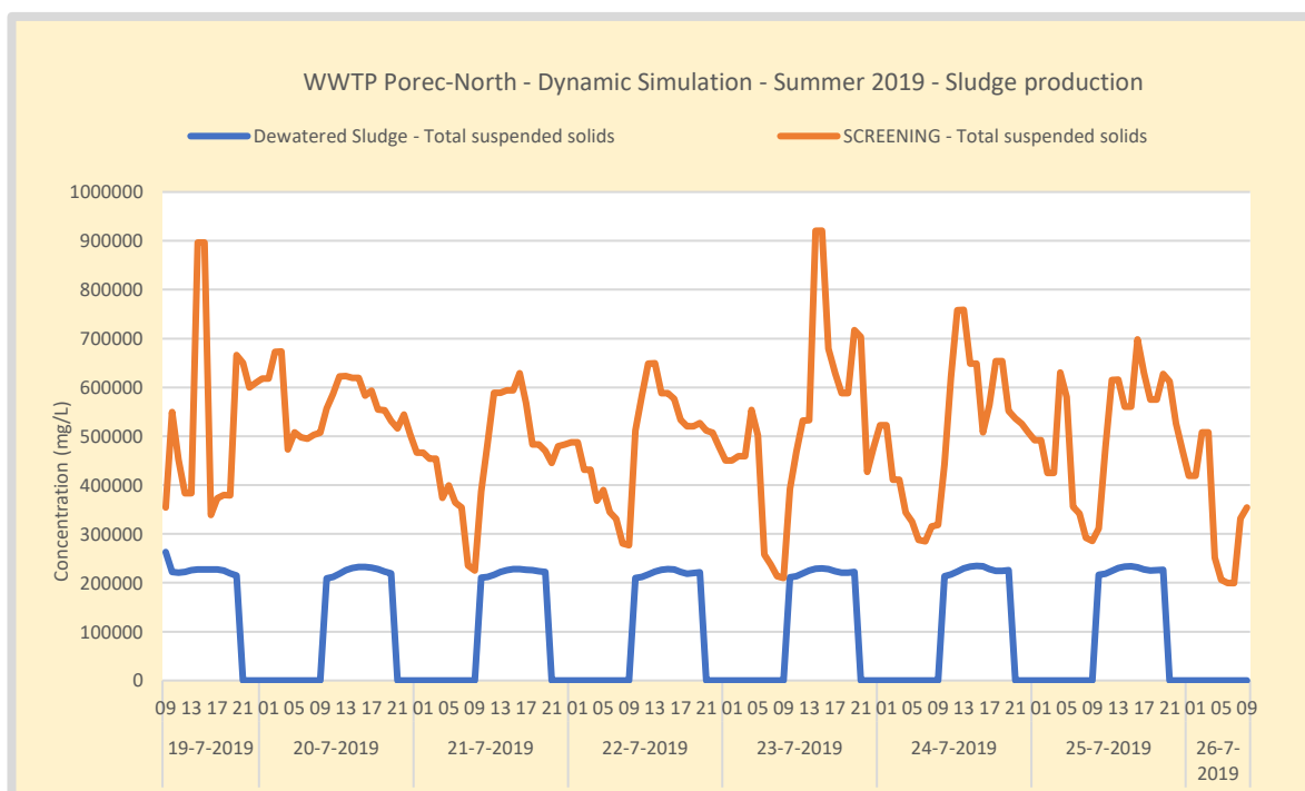
Figure 132. Summer – WWTP Poreč-North dewatered sludge and screening sludge concentration. The design assumes dewatered sludge at 23% dry matter. Screening is an estimated concentration as the result of the press operation.
