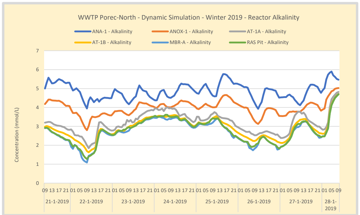
Figure 100. Winter – WWTP Poreč-North alkalinity profile over the activated sludge reactors. Influent alkalinity is estimated from local drinking water quality measurements at 7,46 mmol/L. Potentially there is a limitation of alkalinity in the winter due to CO 2 stripping caused by over aeration.
