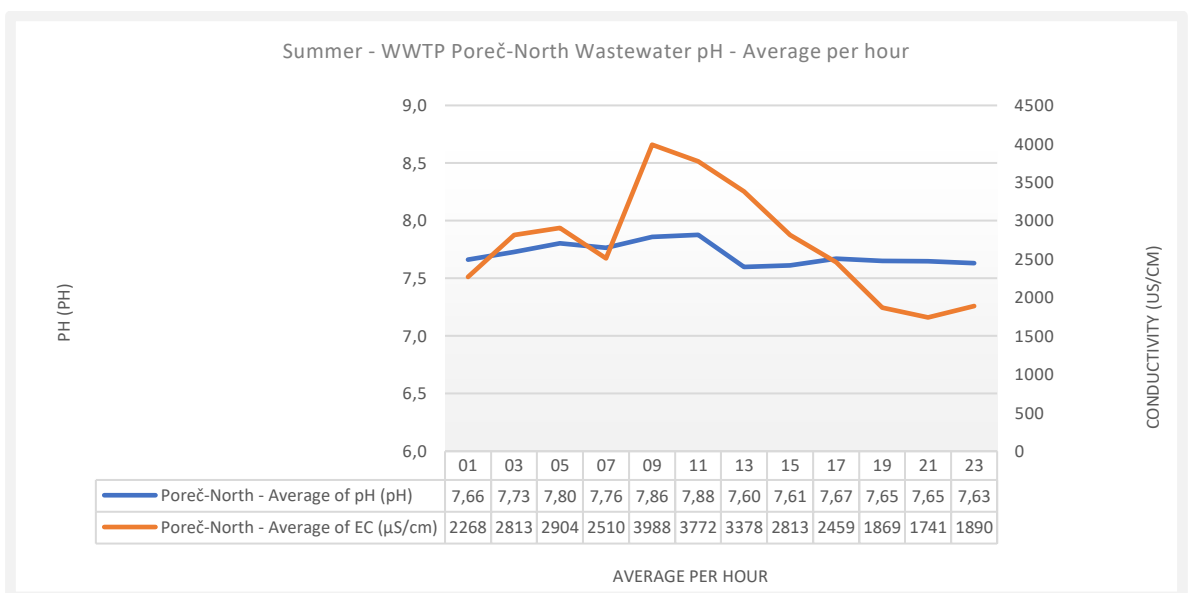
Figure 44. Summer – WWTP Poreč-North 24-hour average pH and conductivity influent measurement.
