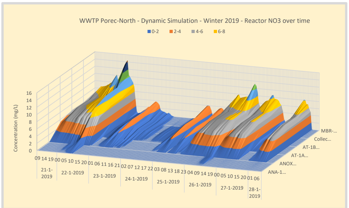
Figure 95. Winter – WWTP Poreč-North NO3 concentration profile over the waterline.
