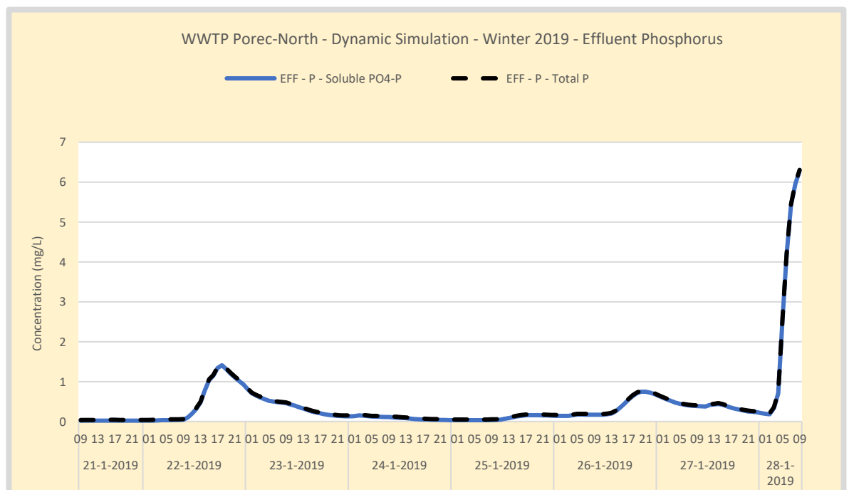
Figure 107. Winter – WWTP Poreč-North Effluent phosphorus concentration. Effluent is measured in the outflow of the large effluent buffer. The last day is a major rain event negatively effecting effluent PO4. The plant is operated without Iron dosage control.
