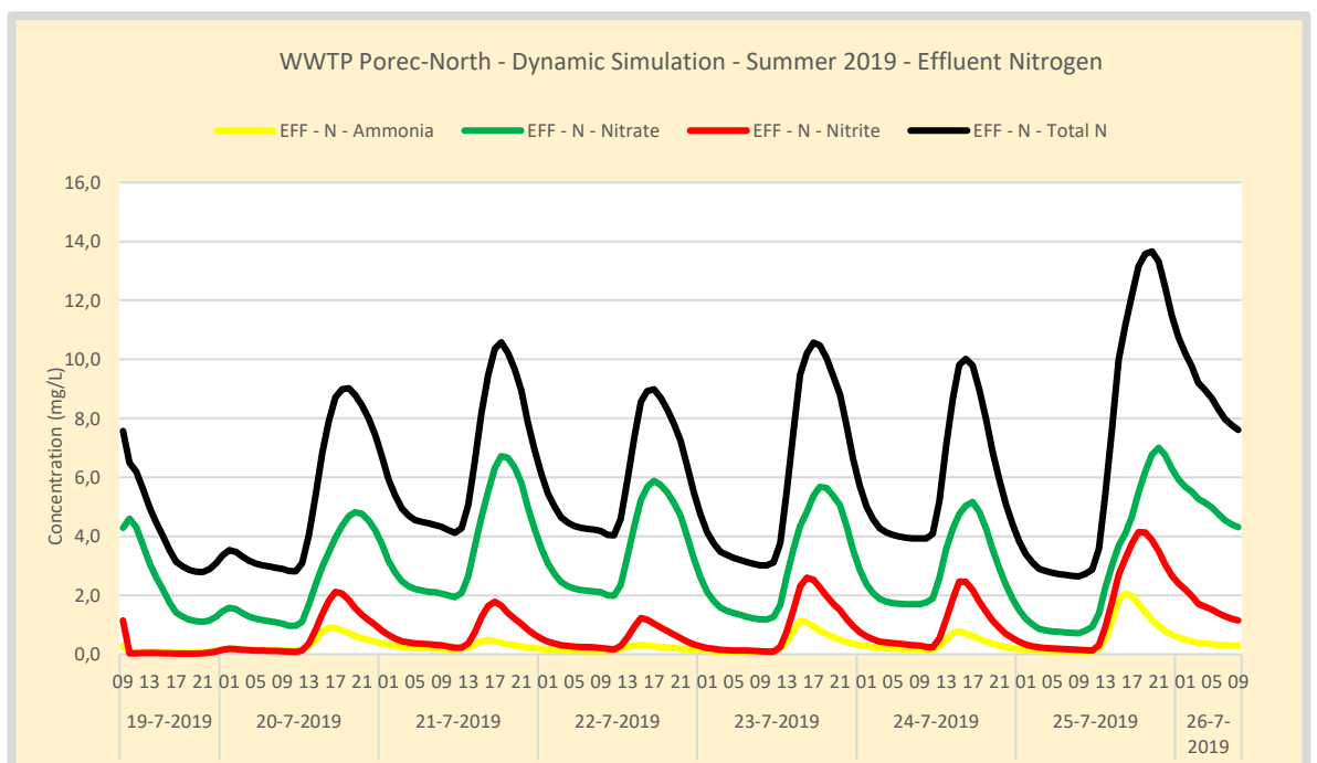
Figure 136. Summer – WWTP Poreč-North Effluent nitrogen concentration. Effluent is measured in the outflow of the large effluent buffer. Nitrite production is low and aeration capacity sufficient.
