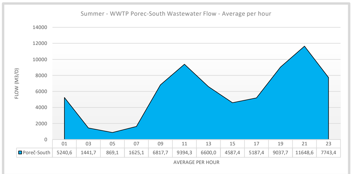
Figure 14. Summer - WWTP Poreč-South Wastewater Flow 24-hour average hourly measurements. Data are used to reconstruct missing data in the flow measurements and for development of scenarios.
