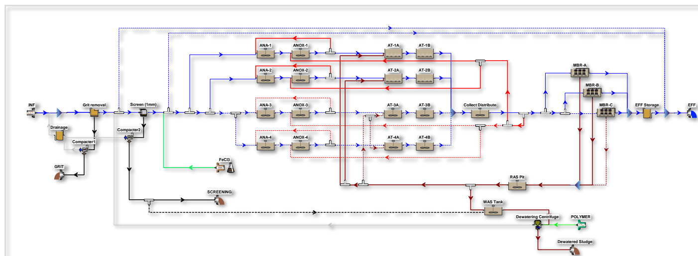
Figure 80. WWTP Poreč-South - BioWin model winter operation. Two lines and one MBR are taken out of operation (dashed lines not operated). Operational adjustments are made to accommodate dynamic modelling. MBR-C is taken out of operation to avoid stripping of alkalinity.
