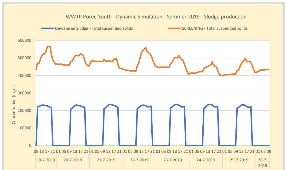
Figure 133. Summer – WWTP Poreč-South dewatered sludge and screening sludge concentration. The design assumes dewatered sludge at 23% dry matter. Screening is an estimated concentration as the result of the press operation.
