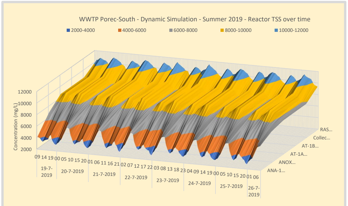
Figure 123. Summer – WWTP Poreč-South TSS concentration profile over the waterline.
