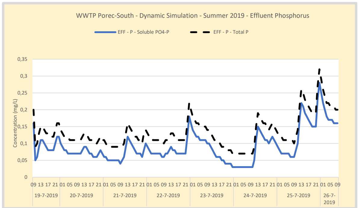
Figure 138. Summer – WWTP Poreč-South Effluent phosphorus concentration. No iron is dosed. Effluent is measured in the outflow of the large effluent buffer.
