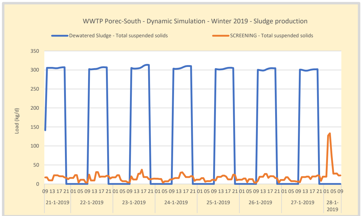
Figure 106. Winter – WWTP Poreč-South dewatered sludge load and compacted screening load. Dewatered sludge is operated 10 hours a day at 23%. Screening is produces continuously as a factor of the influent.
