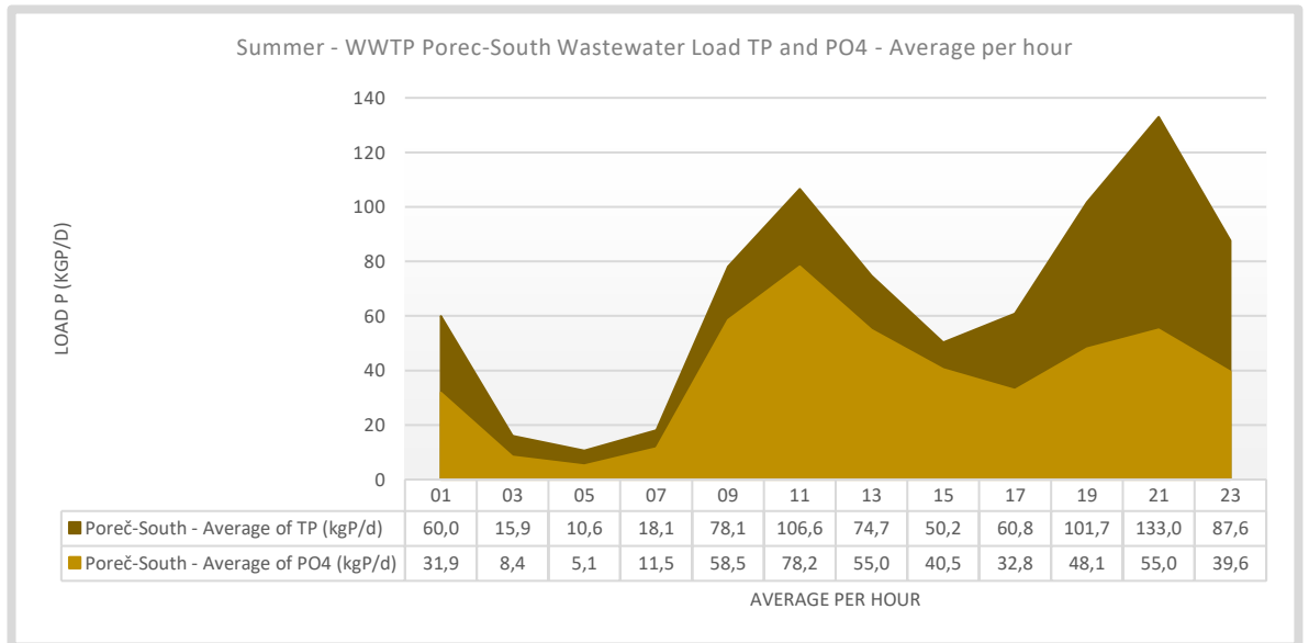
Figure 71. Summer – WWTP Poreč-South hourly average influent loads TP and PO4, based on 7 measurement days. No rain events occurred during the measurement period. This data is used to reconstruct missing data points in 7-day measurement series.
