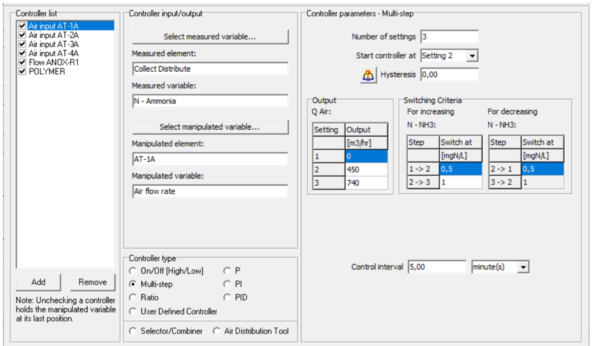
Figure 113. Summer – WWTP Poreč-South BioWin controller toolbox used for controlling the air input of AT-A. The measured variable is NH 4 in the collect distribute tank. The manipulated variable the air flow in AT-A. There are 3 settings for the air flow depending on the NH 4 concentration.
