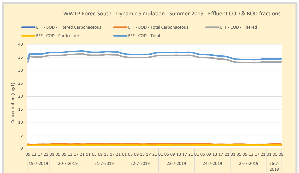
Figure 139. Summer – WWTP Poreč-South Effluent COD and BOD concentration. Effluent is measured in the outflow of the large effluent buffer. The Particulate fraction is the result of a MBR efficiency of 99,9% for particulate and 99,99% for colloidal material. Effluent is measured in the outflow of the large effluent buffer.
