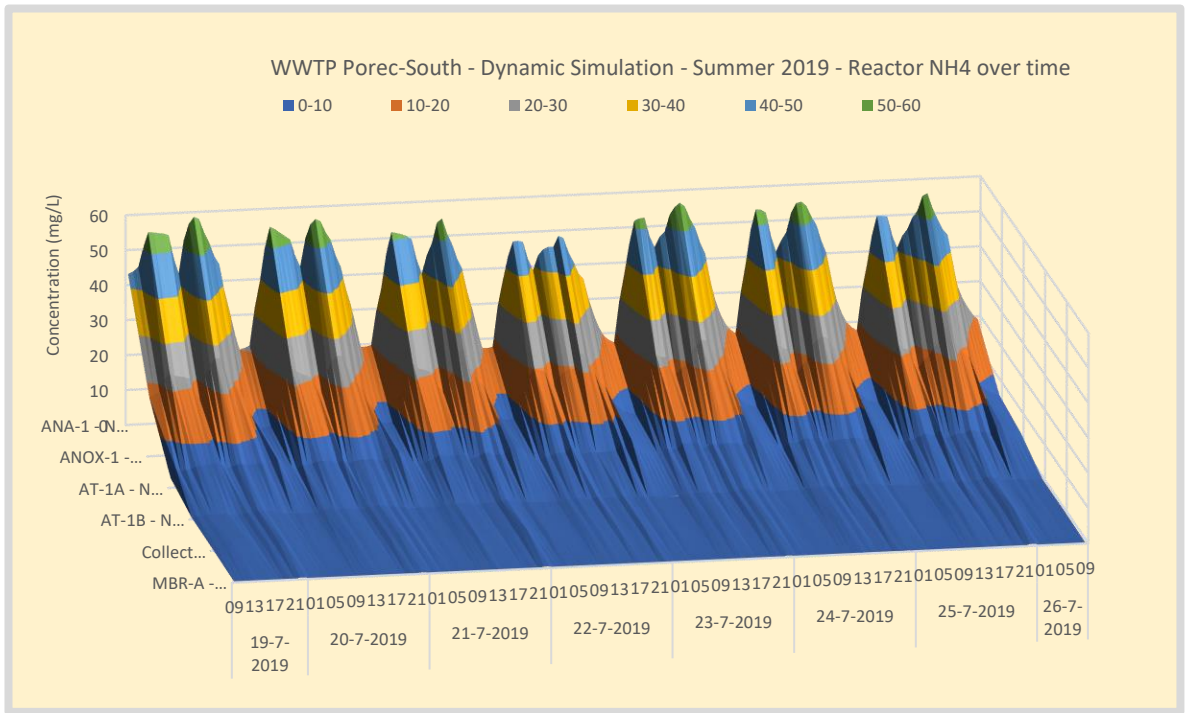
Figure 124. Summer – WWTP Poreč-South NH4 concentration profile over the waterline.
