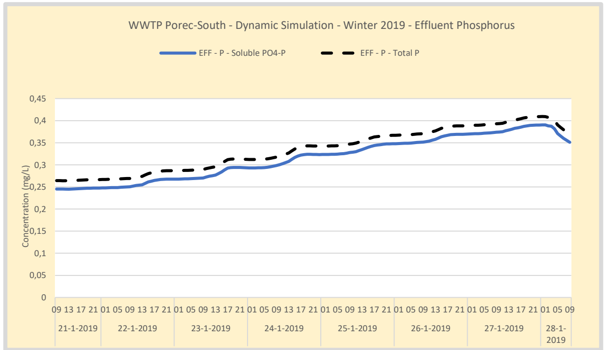
Figure 108. Winter – WWTP Poreč-South Effluent phosphorus concentration. Effluent is measured in the outflow of the large effluent buffer. The last day is a major rain event negatively effecting effluent PO 4 .
