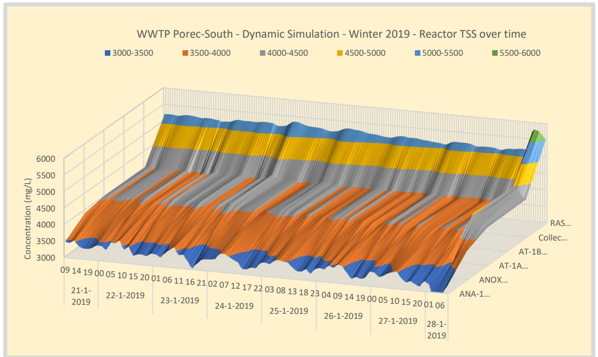
Figure 94. Winter – WWTP Poreč-South TSS concentration profile over the waterline.
