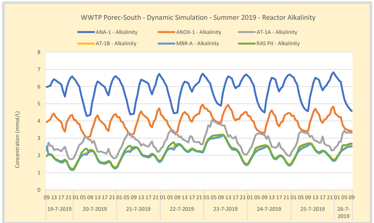
Figure 130. Summer – WWTP Poreč-South alkalinity profile over the activated sludge reactors. Influent alkalinity is estimated from local drinking water quality measurements at 7,46 mmol/L. Alkalinity is not becoming zero however potentially limiting under the operated conditions.
