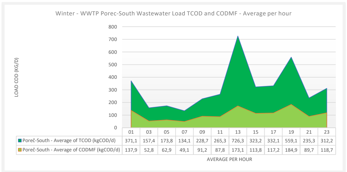
Figure 51. Winter – WWTP Poreč-South hourly average dry weather influent loads of total and filtered COD, based on 7 measurement days, excluding the rain event Monday 28-01-2019. This data is used to reconstruct missing data points in 7-day measurement series.
