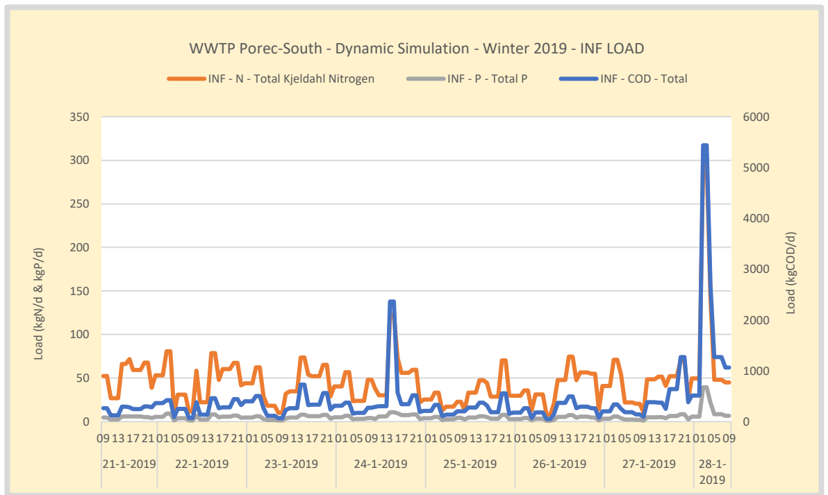
Figure 88. Winter – WWTP Poreč-South Influent loads COD, TKN and TP. 28-01-2019 a major rain event occurred. Influent peak loading events cause daily fluctuations in the effluent nitrate concentration.
