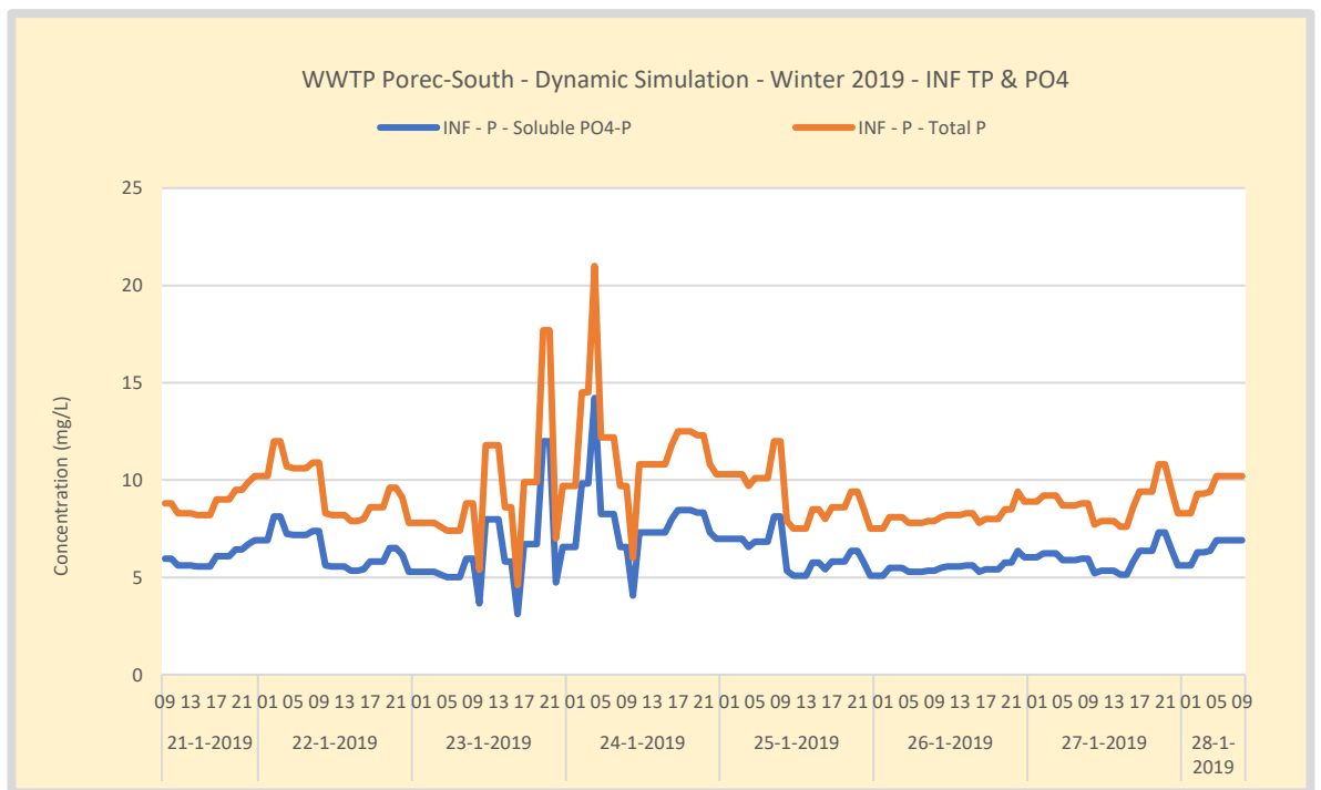
Figure 32. Dynamic Simulation – WWTP Poreč-South – Winter 24-hour average TP and PO4 influent Concentration. The model input is the measured and reconstructed TP concentration. PO4 is calculated based on a (constant) fraction determined in the influent specification. 28-01-2019 a major rain event occurred. 23-1 and 24-1 peak occurred coinciding with COD and TN indicating a (industrial) discharge event or problems with the analytical measurements.
