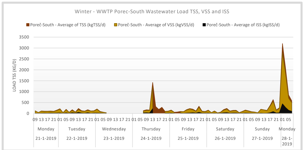
Figure 74. Winter – WWTP Poreč-South Influent TSS, VSS and ISS Loads based on 7 measurement days. A rain event occurred Monday 28-01-2019. For the model input missing data points are reconstructed based on the hourly average dry weather load. In practice TSS is difficult to get a homogeneous sample of TSS. TSS is easily biased, especially when automated samplers are used. This often results in high measurement variations.
