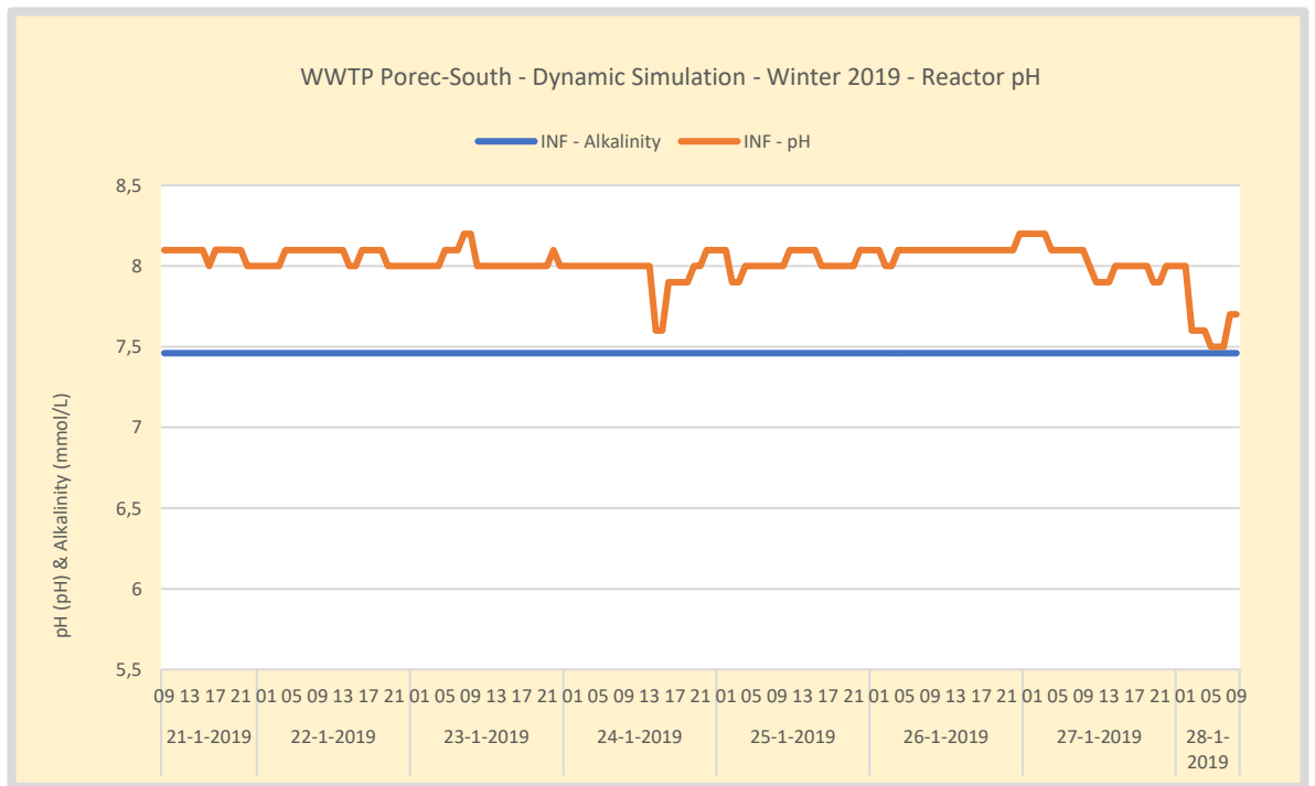
Figure 43. Dynamic Simulation – WWTP Poreč-South – Winter 24-hour average influent pH measurement. pH is a dynamic model input. The alkalinity of wastewater is estimated from Poreč drinking water quality. 28-01-2019 a major rain event occurred. The peak 22-1 coincides with other measured parameters indicating a nondomestic discharge.
