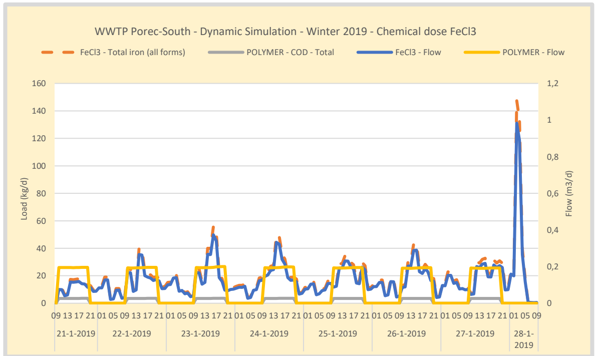
Figure 102. Winter – WWTP Poreč-South load and flow of Iron and PE. Iron is dosed proportionally to the effluent PO 4 -concentration. PE is assumed particulate biodegradable COD with a COD/VSS ratio of 1,42 gCOD/gTSS and dosed proportional to the WAS load based on 8 kg PE (dry weight) dosed per 1000 kg WAS (dry weight) flowing in the dewatering.
