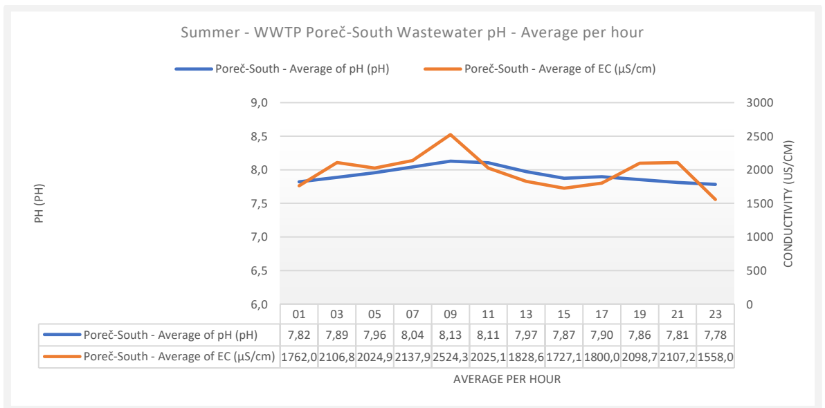
Figure 44. Summer – WWTP Poreč-South 24-hour average pH and conductivity influent measurement.
