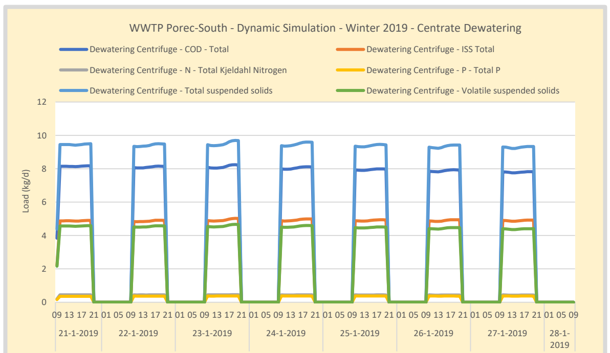
Figure 105. Winter – WWTP Poreč-South Centrate load dewatering.
