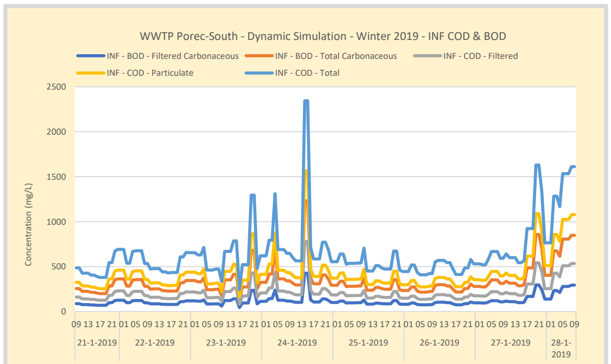
Figure 20. Dynamic Simulation – WWTP Poreč-South – Winter 24-hour average COD, COD micro-filtered, COD particulate, BOD and BOD filtered influent Concentration. The model input is the measured and reconstructed COD concentration. The other lines are calculated based on (constant) fractions determined in the influent specification. 28-01-2019 a major rain event occurred. Peaks are measured 23-1 and 24-1 indicating non-domestic discharge.
