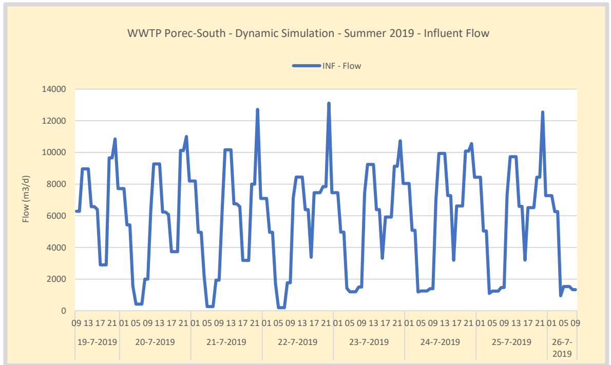
Figure 15. Summer – BioWin modelling WWTP Poreč-South: Wastewater Flow 24-hour 7-day dynamic model input data. In the model data are interpolated on an hourly basis.
