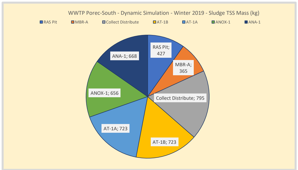
Figure 82. Winter – WWTP Poreč-South sludge mass distribution (kgTSS) in the reactor tanks. Based on these data and the average sludge production, the SRT of the WWTP is calculated. Mass of idle tanks is not included.
