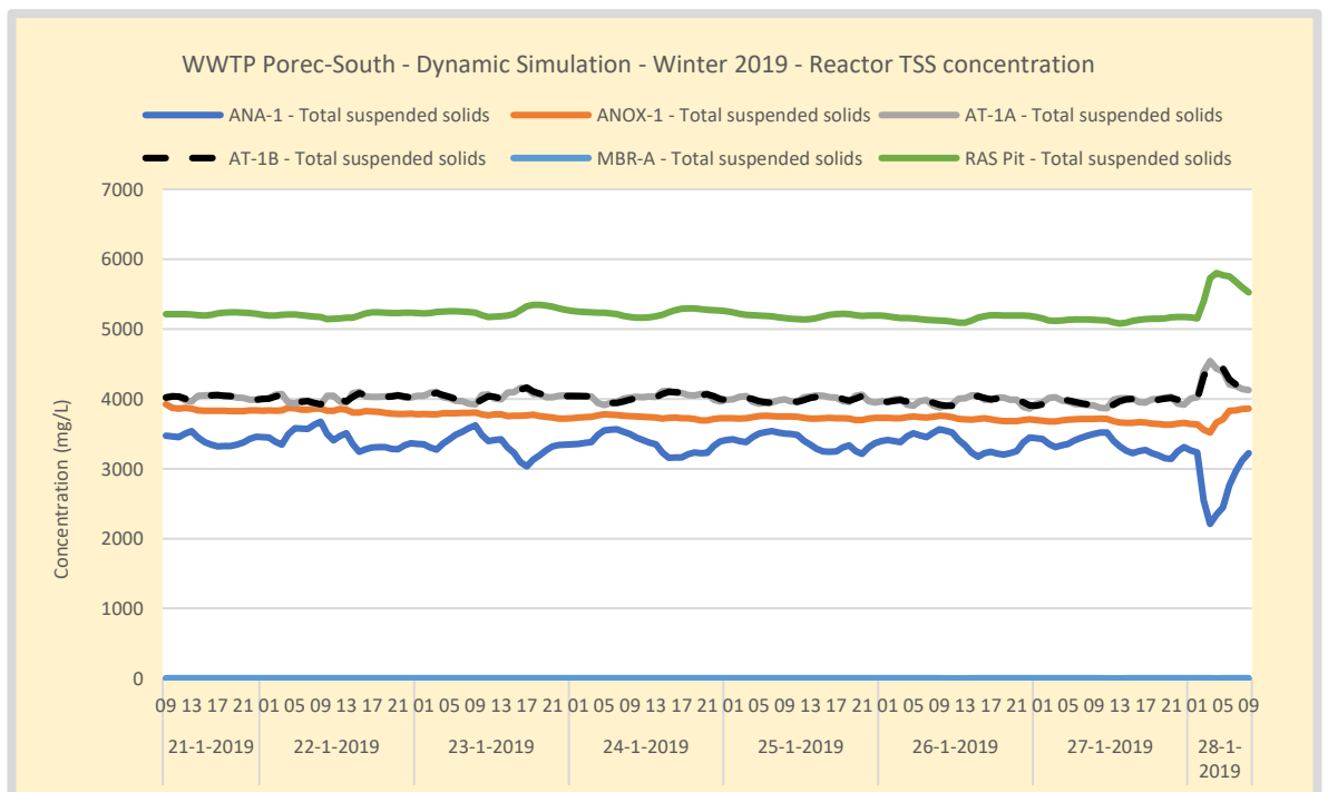
Figure 91. Winter – WWTP Poreč-South TSS profile in the waterline. TSS in the MBR is controlled on approximately 5 gTSS/L by adjusting the WAS flow and SRT. In the winter, the reactor volume relative to the influent loading is very high. This results in low sludge production and a too long SRT. The process is therefore operated with a lower TSS concentration during the winter.
