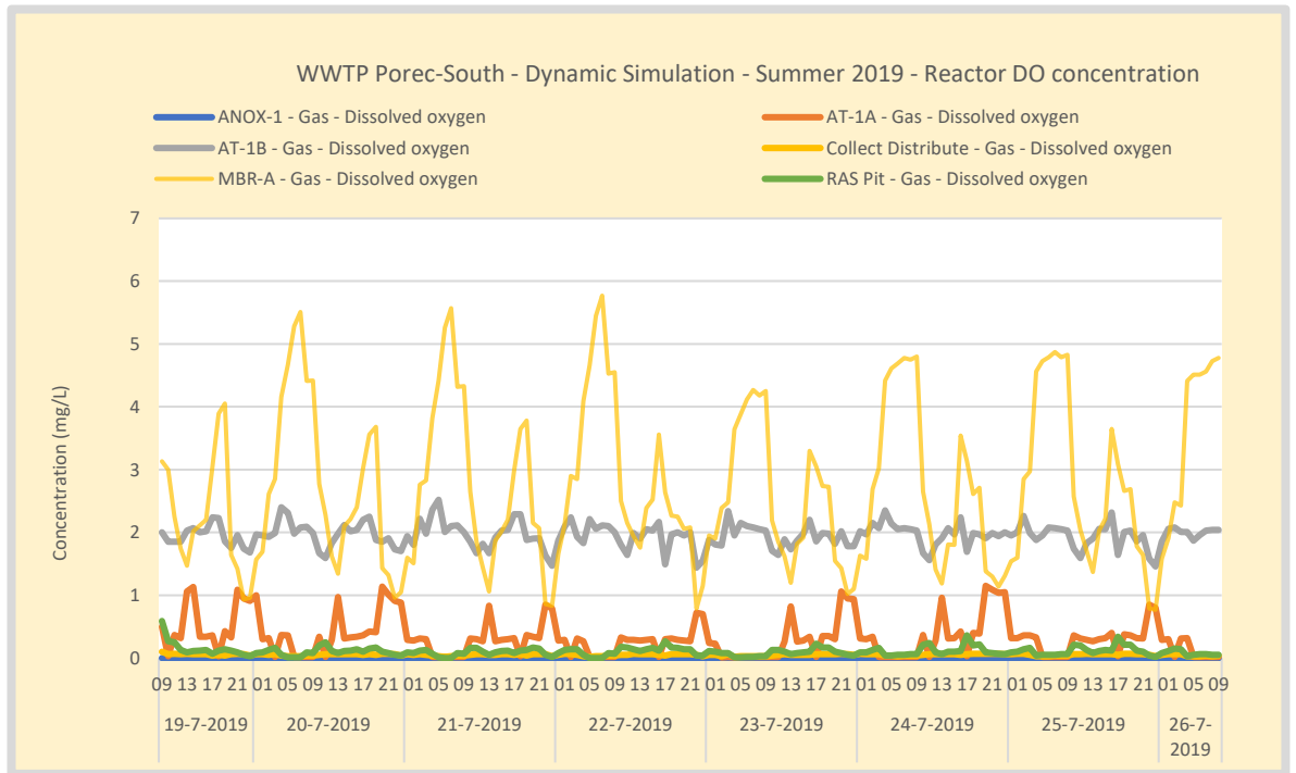
Figure 128. Summer – WWTP Poreč-South DO concentration gradients. DO is controlled in the AT-B on 2 mgO 2 /L and the air flow of AT-B on NH 4 concentration in the outflow of the aeration. In the MBR the DO is the result of the designed maximum air input. Little oxygen is recycled over the reactors and little oxygen is measured in the anoxic zone. The DO setpoint can be maintained based on the designed air flow.
