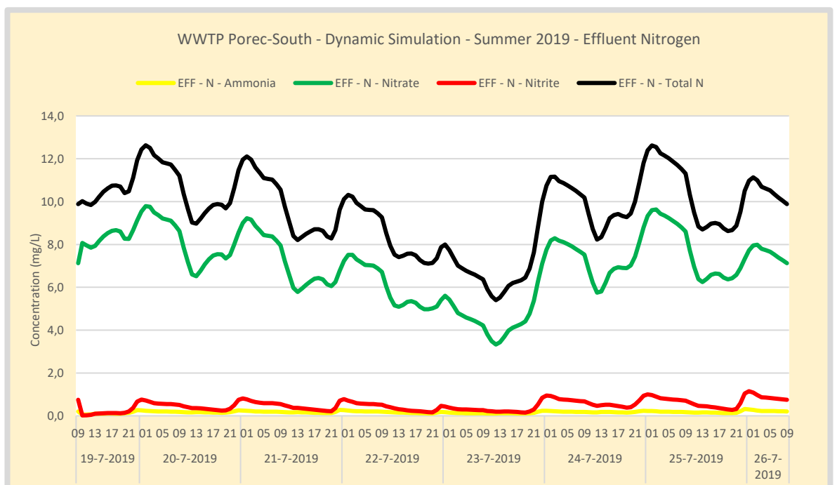
Figure 137. Summer – WWTP Poreč-South Effluent nitrogen concentration. Effluent is measured in the outflow of the large effluent buffer. Nitrite production is low and aeration capacity sufficient.
