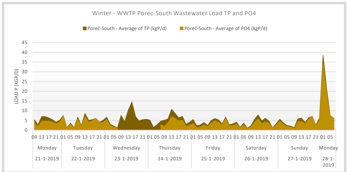
Figure 66. Winter – WWTP Poreč-South Influent TP and PO4 Loads based on 7 measurement days. A rain event occurred Monday 28-01-2019. For the model input missing data points are reconstructed based on the hourly average dry weather load.
