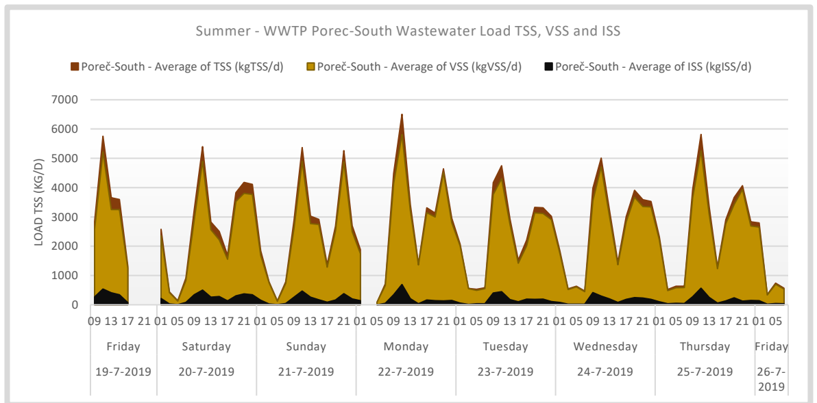
Figure 78. Summer - WWTP Poreč-South Wastewater Loads TSS, VSS and ISS. No rain events occurred during the measurement period. For the model input missing data points are reconstructed based on the hourly average load.
