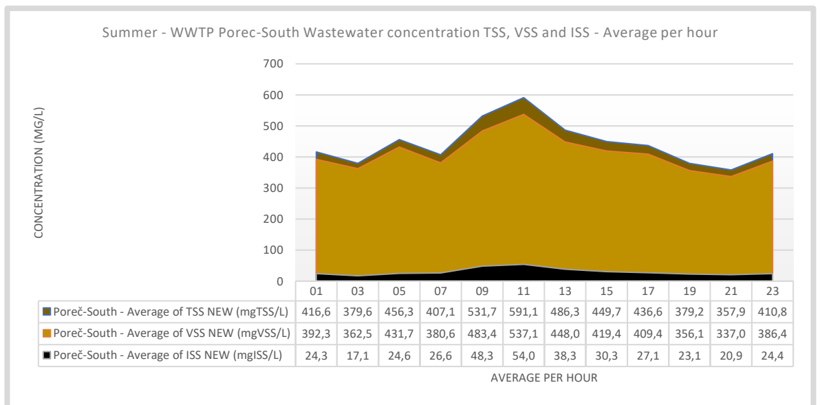
Figure 40. Summer – WWTP Poreč-South 24-hour average TSS, VSS and ISS influent Concentration.
