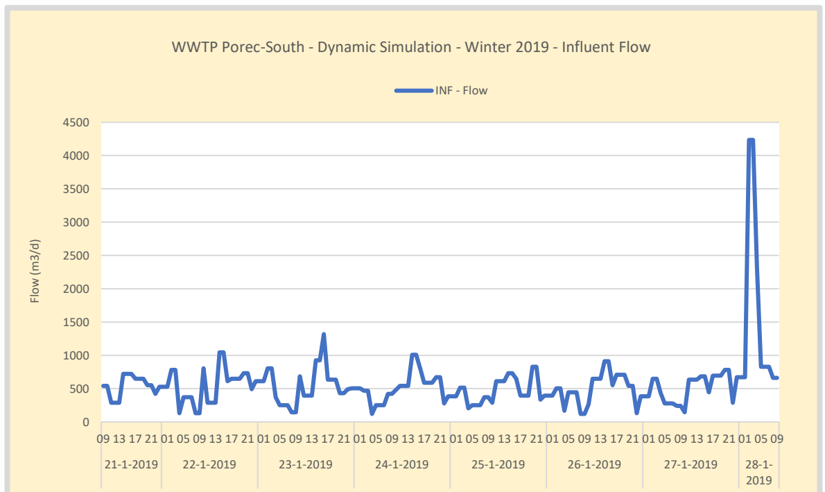
Figure 87. Winter – WWTP Poreč-South Influent flow. 28-01-2019 a major rain event occurred.
