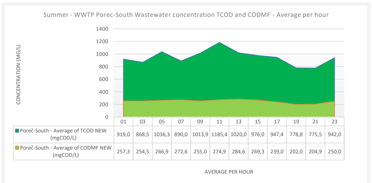
Figure 22. Summer – WWTP Poreč-South 24-hour average COD and COD micro-filtered influent Concentration. While soluble COD is relative constant the total which also contains the particulate is more distributed towards the first flow peak of the day.
