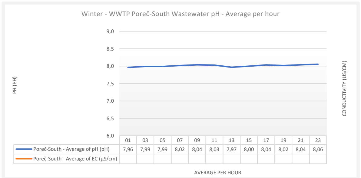
Figure 42. Winter – WWTP Poreč-South 24-hour average pH influent measurement. During the winter period no conductivity was measured.
