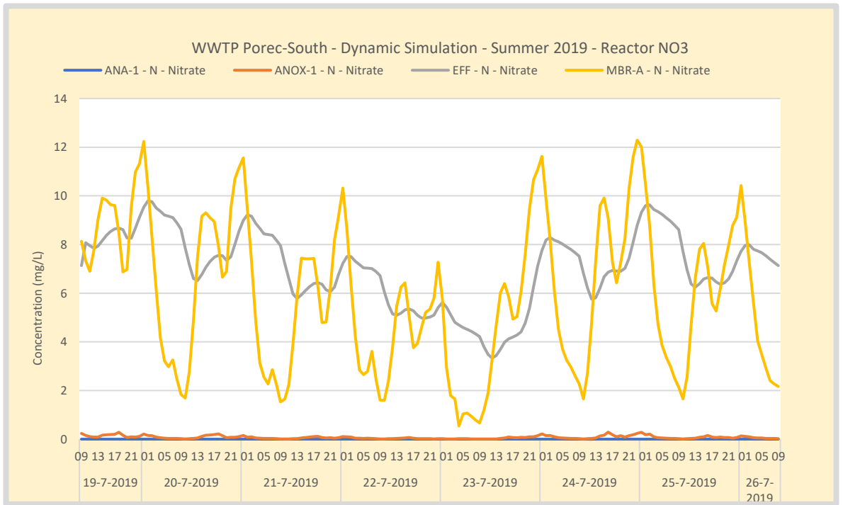
Figure 122. Summer – WWTP Poreč-South nitrate in the anoxic tank. The anoxic recycle rate is controlled on a nitrate setpoint of 2 mgNO 3 /L in the anoxic tank. Internal recycle capacity is not sufficient to reach this setpoint. NO 3 in the anoxic tank is almost zero at maximum recycle rate.
