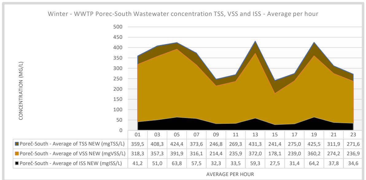
Figure 37. Winter – WWTP Poreč-South 24-hour average TSS, VSS and ISS influent Concentration.
