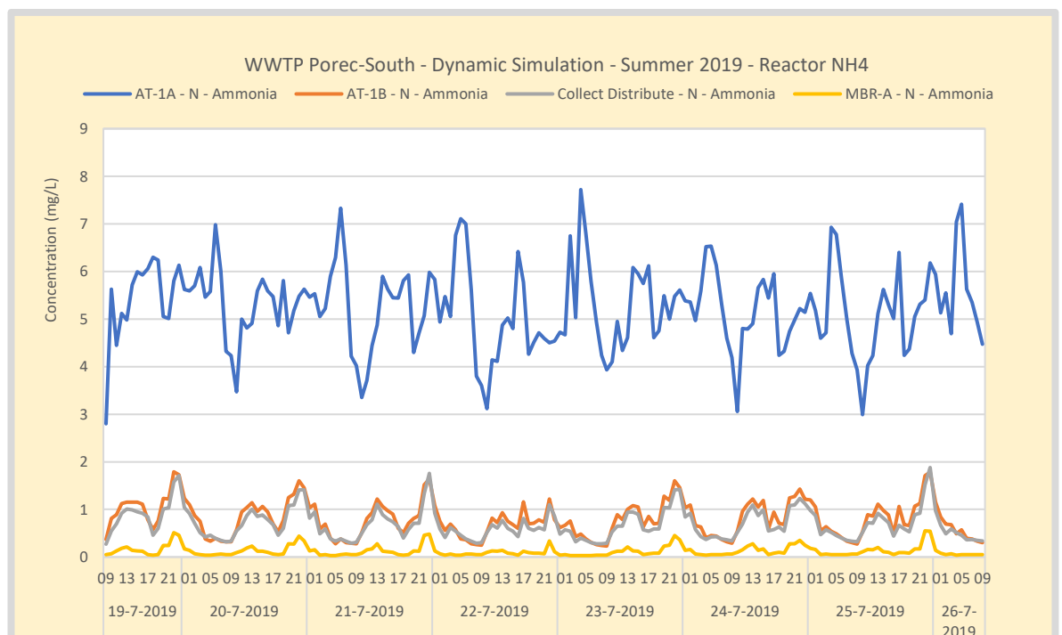
Figure 121. Summer – WWTP Poreč-South ammonium profile in the waterline. The air input of AT-A is controlled based on \text{NH}_4 measured in the collect distribute tank using a 3-step controller. Above 1,0 \text{mgNH}_4/\text{L} the air input goes to its maximum value. Below 0,5 air shuts off. AT-B is DO controlled on 2,0 \text{mgO}_2/\text{L} .
