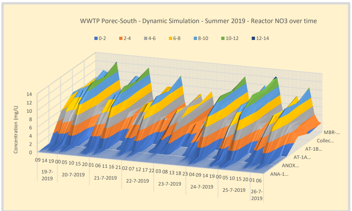
Figure 125. Summer – WWTP Poreč-South NO3 concentration profile over the waterline.
