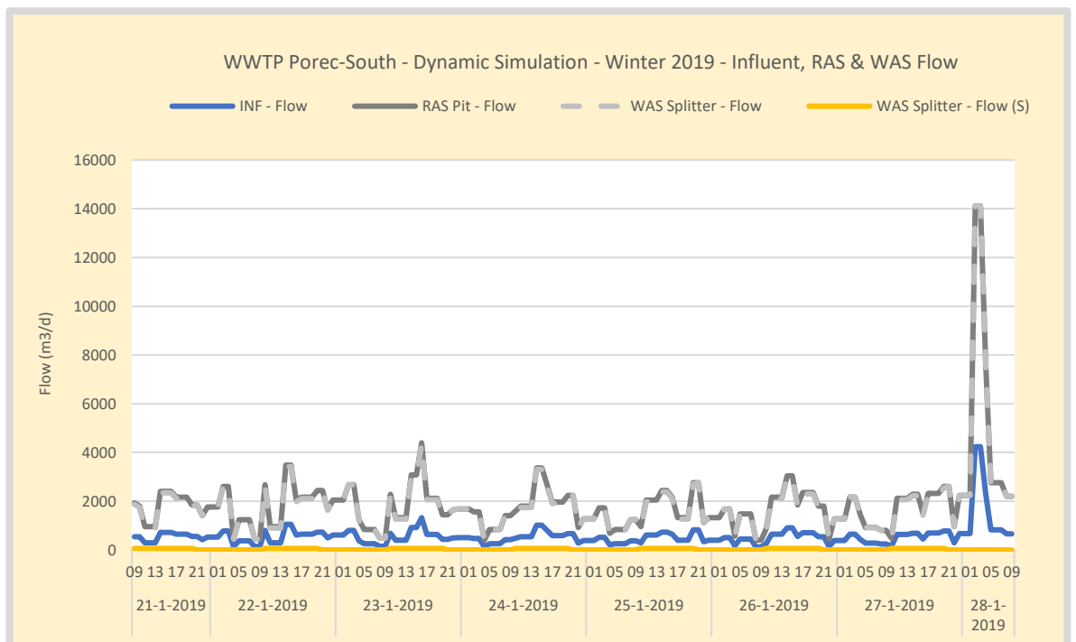
Figure 89. Winter – WWTP Poreč-South flow rate settings and control. The MLSS sludge return flow is controlled proportional to the influent. This results in a more stable TSS concentration in the reactors. The WAS flow is operated 10 hours a day on a constant flow to the dewatering.
