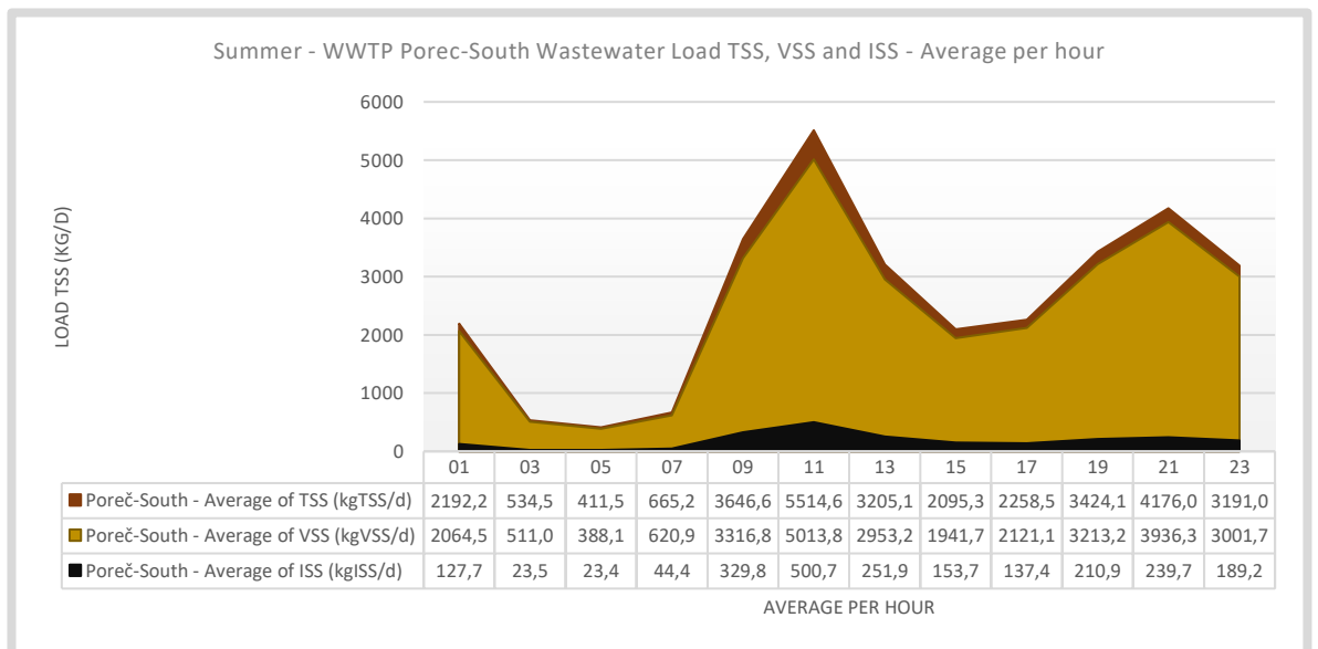
Figure 79. Summer – WWTP Poreč-South hourly average influent loads TSS, VSS and ISS, based on 7 measurement days. No rain events occurred during the measurement period. This data is used to reconstruct missing data points in 7-day measurement series.
