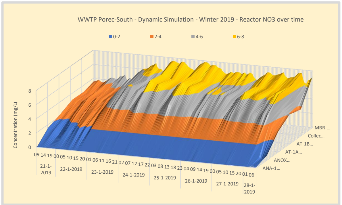
Figure 96. Winter – WWTP Poreč-South NO3 concentration profile over the waterline.
