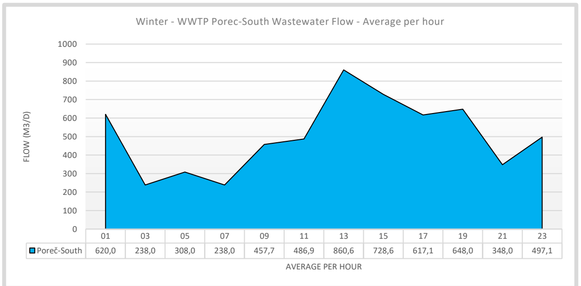
Figure 7. Winter - WWTP Poreč-South Dry Weather Wastewater Flow 24-hour average hourly measurements. These data are used to reconstruct missing datapoints in the 7-day 24-hours measurements and can be used for scenario calculations.
