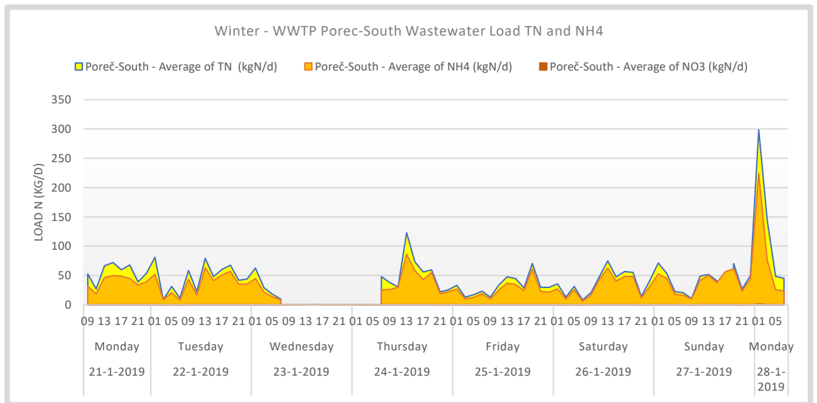
Figure 58. Winter – WWTP Poreč-South Influent TN, NH4 and NO3 Loads based on 7 measurement days. A rain event occurred Monday 28-01-2019. For the model input missing data (23-1) points are reconstructed based on the hourly average dry weather load.
