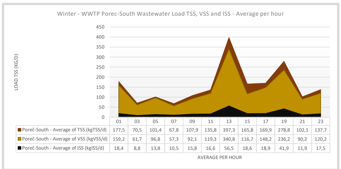
Figure 75. Winter – WWTP Poreč-South hourly average influent loads TSS, VSS and ISS, based on 7 measurement days, excluding the rain event Monday 28-01-2019. This data is used to reconstruct missing data points in 7-day measurement series.
