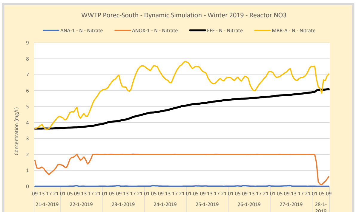
Figure 93. Winter – WWTP Poreč-South nitrate in the anoxic tank. The anoxic recycle rate is controlled on a nitrate setpoint of 2 \text{ mgNO}_3/\text{L} in the anoxic tank. The setpoint can be reached during most of the 7-day operation.
