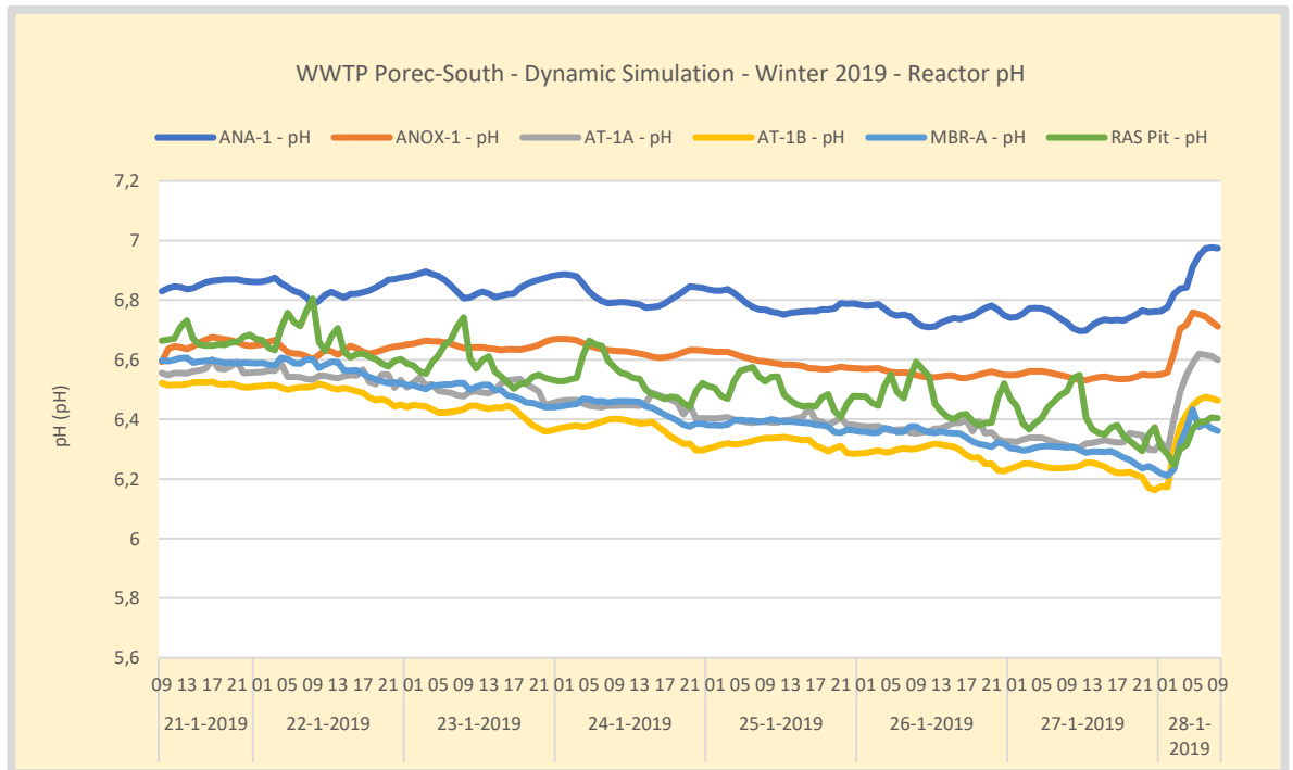
Figure 100. Winter – WWTP Poreč-South pH profile over the activated sludge reactors. Influent pH is measured continuously and is not limiting.
