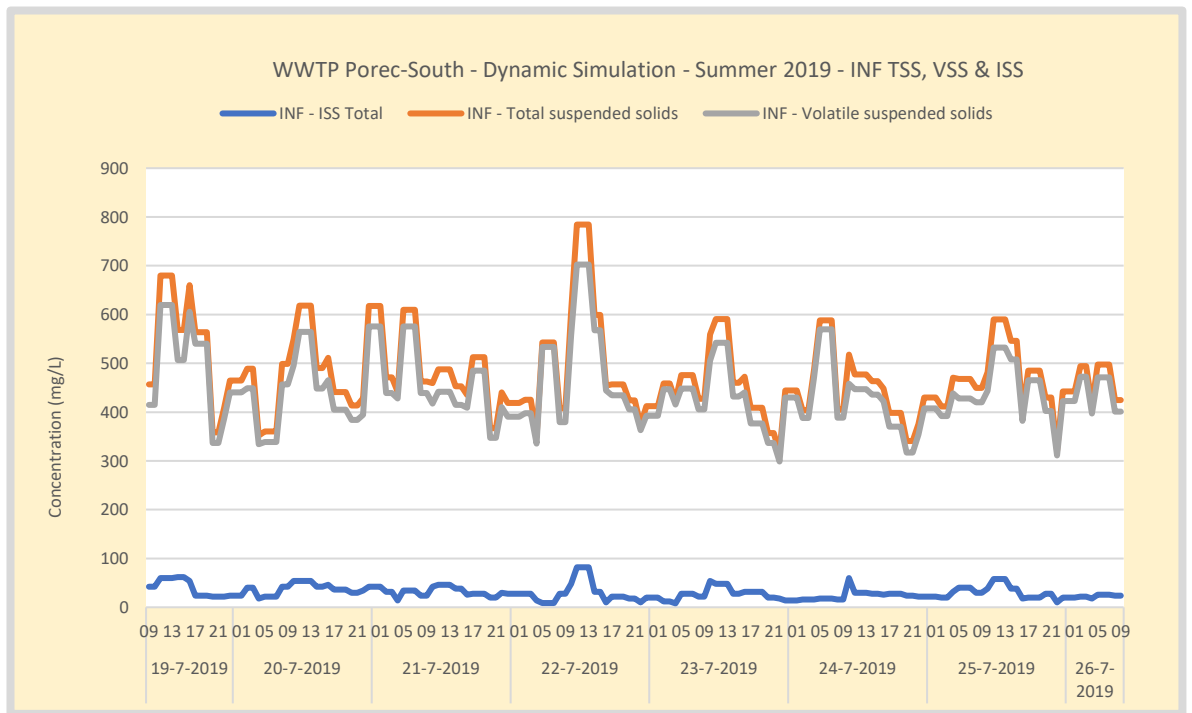
Figure 41. Dynamic Simulation – WWTP Poreč-South – Summer 24-hour average TSS, VSS (organic particulate) and ISS (inorganic particulate) influent Concentration. The model input is the measured and reconstructed ISS concentration. VSS is calculated based on (constant) fractions determined in the influent specification. TSS is modelled as the sum of ISS and VSS. No rain occurred. A peak measured 22-7 could indicate a measurement error.
