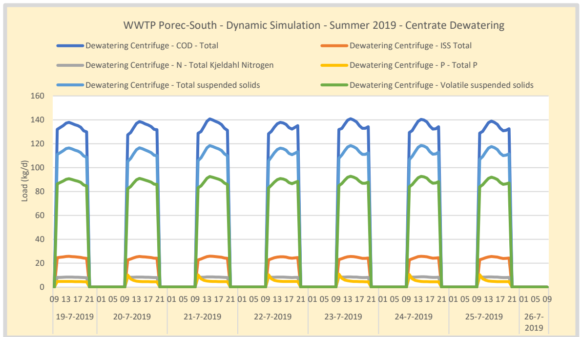
Figure 134. Summer – WWTP Poreč-South Centrate load dewatering.
