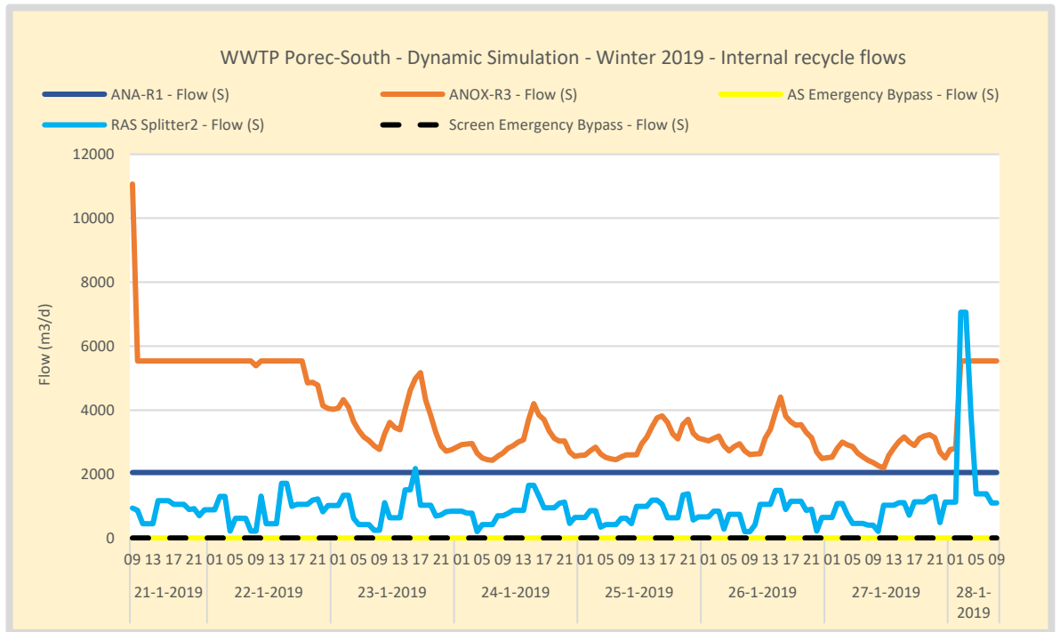
Figure 90. Winter – WWTP Poreč-South flow rate settings and control. The bypasses are not used. The anoxic recycle is controlled based on nitrate in the anoxic tank. The flow is reduced when Nitrate becomes higher than 2 mgNO 3 /L.
