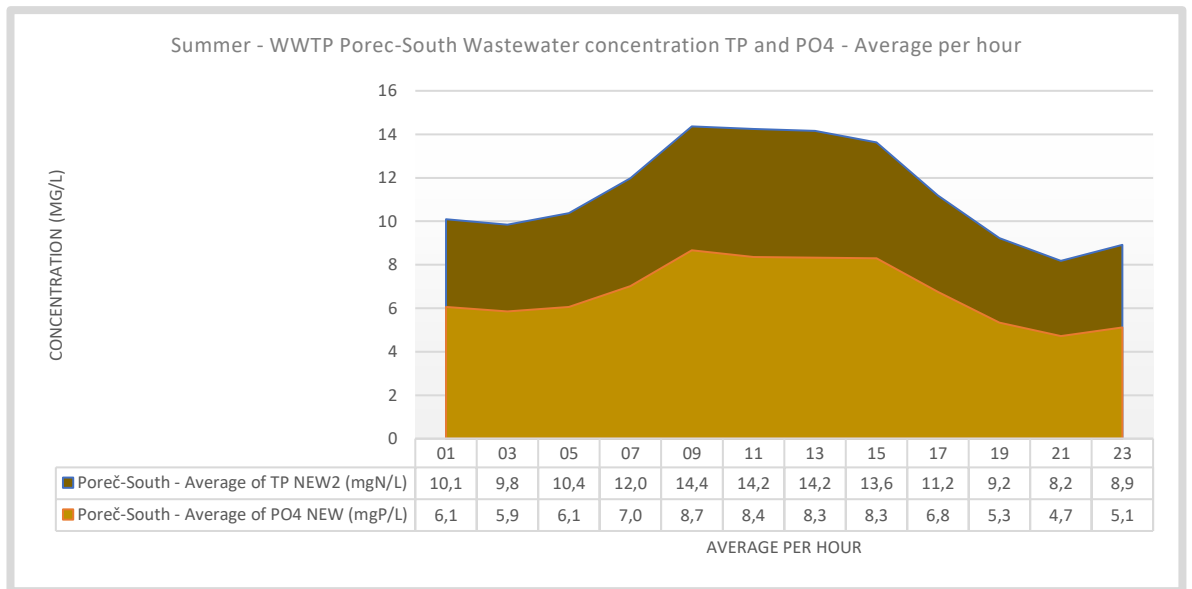
Figure 34. Summer – WWTP Poreč-South 24-hour average TP and PO4 influent Concentration. The figure shows a typical concentration distribution for domestic sewage, in accordance with TN, with a peak in the morning. TP has a larger particulate fraction which results in a peak arriving later in the day compared to TN.
