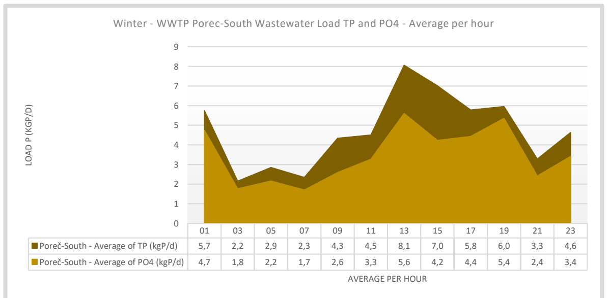
Figure 67. Winter – WWTP Poreč-South hourly average influent loads TP and PO4, based on 7 measurement days, excluding the rain event Monday 28-01-2019. This data is used to reconstruct missing data points in 7-day measurement series.
