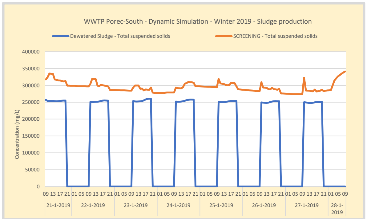
Figure 104. Winter – WWTP Poreč-South dewatered sludge and screening sludge concentration. The design assumes dewatered sludge at 23% dry matter. Screening is an estimated concentration as the result of the press operation.
