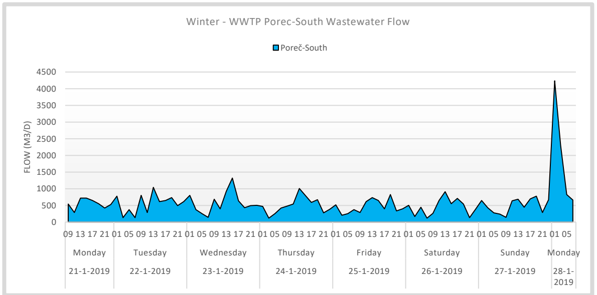
Figure 6. Winter - WWTP Poreč-South Wastewater Flow 24-hour 7-day dynamic measurements. This data is used for dynamic modelling.
