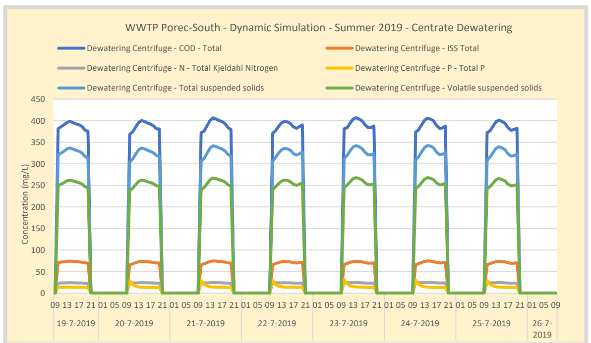
Figure 135. Summer – WWTP Poreč-South Centrate concentrations dewatering.
