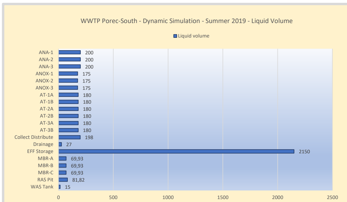
Figure 111. WWTP Poreč-South – Volume distribution of modelled reactor elements. The actual WAS tank is 150 m3 however the sludge volume is modelled based on an HRT less than 2,5 hours to avoid P-release. The WAS tank is not suitable for sludge storage.
