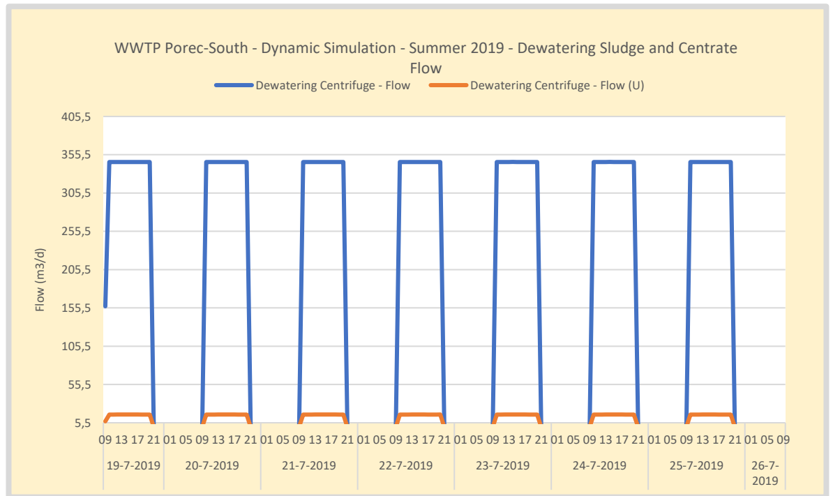
Figure 132. Summer – WWTP Poreč-South dewatered sludge and centrate flow.
