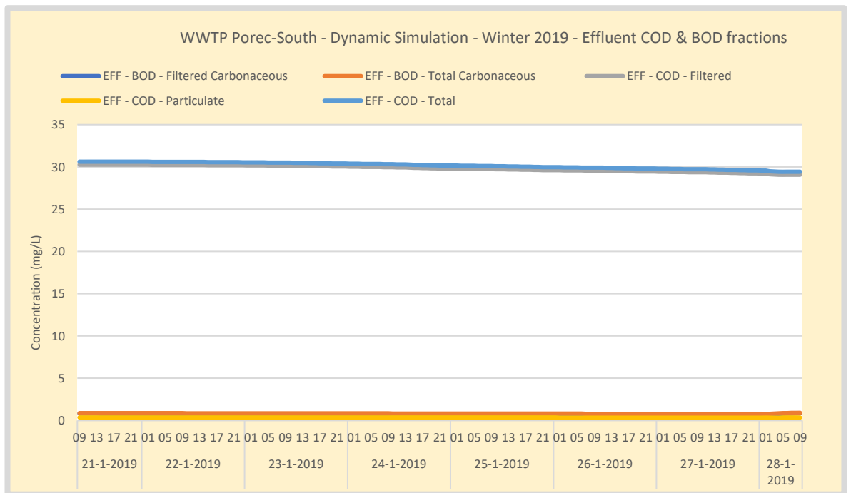
Figure 109. Winter – WWTP Poreč-South Effluent COD and BOD concentration. Effluent is measured in the outflow of the large effluent buffer. The Particulate fraction is the result of a MBR efficiency of 99,9% for particulate and 99,99% for colloidal material. Effluent is measured in the outflow of the large effluent buffer.
