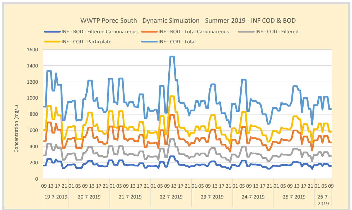
Figure 23. Dynamic Simulation – WWTP Poreč-South – Summer 24-hour average COD, COD micro-filtered, COD particulate, BOD and BOD filtered influent Concentration. The model input is the measured and reconstructed COD concentration. The other lines are calculated based on (constant) fractions determined in the influent specification. No rain occurred. 22-7-2019 a COD concentration peak was measured.
