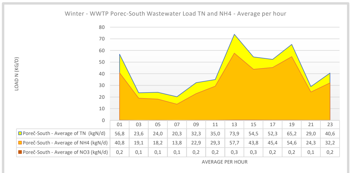
Figure 59. Winter – WWTP Poreč-South hourly average dry weather influent loads TN, NH4 and NO3, based on 7 measurement days, excluding the rain event Monday 28-01-2019. This data is used to reconstruct missing data points in 7-day measurement series.
