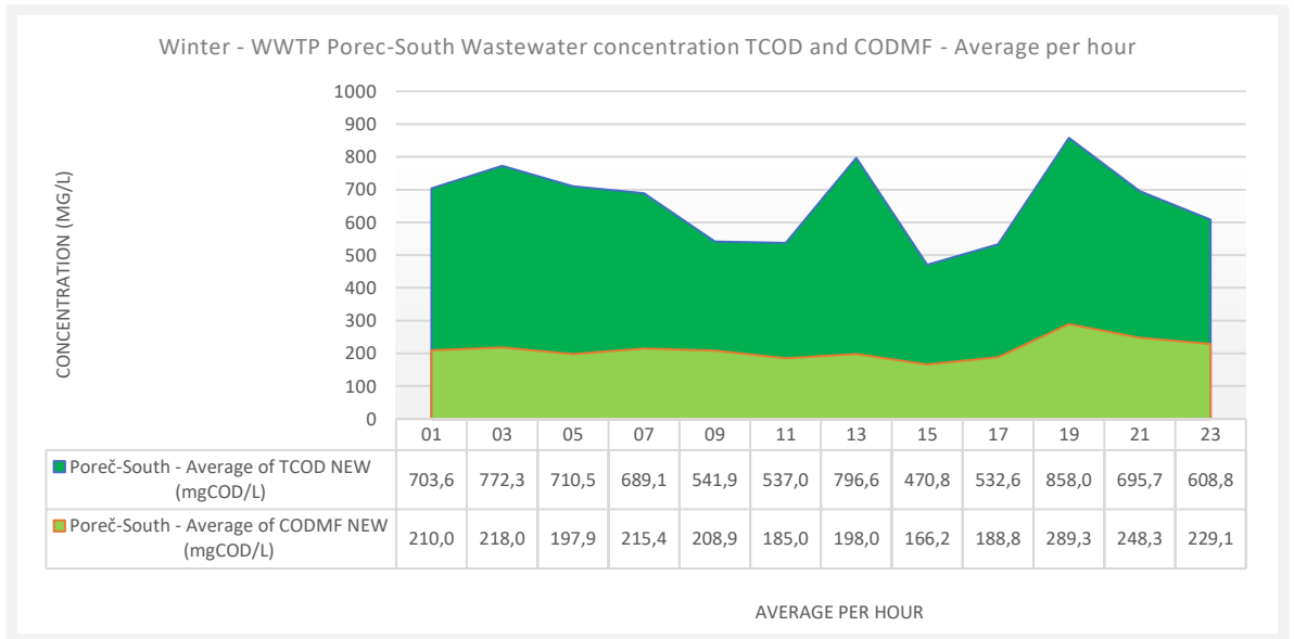
Figure 19. Winter – WWTP Poreč-South 24-hour average COD and COD micro-filtered influent Concentration.
