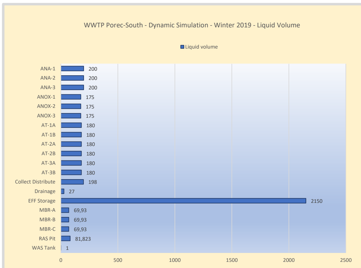
Figure 81. WWTP Poreč-South – Volume distribution of modelled reactor elements. The actual WAS tank is 150 m3 however the sludge volume is modelled based on an HRT less than 2,5 hours to avoid P-release. The WAS tank is not suitable for sludge storage.
