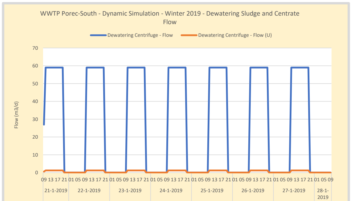
Figure 103. Winter – WWTP Poreč-South dewatered sludge and centrate flow.
