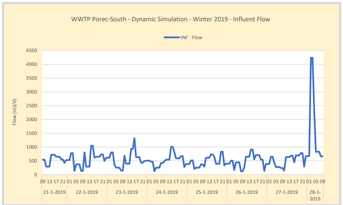
Figure 8. Winter – BioWin modelling WWTP Poreč-South: Wastewater Flow 24-hour 7-day dynamic model input data. Some datapoint are reconstructed from 24-hour average hourly measurements. The data is interpolated in the model on an hourly basis.
