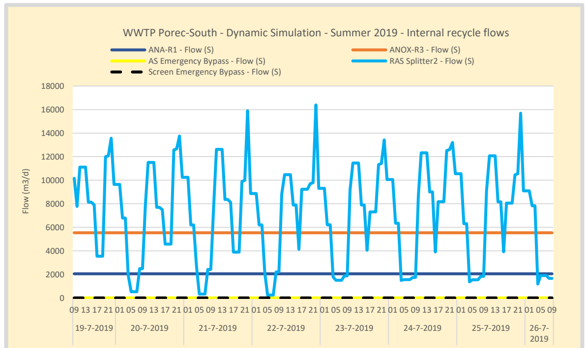
Figure 119. Summer – WWTP Poreč-South flow rate settings and control. The bypasses are not used. The anoxic recycle is controlled based on nitrate in the anoxic tank. The flow is reduced when Nitrate becomes higher than 2 mgNO 3 /L. The fact that this setpoint cannot be reached, indicates the recycle is limiting or that the anoxic tank is too large.
