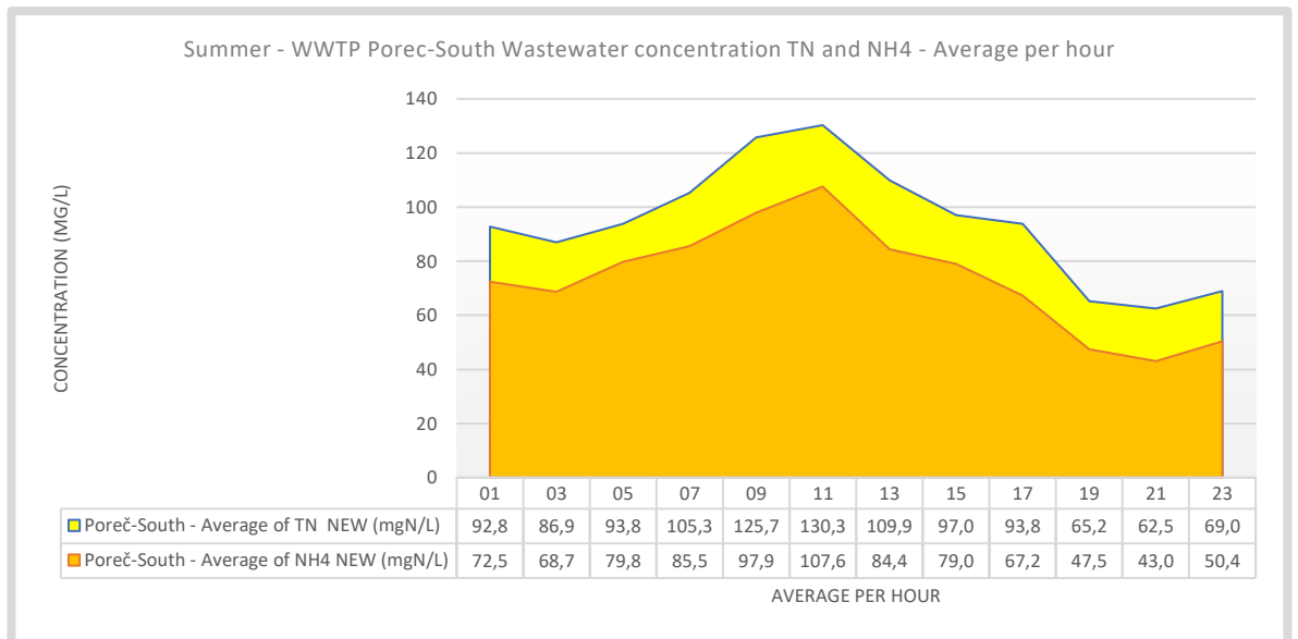
Figure 28. Summer – WWTP Poreč-South 24-hour average TN and NH4 influent Concentration. A typical distribution with peak in the morning. Based on the time of the morning peak the estimated sewer HRT is 4 hours.
