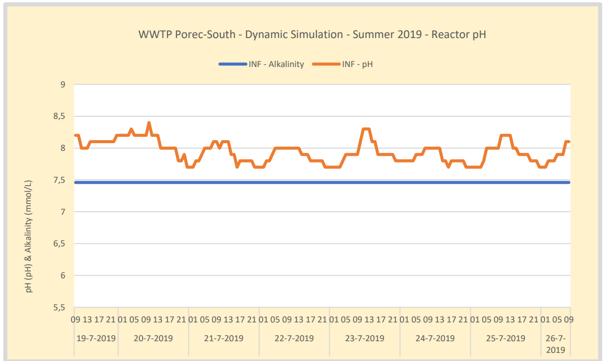
Figure 45. Dynamic Simulation – WWTP Poreč-South – Summer 24-hour average influent pH measurement. pH is a dynamic model input. The alkalinity of wastewater is estimated from Poreč drinking water quality.
