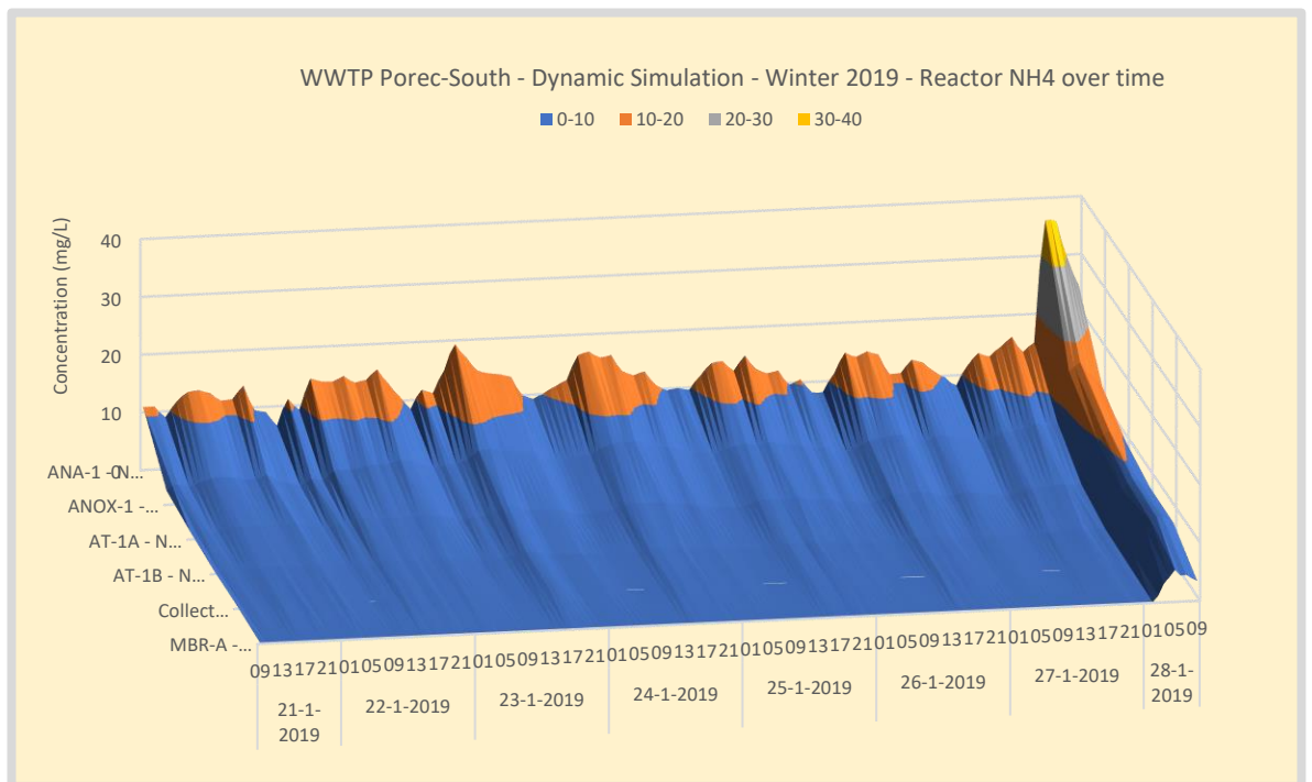
Figure 95. Winter – WWTP Poreč-South NH4 concentration profile over the waterline.
