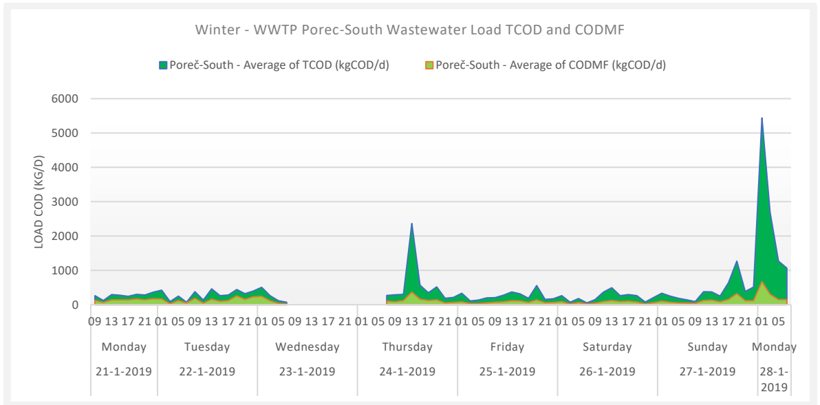
Figure 50. Winter – WWTP Poreč-South Influent Total and filtered COD Loads based on 7 measurement days. A rain event occurred Monday 28-01-2019. For the model input missing data points (23-1) are reconstructed based on the hourly average dry weather load.
