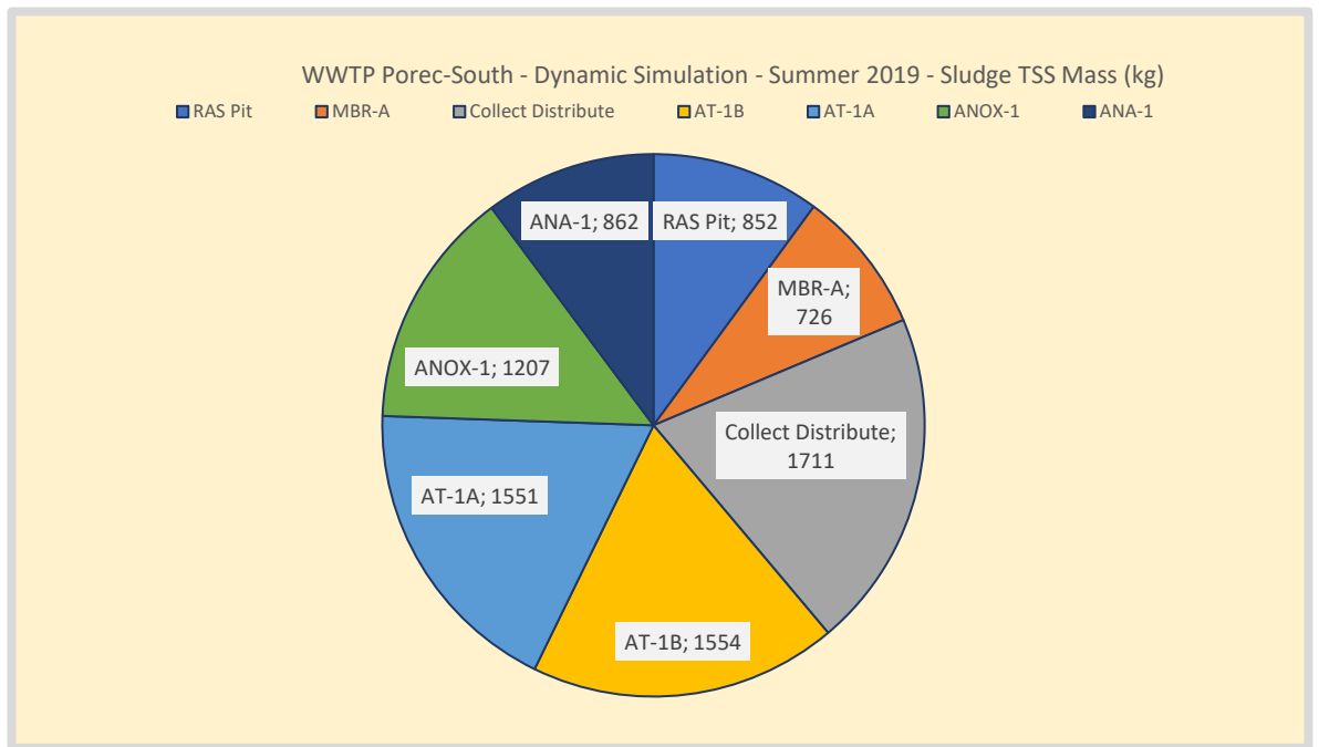
Figure 112. Summer – WWTP Poreč-South sludge mass distribution (kgTSS) in the reactor tanks. Based on these data and the average sludge production, the SRT of the WWTP is calculated. All operated reactors containing activated sludge are included in the SRT calculations.
