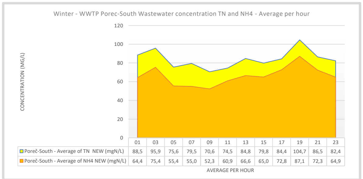
Figure 25. Winter – WWTP Poreč-South 24-hour average TN and NH4 influent Concentration.
