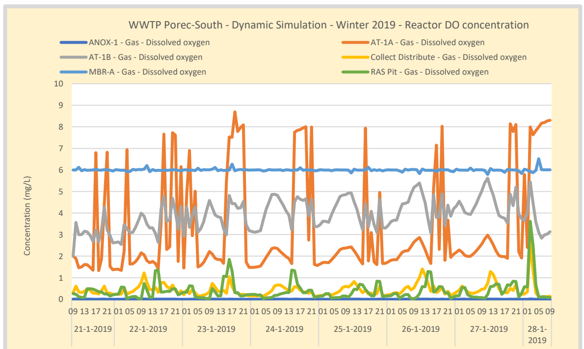
Figure 99. Winter – WWTP Poreč-South DO concentration gradients. DO is controlled in the AT. In the MBR the DO is the result of the designed air input. Oxygen is recycled over the reactors causing accumulation of DO in the AT during periods of low influent loading.
