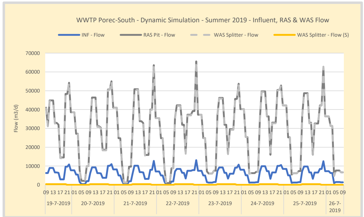
Figure 118. Summer – WWTP Poreč-South flow rate settings and control. The MLSS sludge return flow is controlled proportional to the influent. The WAS flow is time controlled and operated 10 hours a day on a constant flow.
