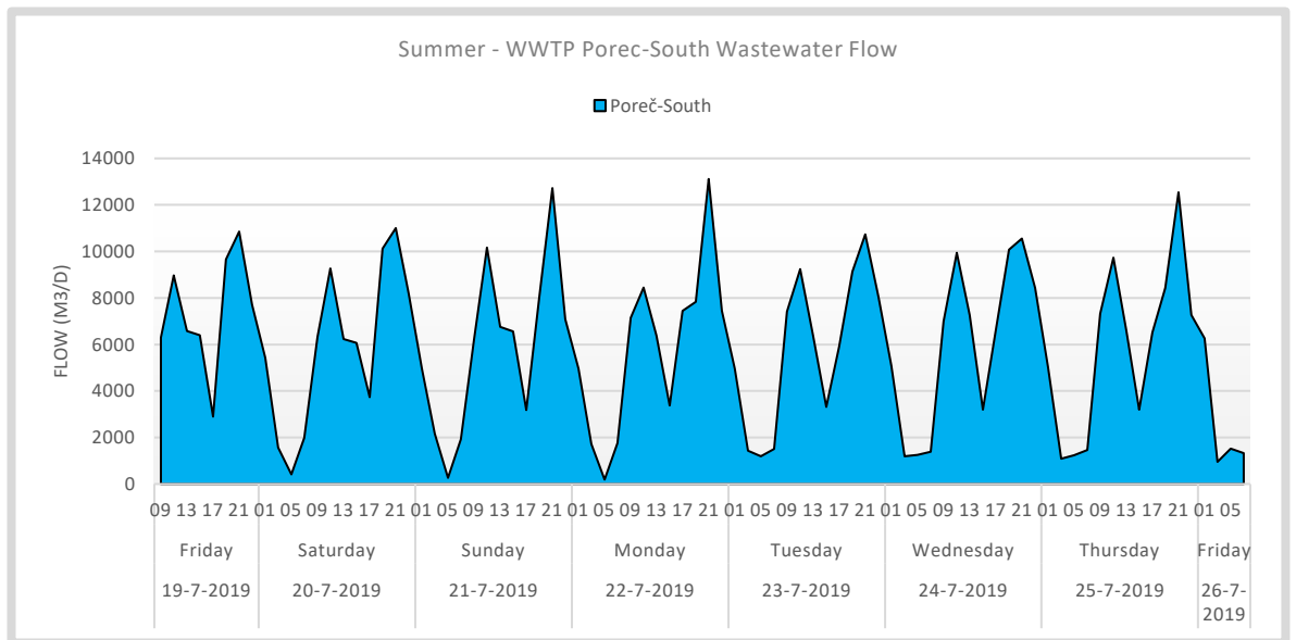
Figure 13. Summer - WWTP Poreč-South Dry Weather Wastewater Flow 24-hour 7-day dynamic measurements. No rain events occurred during the measurements.
