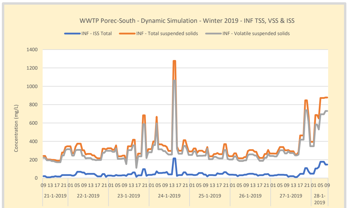
Figure 38. Dynamic Simulation – WWTP Poreč-South – Winter 24-hour average TSS, VSS (organic particulate) and ISS (inorganic particulate) influent Concentration. The model input is the measured and reconstructed ISS concentration. VSS is calculated based on (constant) fractions determined in the influent specification. TSS is modelled as the sum of ISS and VSS. 28-01-2019 a major rain event occurred causing an increase in the TSS concentration. TSS peaks around 23 and 24-1 coincide with other measured parameters and could indicate a nondomestic discharge.
