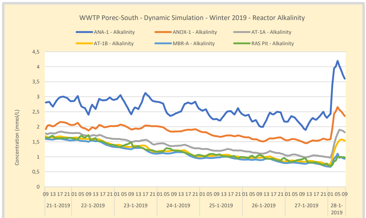
Figure 101. Winter – WWTP Poreč-South alkalinity profile over the activated sludge reactors. Influent alkalinity is estimated from local drinking water quality measurements at 7,46 mmol/L. Potentially there is a limitation of alkalinity in the winter due to CO 2 stripping caused by over aeration.
