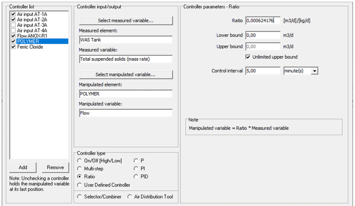
Figure 85. Winter – WWTP Poreč-South BioWin controller toolbox used for controlling the polymer dosage of the dewatering. Indicated are the measured variable being the TSS load entering the dewatering and manipulated variable the PE flow. The applied control ratio is 8 kg PE per 1000 kg TSS based on dry weight. PE is assumed to be particulate substrate with a COD/VSS ratio of 1,42.
