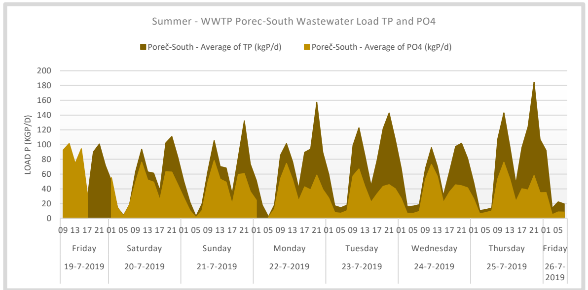
Figure 70. Summer - WWTP Poreč-South Wastewater Loads TP and PO4. No rain events occurred during the measurement period. For the model input missing data points are reconstructed based on the hourly average dry weather load.
