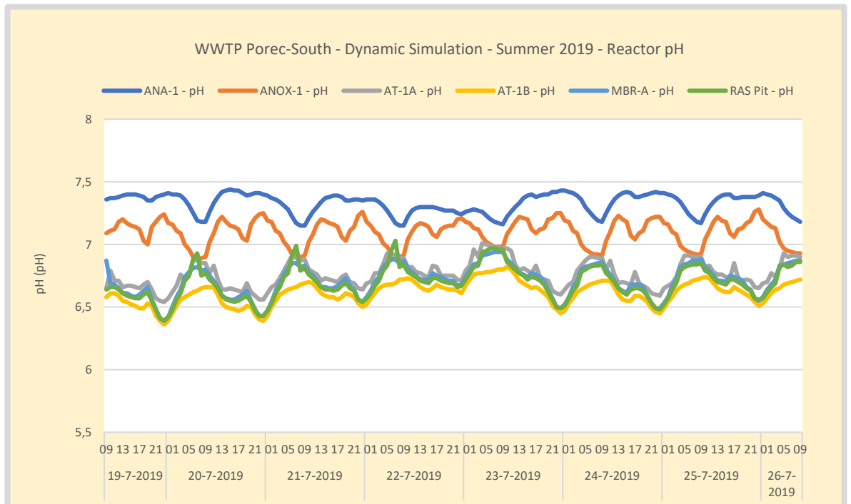
Figure 129. Summer – WWTP Poreč-South pH profile over the activated sludge reactors. Influent pH is measured continuously and is not limiting. pH is not limiting.
