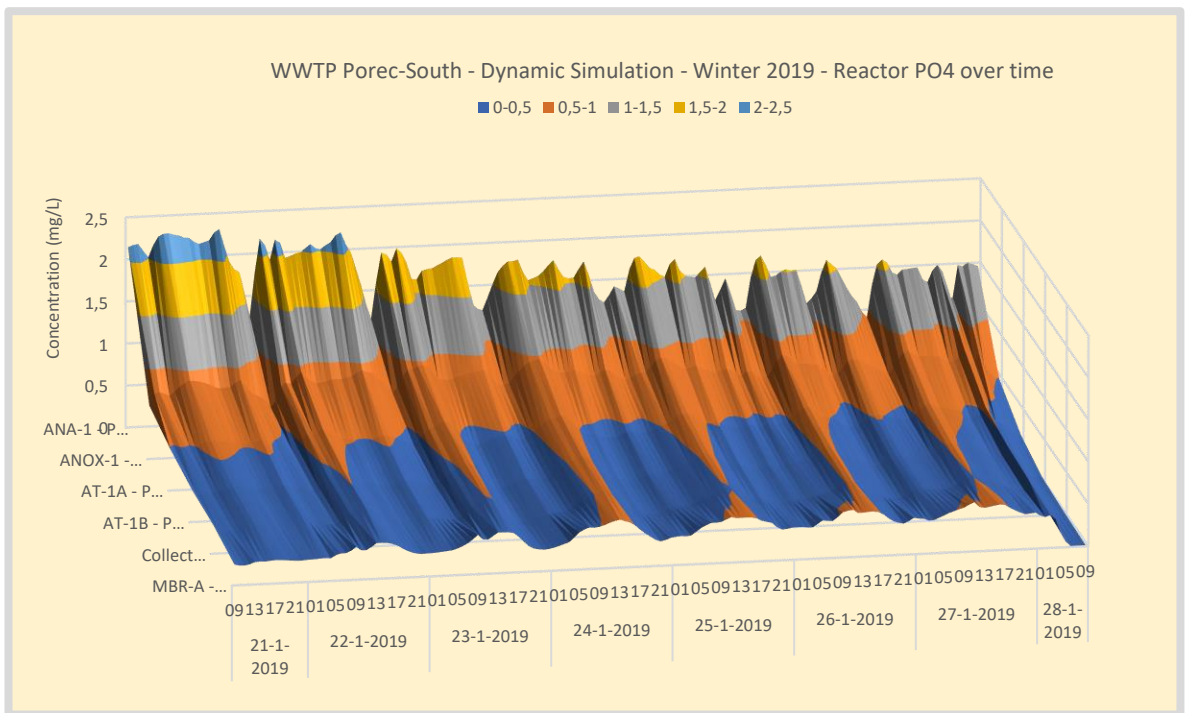
Figure 97. Winter – WWTP Poreč-South PO4 concentration profile over the waterline.
