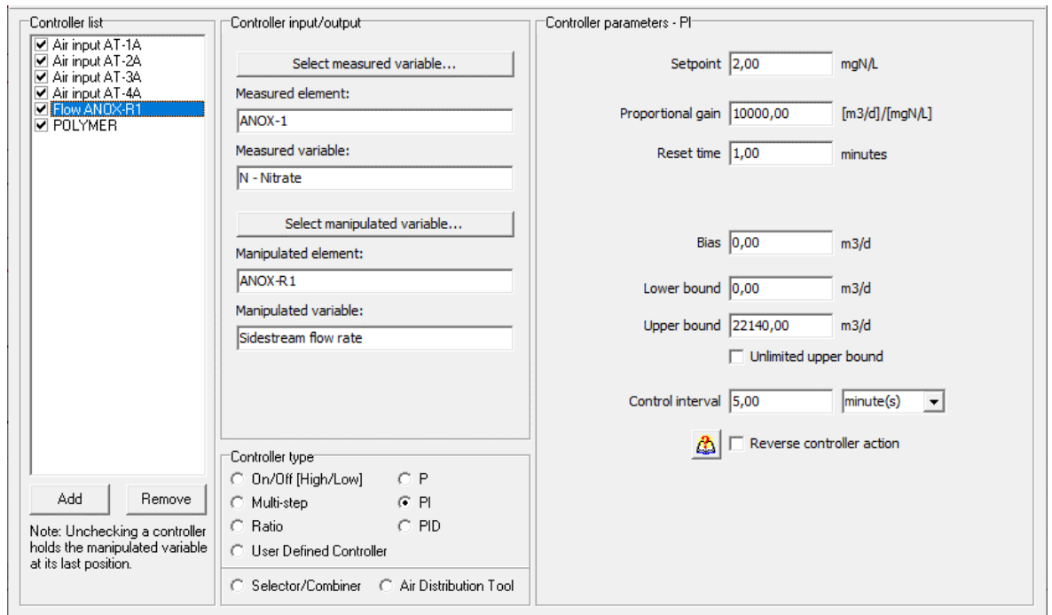
Figure 114. Summer – WWTP Poreč-South BioWin controller toolbox used for controlling the anoxic recycle ANOX-R. Indicated are the measured variable being NO 3 in the anoxic tank and manipulated variable the recycle flow ANOX-R. The PI controller has an upper bound of 22140 m 3 /d equal to the maximum installed pump capacity.
