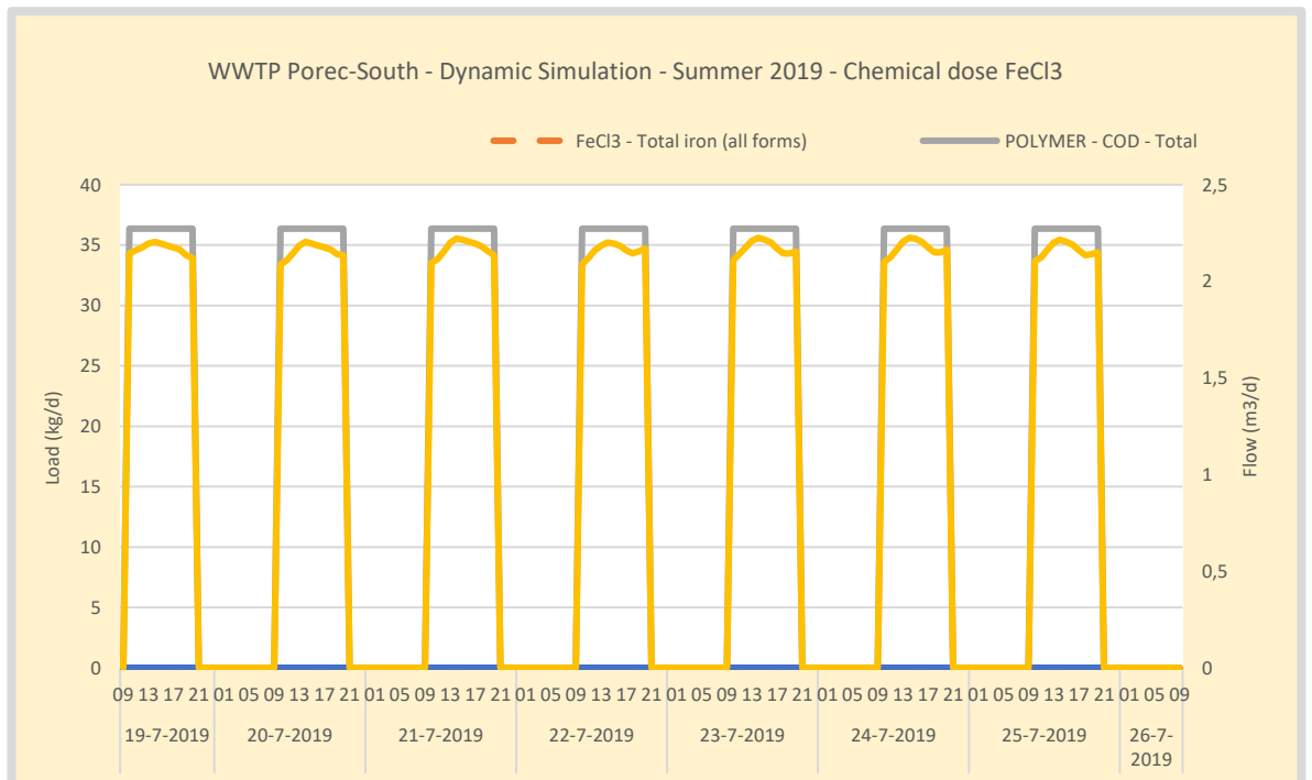
Figure 131. Summer – WWTP Poreč-South load and flow of Iron and PE. No iron is dosed. PE is assumed particulate biodegradable COD with a COD/VSS ratio of 1,42 gCOD/gTSS and dosed proportional to the WAS load based on 8 kg PE (dry weight) dosed per 1000 kg WAS (dry weight) flowing in the dewatering.
