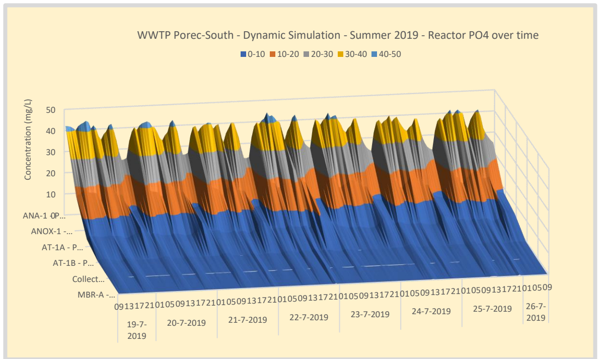
Figure 126. Summer – WWTP Poreč-South PO4 concentration profile over the waterline.
