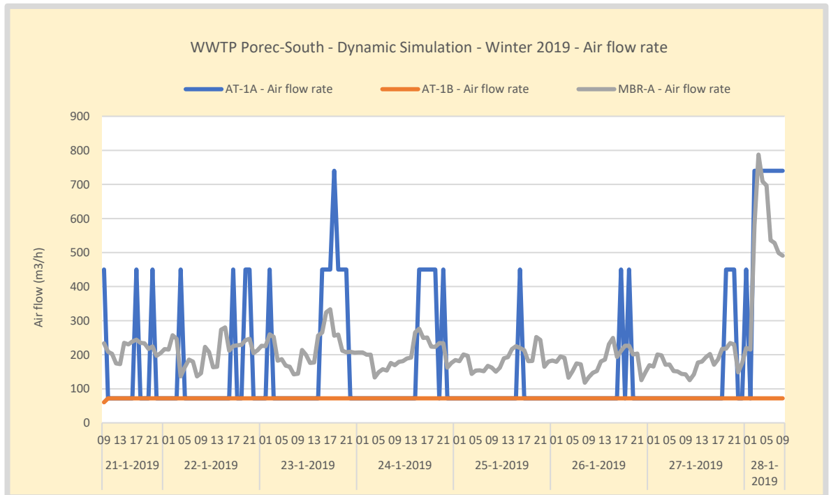
Figure 98. Winter – WWTP Poreč-South air input in the different aerated reactors. AT-A is step controlled on \text{NH}_4 , AT-B is setpoint controlled on the DO, the MBR is DO controlled on 6 \text{ mgO}_2/\text{L} reducing stripping of alkalinity.
