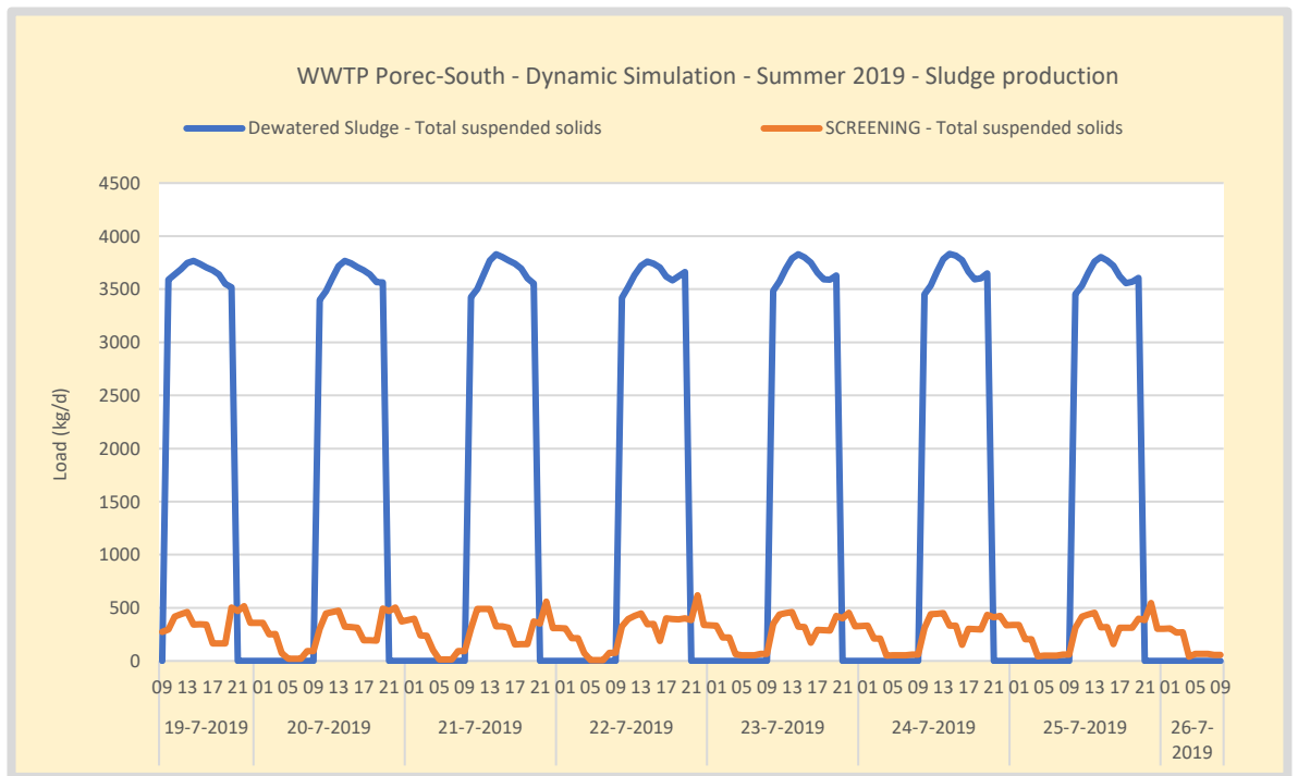
Figure 136. Summer – WWTP Poreč-South dewatered sludge load and compacted screening load. Dewatered sludge is operated 10 hours a day at 23%. Screening is produces continuously as a factor of the influent.
