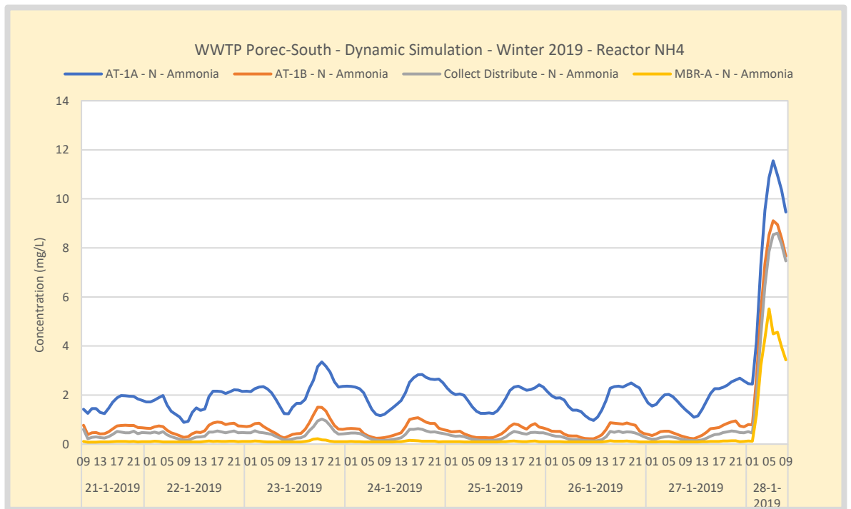
Figure 92. Winter – WWTP Poreč-South ammonium profile in the waterline. The air input of AT-A is controlled based on \text{NH}_4 measured in the collect distribute tank using a 3-step controller. Above 1,0 \text{ mgNH}_4/\text{L} the air input goes to its maximum value. Below 0,5 air shuts off. AT-B is DO controlled on 2,0 \text{ mgO}_2/\text{L} .
