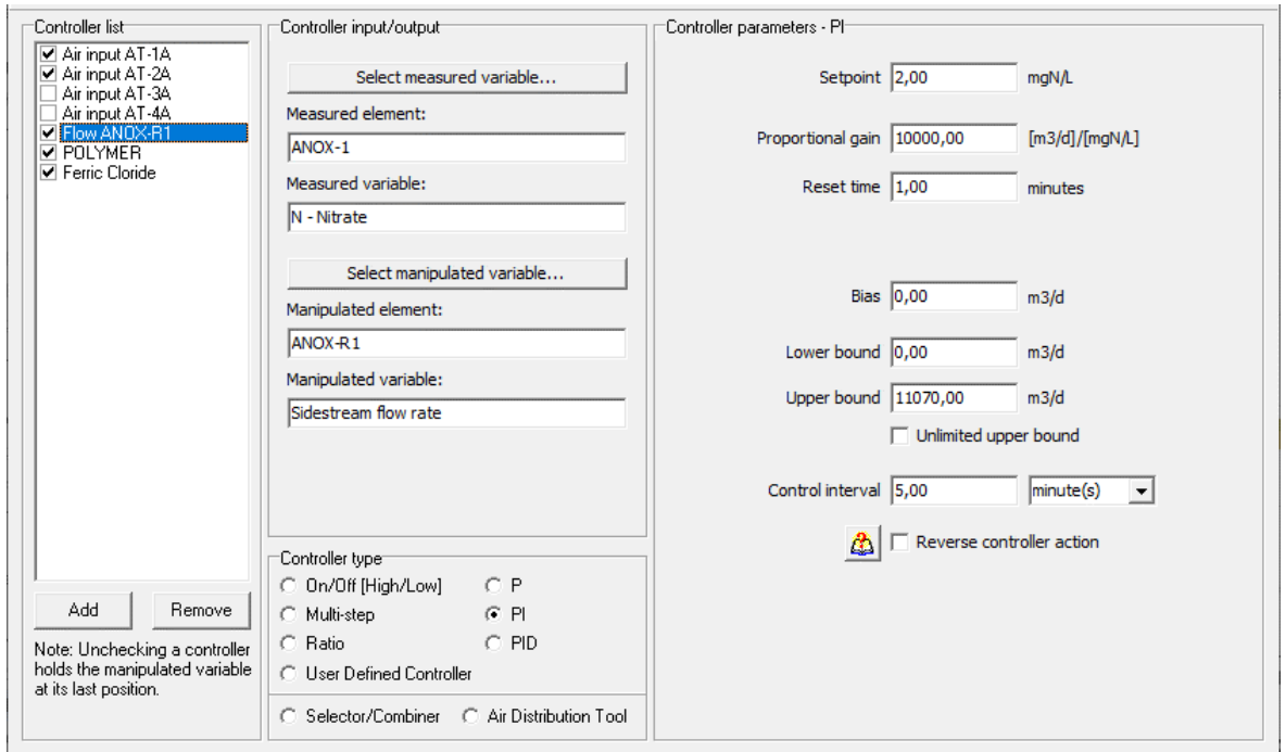
Figure 84. Winter – WWTP Poreč-South BioWin controller toolbox used for controlling the anoxic recycle ANOX-R. Indicated are the measured variable being NO 3 in the anoxic tank and manipulated variable the recycle flow ANOX-R. The PI controller has an upper bound of 11.070 m 3 /d according to the maximum installed pump capacity per lane.
