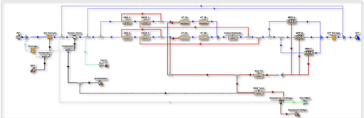
Figure 110. WWTP Poreč-South - BioWin model summer operation. All lines are in operation. Dashed lines are not operated. Operational adjustments are made to accommodate dynamic modelling under summer conditions.
