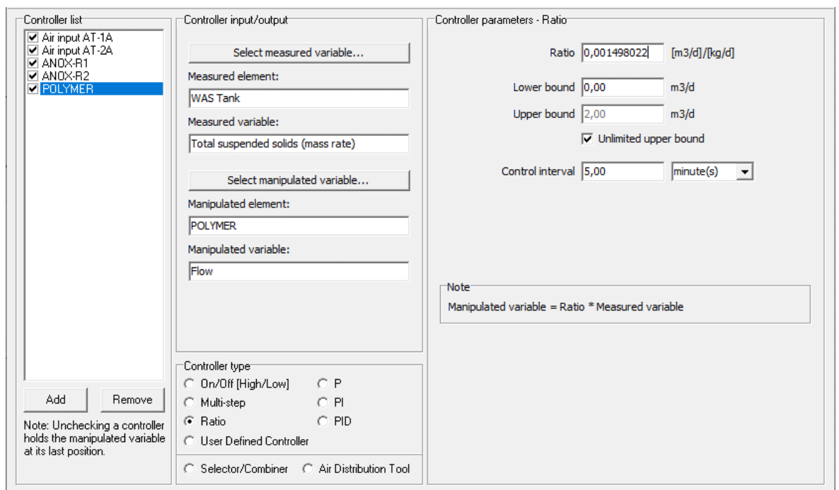
Figure 115. Summer – WWTP Poreč-South BioWin controller toolbox used for controlling the polymer dosage of the dewatering. Indicated are the measured variable being the TSS load entering the dewatering and manipulated variable the PE flow. The applied control ratio is 8 kg PE per 1000 kg TSS based on dry weight. PE is assumed to be particulate substrate with a COD/VSS ratio of 1,42.
