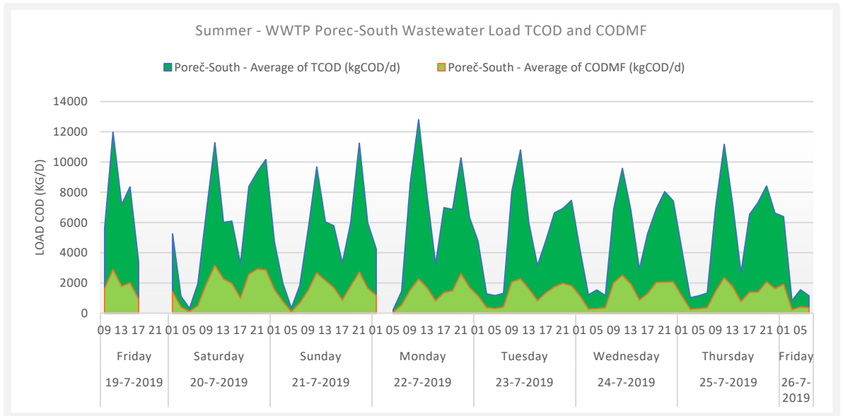
Figure 54. Summer - WWTP Poreč-South Wastewater Load TCOD and CODMF. No rain events occurred during the measurement period. For the model input missing data points are reconstructed based on the hourly average dry weather load.
