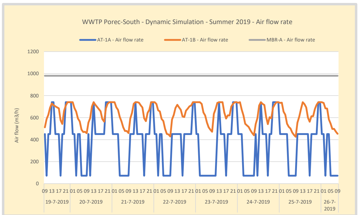
Figure 127. Summer – WWTP Poreč-South air input in the different aerated reactors. AT-A is step controlled on NH4, AT-B is setpoint controlled on the DO, the MBR is fully aerated according to the design value.
