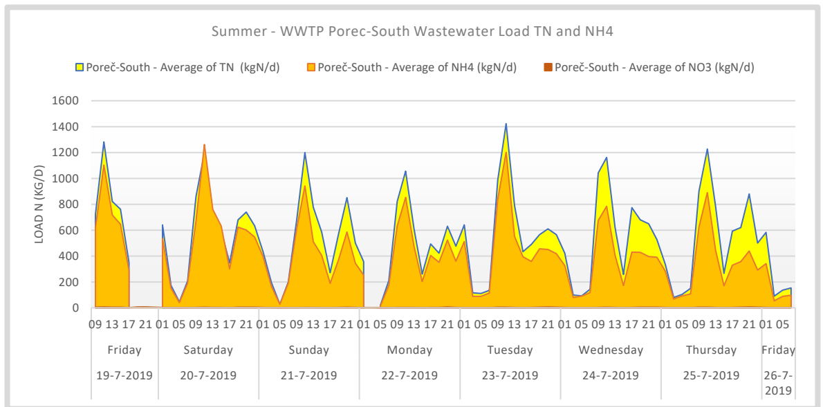
Figure 62. Summer - WWTP Poreč-South Wastewater Load TN, NH4 and NO3. No rain events occurred during the measurement period. For the model input missing data points (19 and 22-7) are reconstructed based on the hourly average dry weather load.
