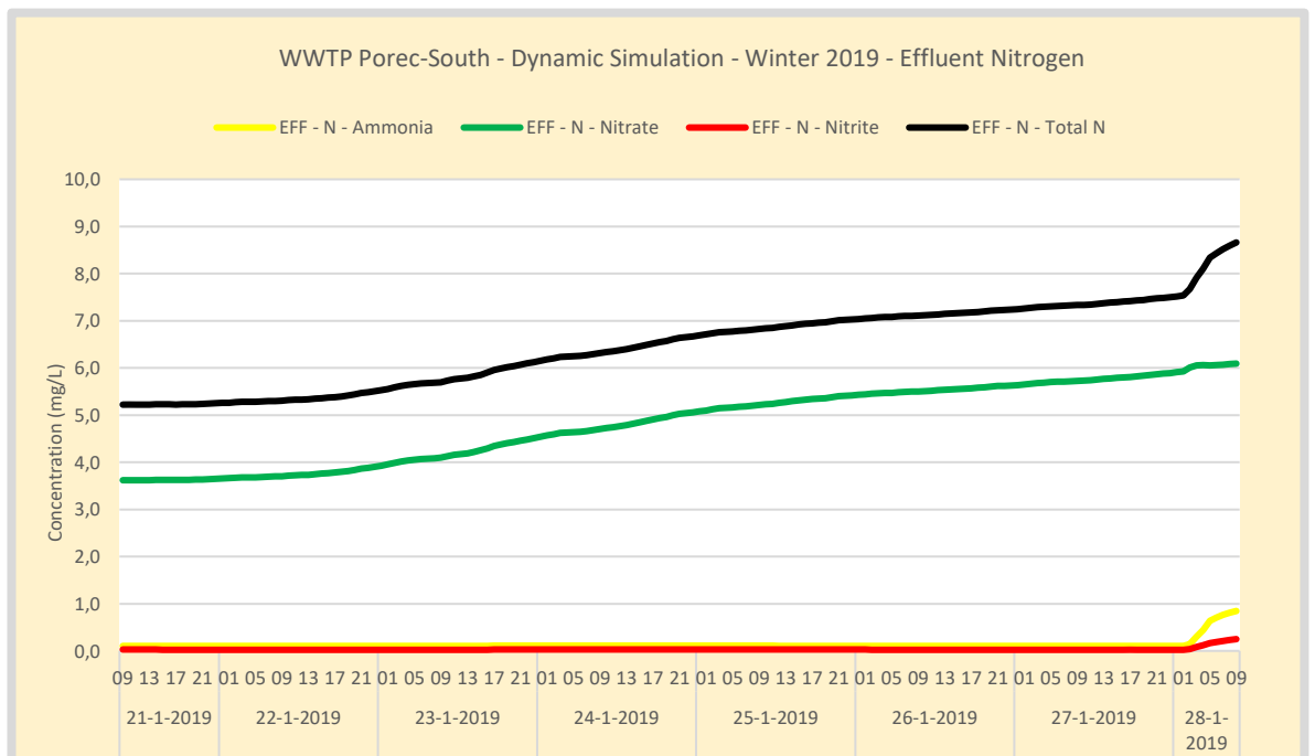
Figure 107. Winter – WWTP Poreč-South Effluent nitrogen concentration. Effluent is measured in the outflow of the large effluent buffer.
